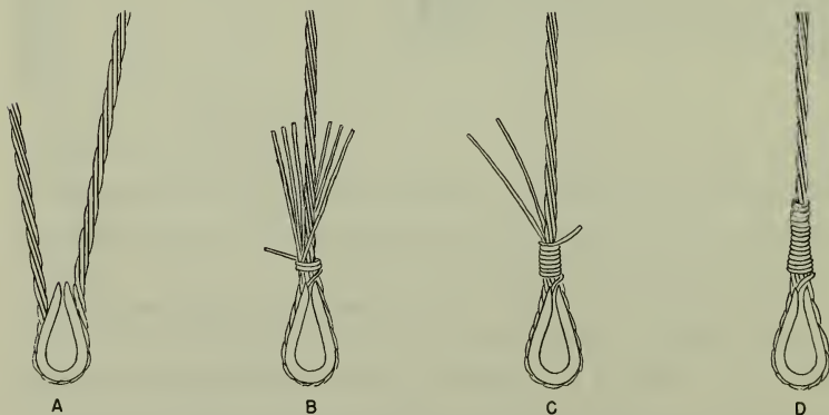
Figure 18.—Steps in making an eye splice in 7-wire strand.
