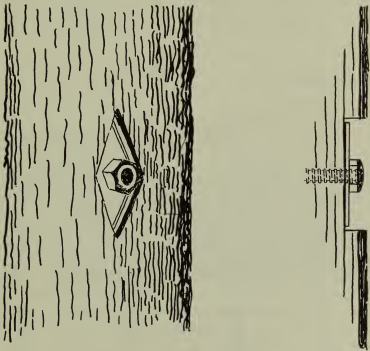
Figure 17.—Countersink.
