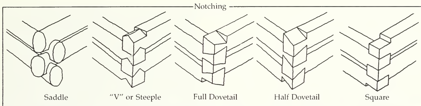
Fig. 10. Five examples of the more common historical methods of corner notching. Drawing: James Caufield.
