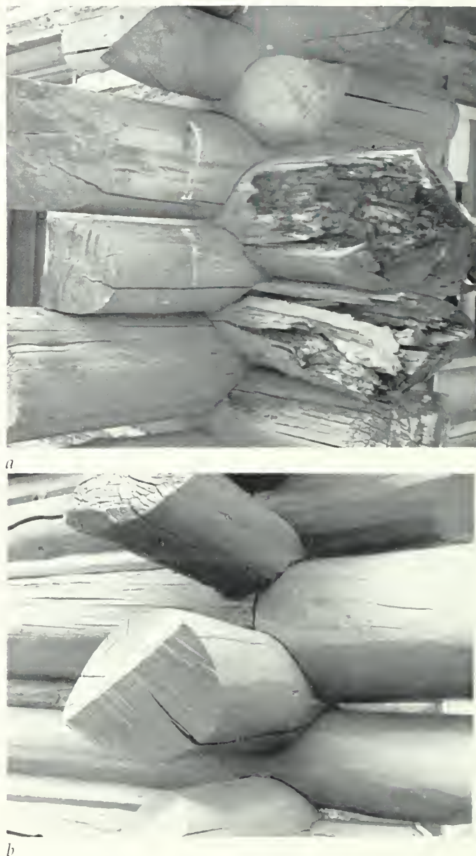
Fig. 20. (a) These deteriorated log crowns were (b) repaired with new crowns which were attached to the historic logs with reinforcing bars and epoxy. Epoxy repair of log crowns is most successful when the repaired crowns are protected from excess moisture by a roof overhang. Photos: Harrison Goodall.
