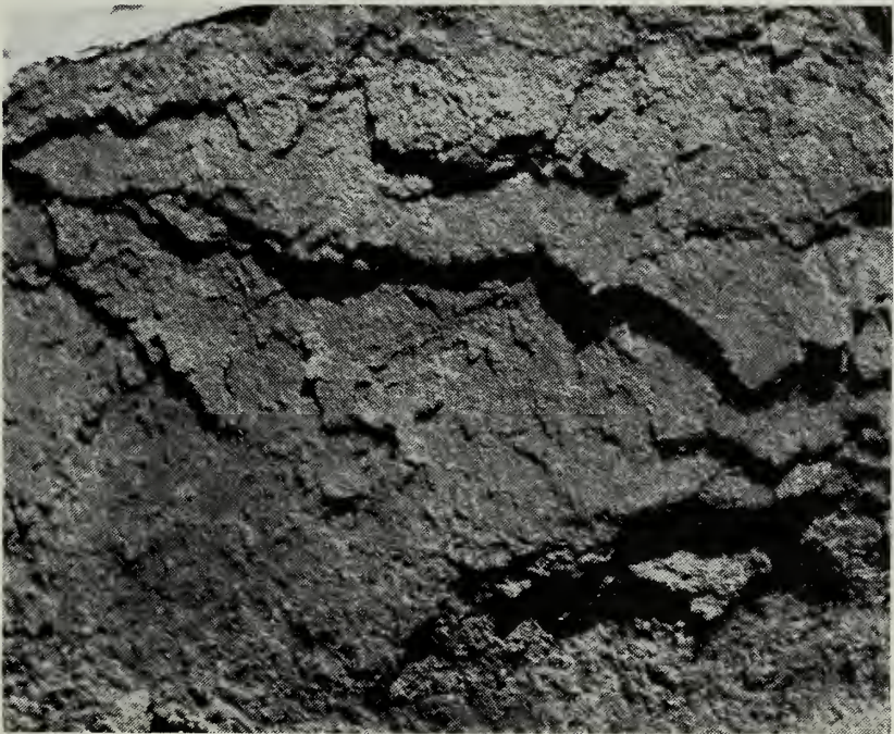
Exfoliation of sandstone. Photograph: Anne E. Grimmer.
