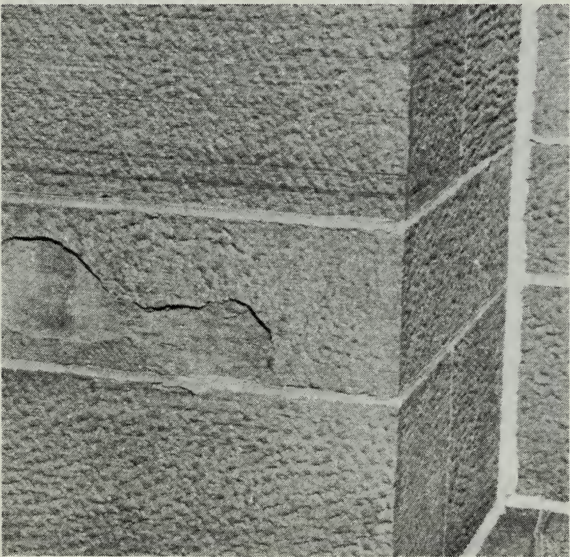
Blistering of sandstone. Photograph: Anne E. Grimmer.
