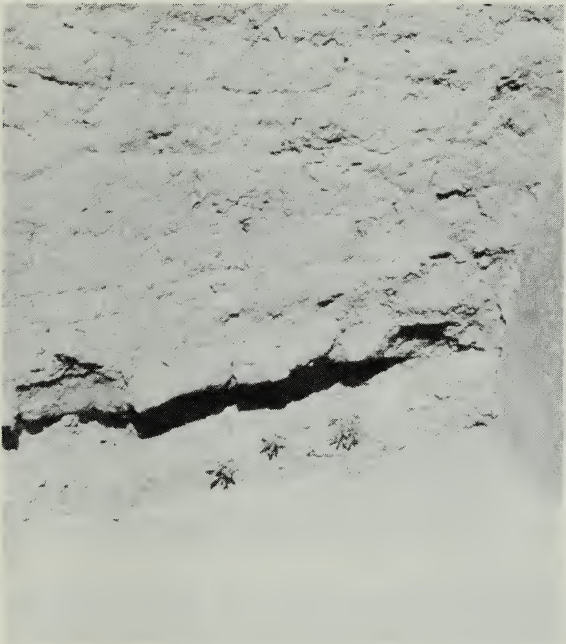
Coving of adobe wall. Photograph: National Park Service.
