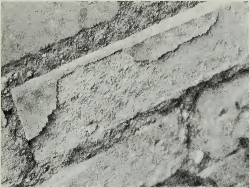
Spalling of brick. Photograph: Susan Dynes.
