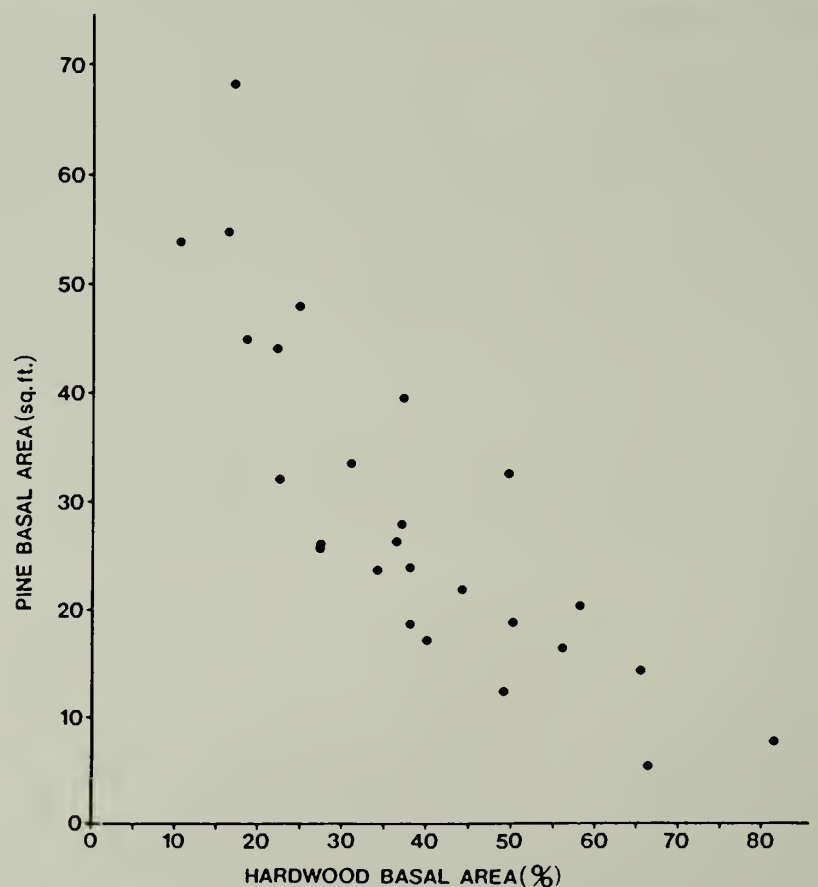
Figure 2. Pine basal area per acre to percent hardwood basal area comparison at Floyd County (age 11).
