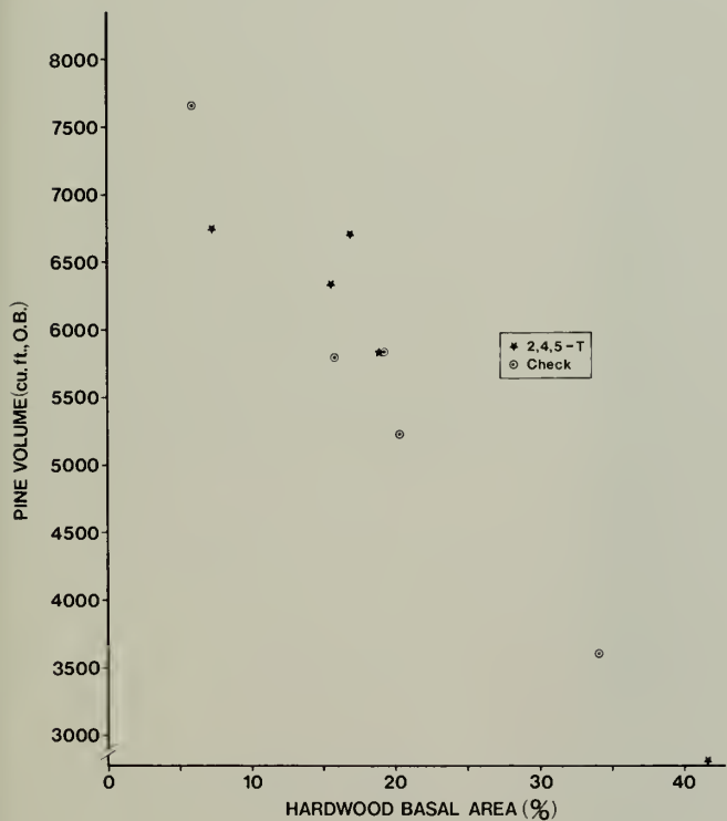
Figure 4. Pine cubic foot volume per acre to percent hardwood basal area comparison at Summerville-6 (age 30).
