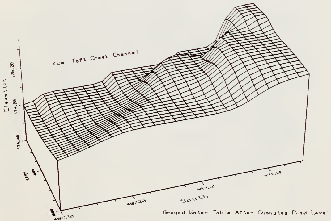
FIGURE 4. THREE DIMENSIONAL PLOT DEPICTING THE GROUND WATER TABLE BEFORE AND AFTER CHANGING THE POND LEVEL
