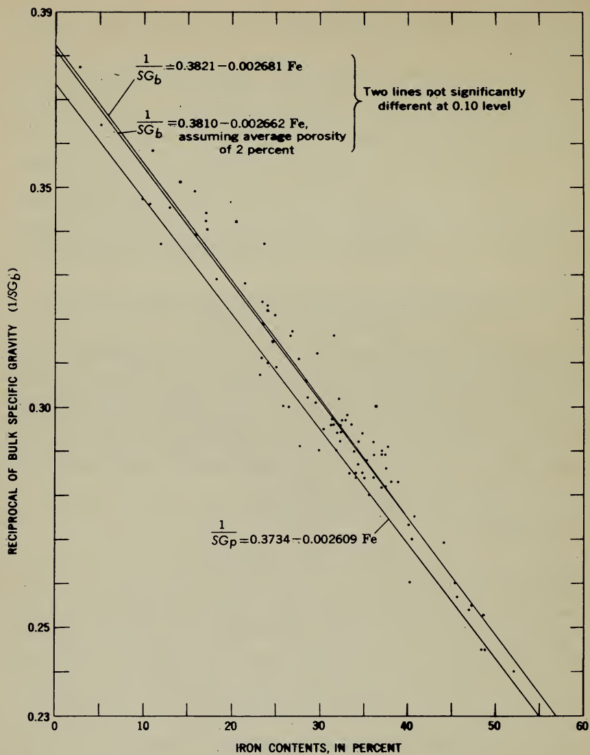
FIGURE 3.—Correlation between the reciprocal of the bulk specific gravity and the iron content. The line of equation 1/SG_p = 0.3734 - 0.002609 \text{ Fe} from figure 2.
