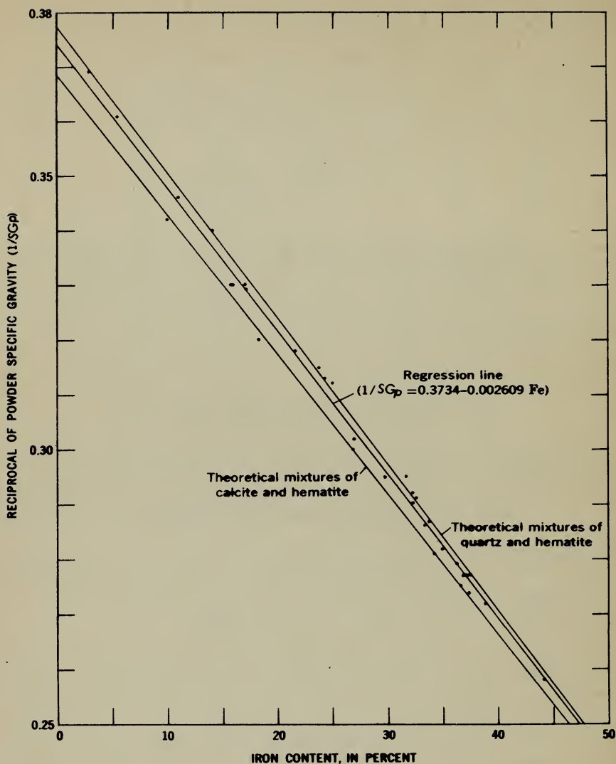
FIGURE 2.—Correlation between the reciprocal of the powder specific gravity and the iron content.
