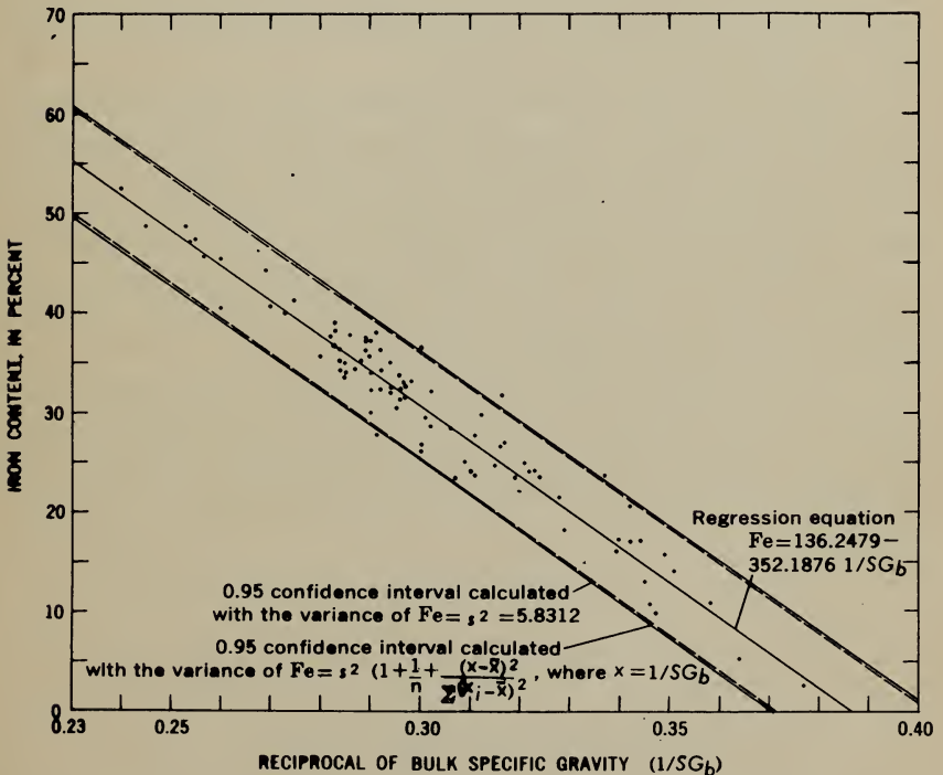
FIGURE 4.—Quality-control chart for selection of iron ore from the reciprocal of bulk specific gravity.
