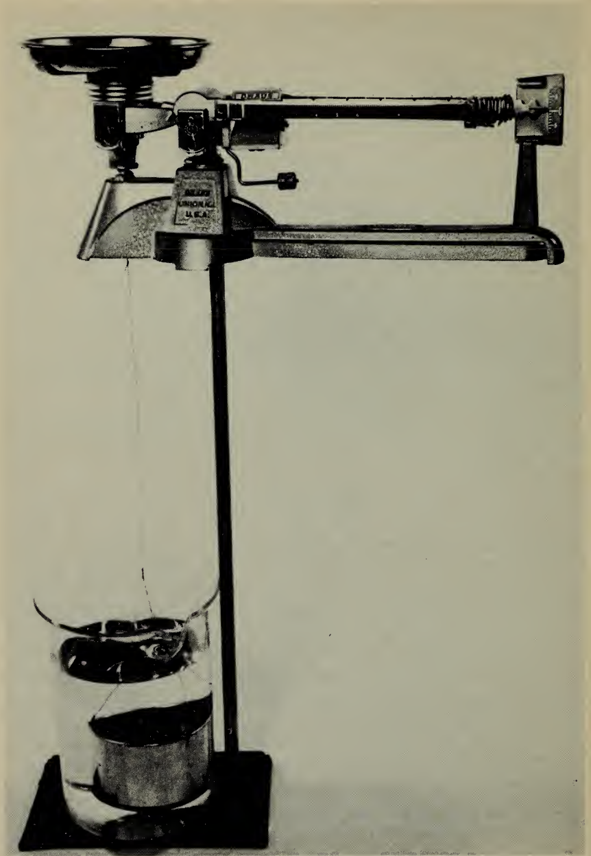
FIGURE 1.—Specific-gravity balance. Apparatus is 26 inches high.
