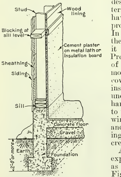
FIGURE 7.—Recommended construction of walls and floors of new frame barns. Cement plaster on metal lath or insulating board is applied to the inside of the studs at least to the level of the window sills as a better protection against rats and as being more easily kept clean than wooden lining
