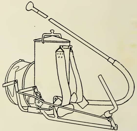
FIGURE 7.—Knapsack-bellows duster.
