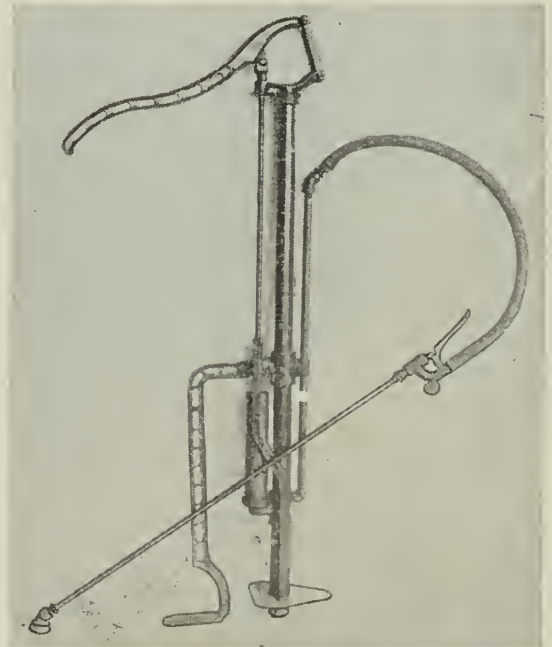
FIGURE 4.—Bucket pump with hose, extension rod, cut-off, and nozzle.
