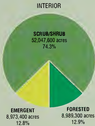
Figures 12, 13, 14 Palustrine Vegetated Wetlands by Region
