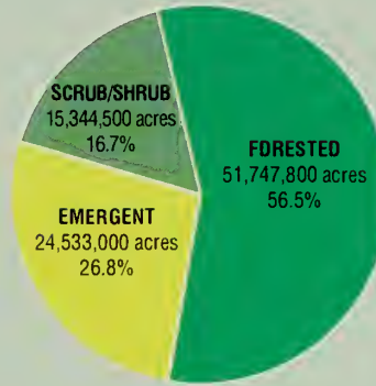
Figure 11 Palustrine Vegetated Wetlands in the Lower 48 States
