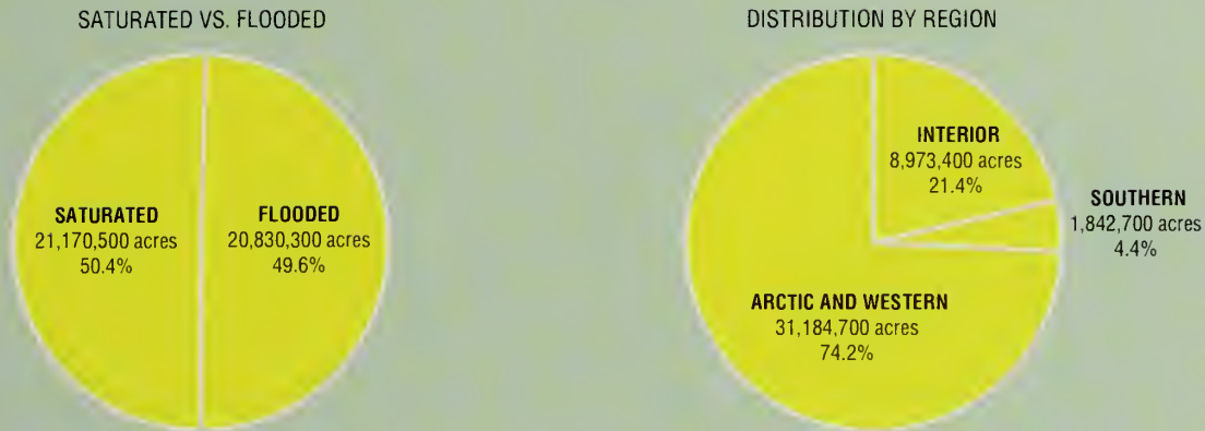
Figures 15, 16 Palustrine Emergent Wetlands
