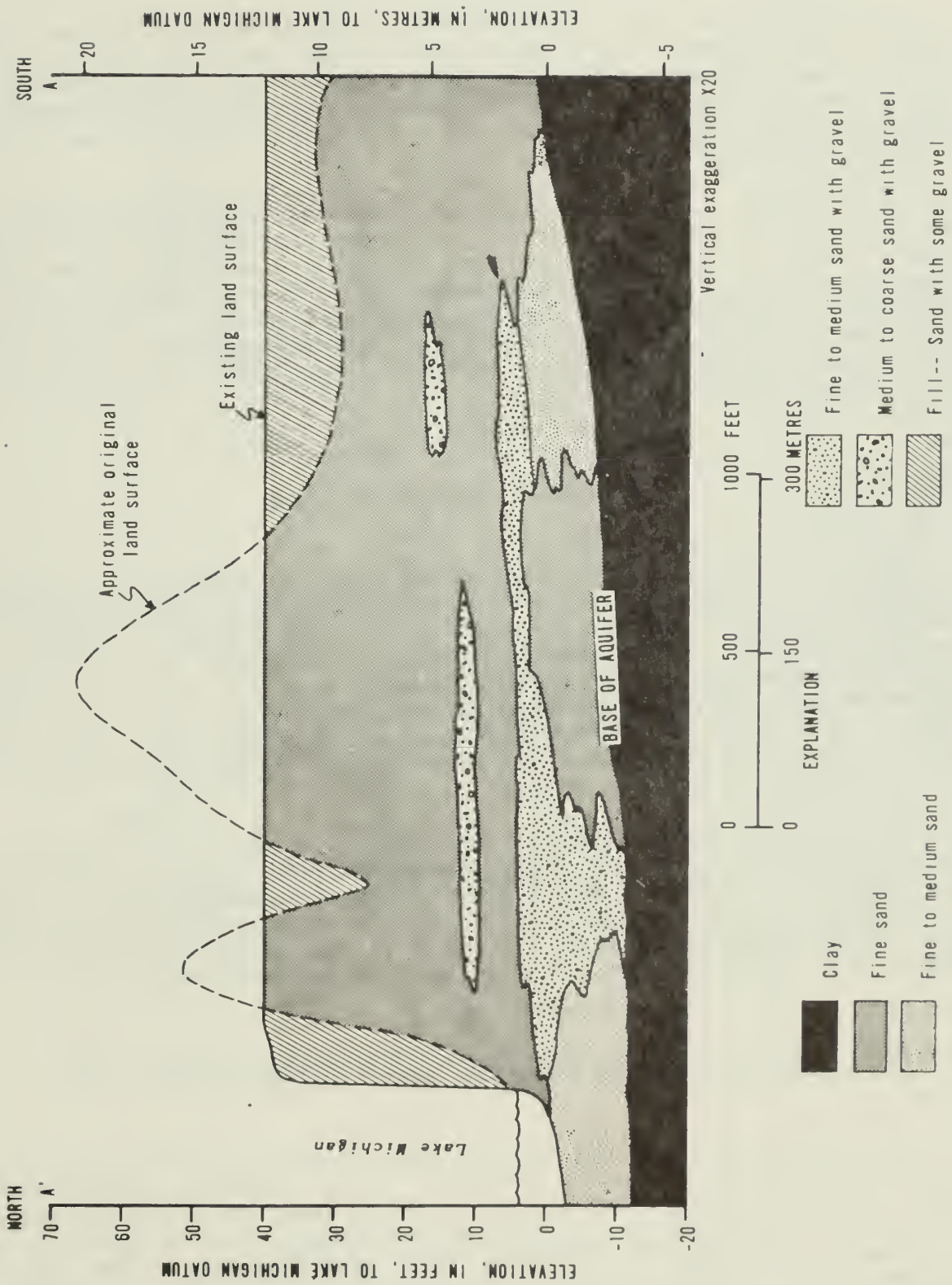
Figure 3.-- Idealized geologic section of the construction site.
