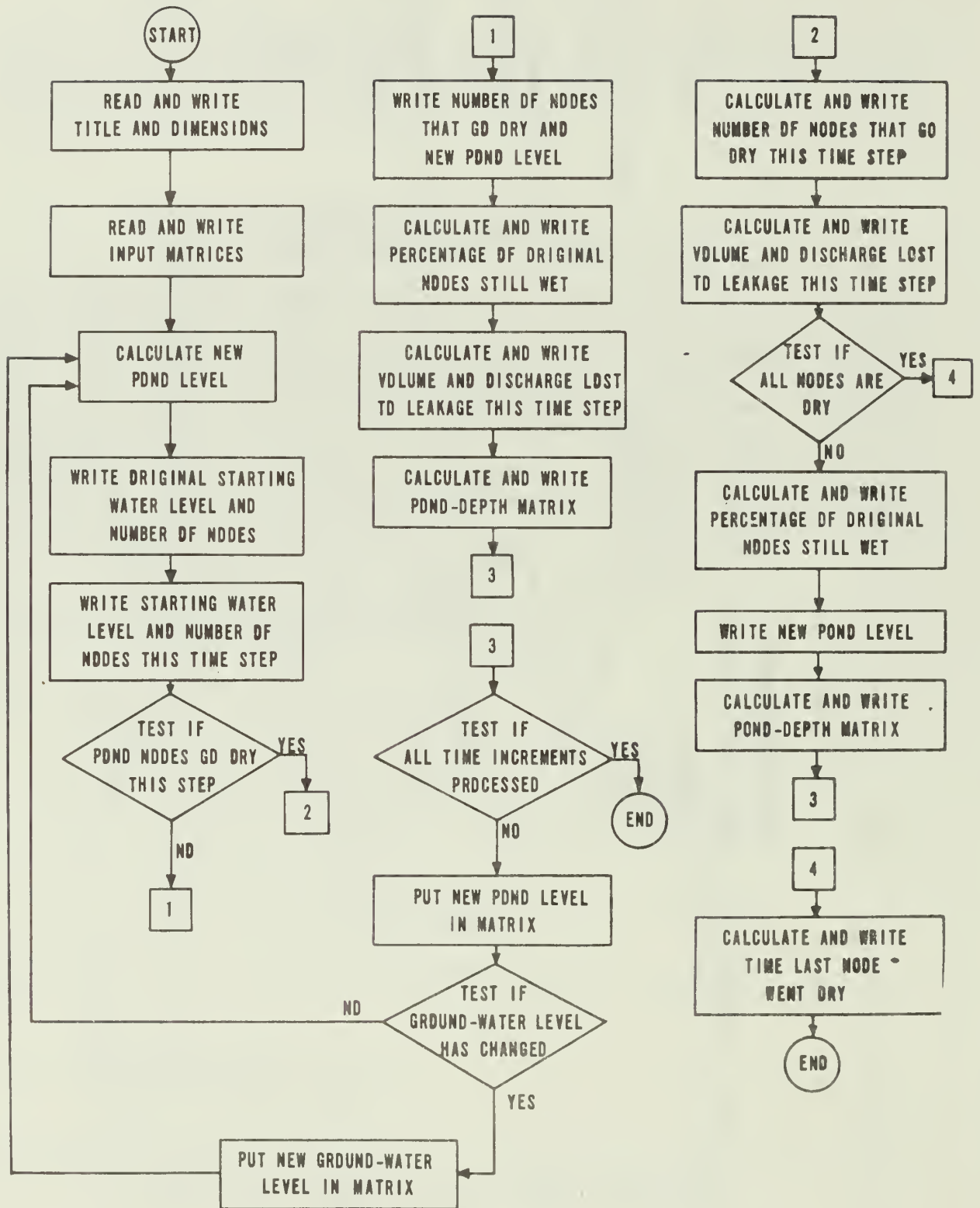
Figure 8. -- Flow chart for pond model.
