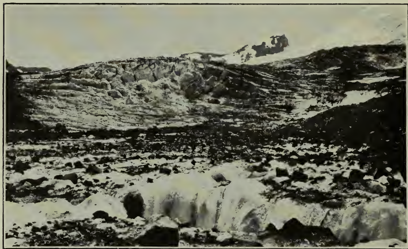
FIG. 14.—A CREVASSÉD DOME ON THE LOWER WINTHROP GLACIER.
