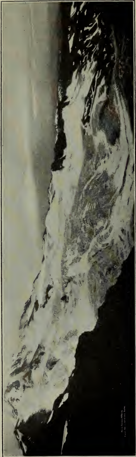
FIG. 20.—THE NORTH MOWICH GLACIER AND THE ICE FIELDS TO THE SOUTH OF IT. Copyrighted photo by Curtis.
