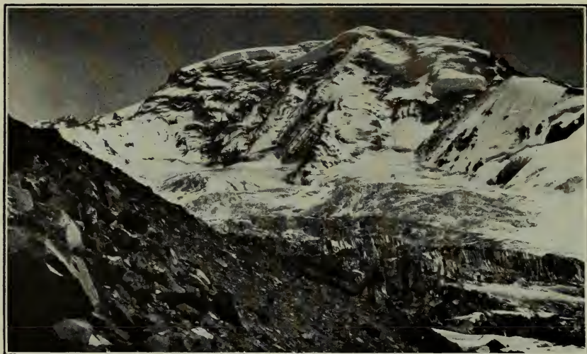
FIG. 15.—THE GREAT AMPHITHEATER OF CARBON GLACIER. THE HEADWALL MEASURES 3,600 FEET IN HEIGHT. GREAT AVALANCHES FALL PERIODICALLY FROM THE SNOW CLIFFS ABOVE, WHICH THEMSELVES ARE 200 TO 300 FEET HIGH.
