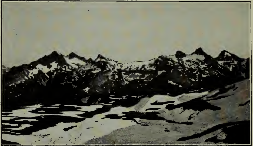
FIG. 3.—THE TATOOSII RANGE, FROM PARADISE GLACIER.
