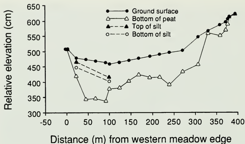
Fig. 27. Thickness of peat along transect 1. A buried mineral horizon occurs within the peat body on the western side of Big Meadows.
