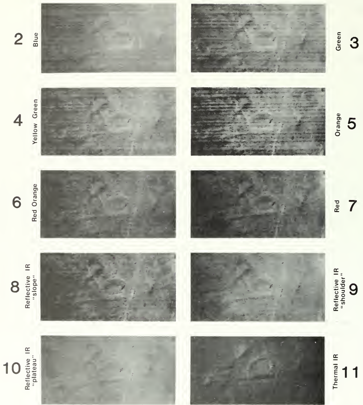
Figure 4 Typical M'S digital-to-image output for an area around Pueblo Alto. Slight differences in gray scale are due to gain and brightness adjustments during video display. Due to photo trimming, each image as shown here contains approximately 235 scan lines and 425 samples; an area on the ground equivalent to 880 feet by 1595 feet (1" = 587 feet). The words "slope", "shoulder", and "plateau" refer to the typical reflected IR curve for vigorous vegetation.
