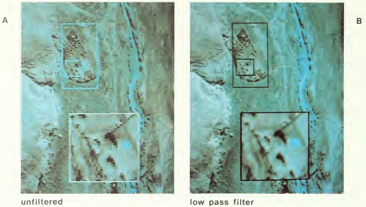
Figure 13 Example of data filtering. The blocky appearance of the enlarged portion of A results from enlarging the pixel size 4-times. Within this area there are several kivas which are lost, for the most part, to visual recognition because of the blockiness. By performing a \frac{\sin X}{X} transformation of pixel values, the blockiness can be "smoothed," as in B, to permit easier pattern recognition. Although the filtered version appears to be somewhat out of focus, it is easier to discern the kiva structures.
