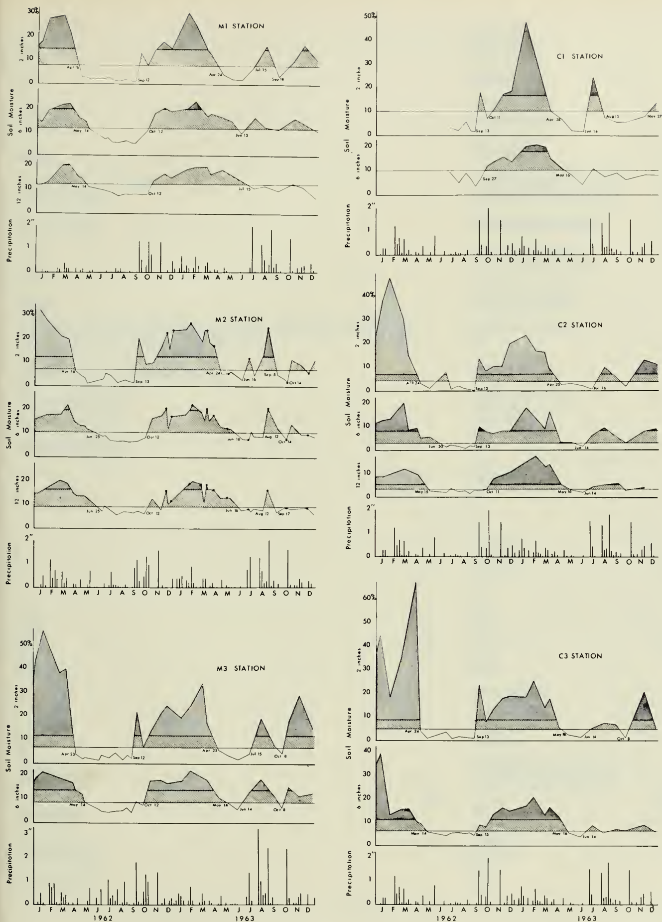
15 Graph showing soil moisture content and precipitation at the six sites in 1962 and 1963. The light hatching indicates available moisture, while the darker shading represents moisture content above field capacity. A continuous horizontal line marks the permanent wilting coefficient for each depth. Precipitation is shown in the bar graphs. At M-2, four replicated gravimetric samples were collected each month during 1963; their average moisture content is indicated by dots.
