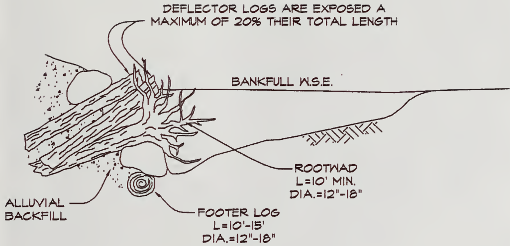
LOG, ROOTWAD, AND BOULDER REVETMENT DETAIL (D) TYPICAL CROSS-SECTION 5 N.T.S
