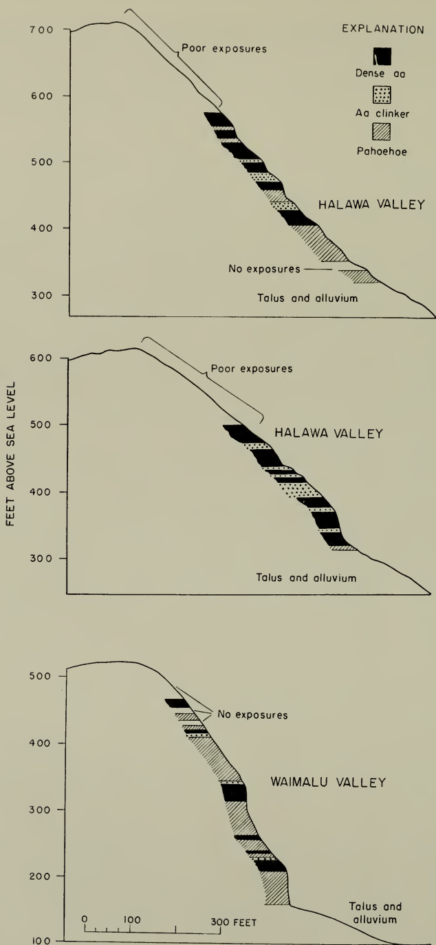
FIGURE 3.—Sections showing proportions of lava-flow types exposed in the walls of Halawa and Waimalu valleys, Oahu.
