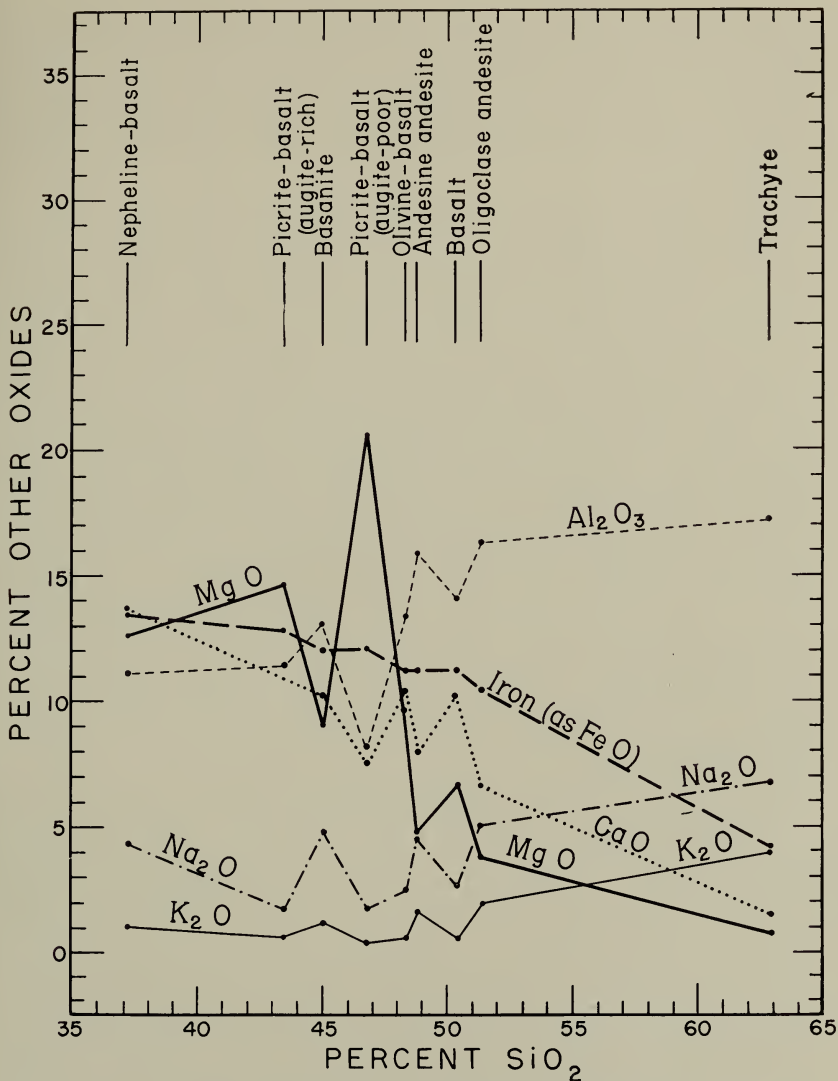
FIGURE 1.—Diagram showing composition of Hawaiian lavas.
