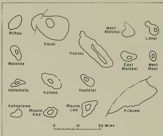
FIGURE 2.—Outlines of Hawaiian shields. The inner contour for each is 1,000 feet below supposed original summit; the second is 3,000 feet below.
