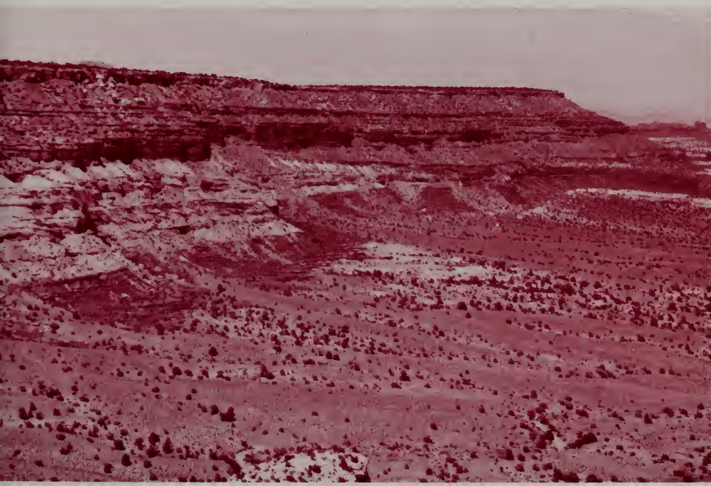
WHITE RIM SANDSTONE in north wall of Range Canyon, south of Elaterite Basin. Bed thins from 230 feet at left (west) to 38 feet at right (east), and disappears (by facies change into red shales) a short distance farther east. See description in text of pinch out of Hoskinnini Tongue. Bed at top of mesa is Moss Back Member of Chinle Formation. Photograph by Donald L. Baars. (Fig. 35)
