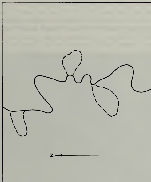
RELATIVELY RECENT RINCONS ALONG INDIAN CREEK, about 3\frac{1}{2} miles above mouth and about 2 miles east of Canyonlands National Park. Above, stereoscopic pair of aerial photographs by U.S. Geological Survey; below, sketch showing drainage changes. The stereoscopic pair can be viewed without optical aids by those accustomed to this procedure, or by use of a simple double-lens stereoscope. (Fig. 73)
