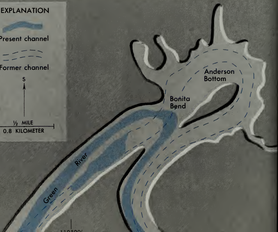
DRAINAGE CHANGES AT ANDERSON BOTTOM RINCON. River shortened itself about 2 miles by this cutoff. (Fig. 66)
