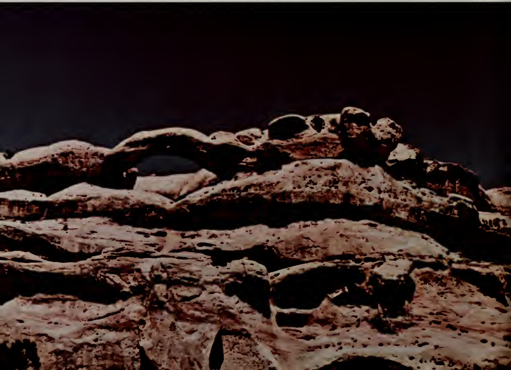
CATERPILLAR ARCH, in upper Lavender Canyon, looking northwest. Photograph by E. N. Hinrichs. (Fig. 48)
