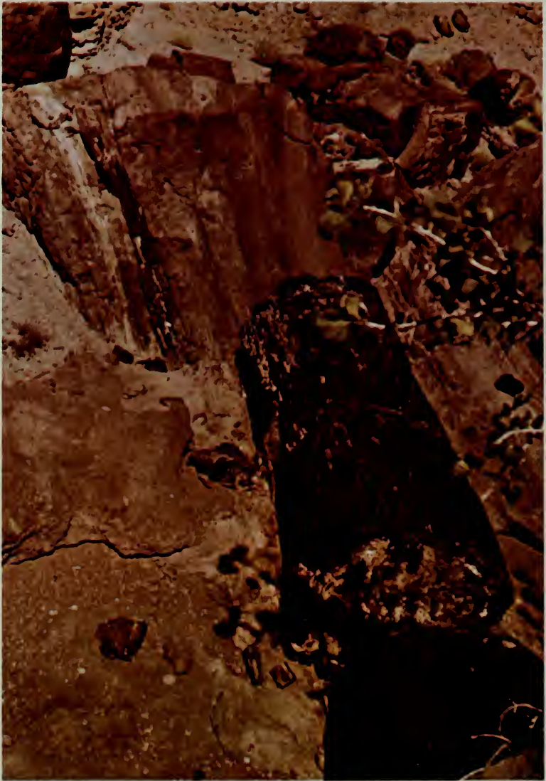
PETRIFIED LOG, near middle of Rico Formation, about 1 mile southeast of Dead Horse Point. Log is estimated to be about 18 inches in diameter. Photograph by Robert R. Norman. (Fig. 72)
