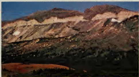
The peaks in this photograph (a view to the northwest from Marias Pass) are remnants of the overthrust block, which moved eastward. The dividing line between the light-colored rocks and the gray talus slopes beneath them is the Lewis Overthrust Fault.
