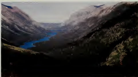
Glacial landforms can be identified in this view of the Mokowanis Valley.
