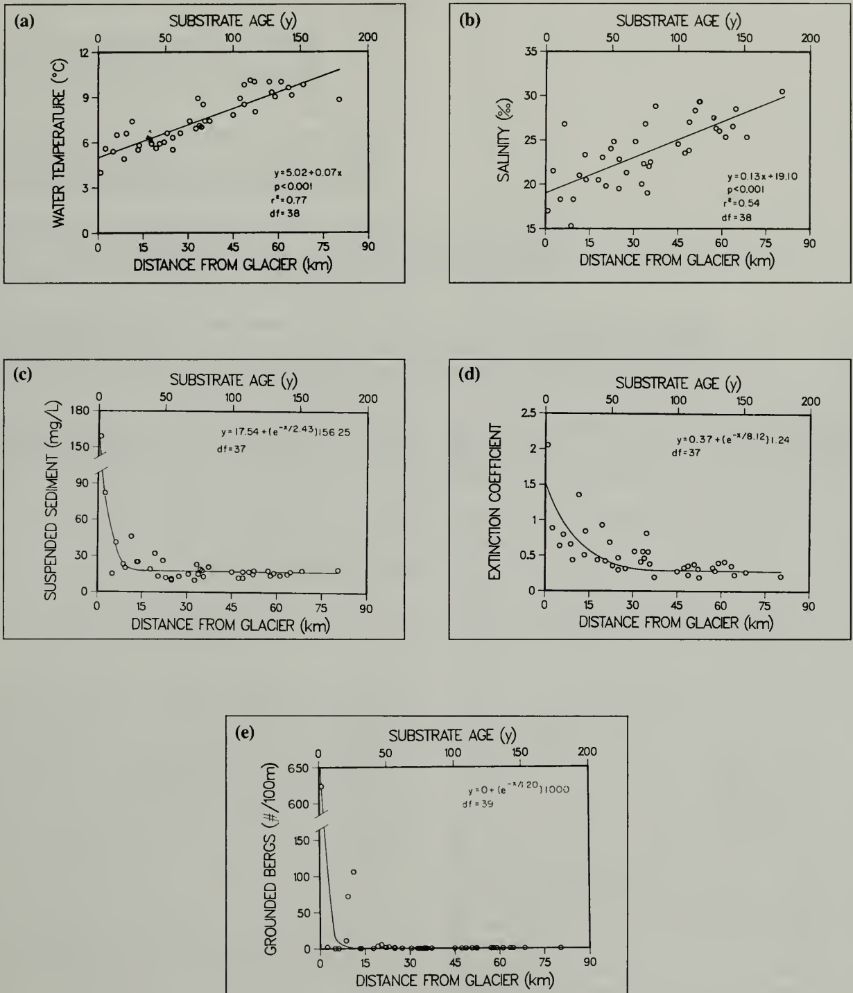
Fig. 3. Relationships to distance from Muir Glacier and substrate age shown by near-surface (a) water temperature, (b) salinity, (c) total suspended particulate concentration, (d) extinction coefficient, and (e) number of grounded ice fragments (= bergs). Values in (a), (b), and (c) are means of measurements made at depths of 0, 2.5, 5, and 7.5 m. N = 40 sites.
