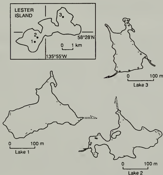
Fig. 1. Qualitative mini-piezometer readings of groundwater seepage for the three Lester Island lakes: "+" = groundwater seepage into the lake; "-" = seepage out of the lake; "0" = no seepage. Lake Three has the most shoreline with groundwater in-seepage, followed by Lake Two; Lake One has no groundwater input. Inlets and outlets are shown by either solid (perennial) or dotted (ephemeral) arrows.
