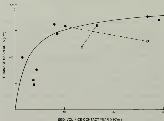
Fig. 3. Sediment volume in ice-proximal basins estimated from seismic profiles (from Molnia et al. 1984) averaged over the period of time Muir Glacier remained in or at the head of each basin, plotted against the successive areas of Muir Glacier's drainage basin (determined from Brown et al. 1982). The plot shows the relationship during recent retreat of the glacier.
