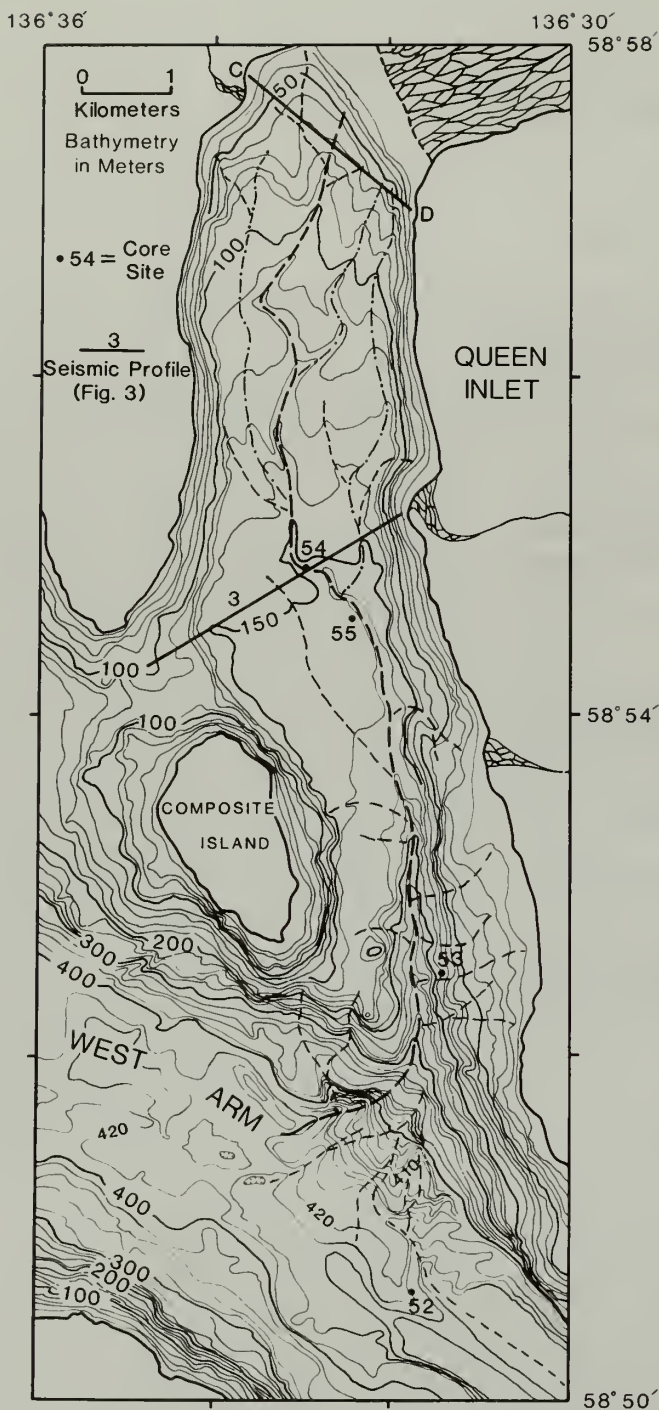
Fig. 1. Bathymetry of Queen Inlet, Glacier Bay, with channel thalwegs superimposed (main channel: thick dashed line; three smaller channels: thin dash-dot lines; smaller tributaries: thin dashed lines). Contour intervals: slopes, 20 m; fjord floor, 10 m; lobate fan area below Queen Inlet, 2 m. Datum is mean lower water. (Bathymetric soundings by U.S. National Oceanic and Atmospheric Administration, 1970). Numbered dots are sample locations. C-D is line of comparison profiles—NOAA, 1970 vs. USGS, 1984.
