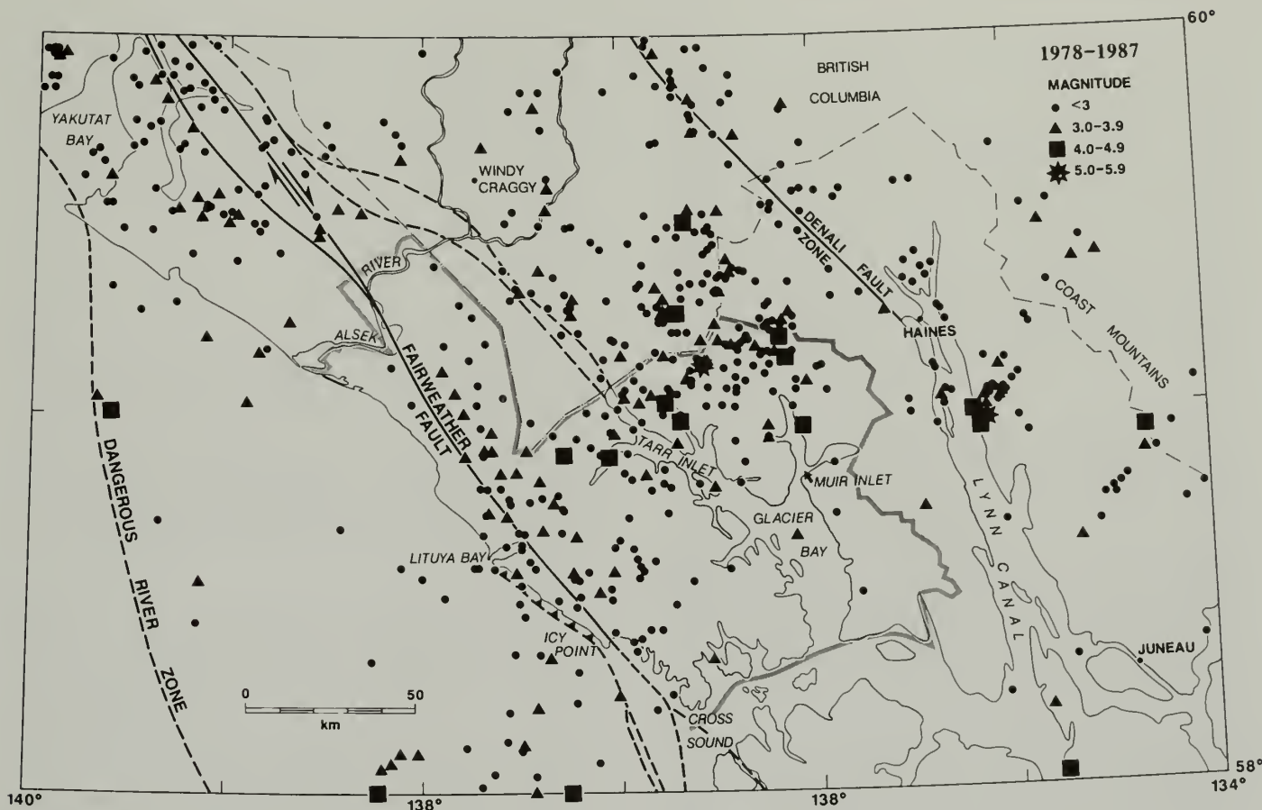
Fig. 3. Seismicity in the Glacier Bay region of southeastern Alaska and adjacent areas of British Columbia from 1978 to 1987. A temporary seismograph was installed at Windy Craggy, B.C., in June 1988.
