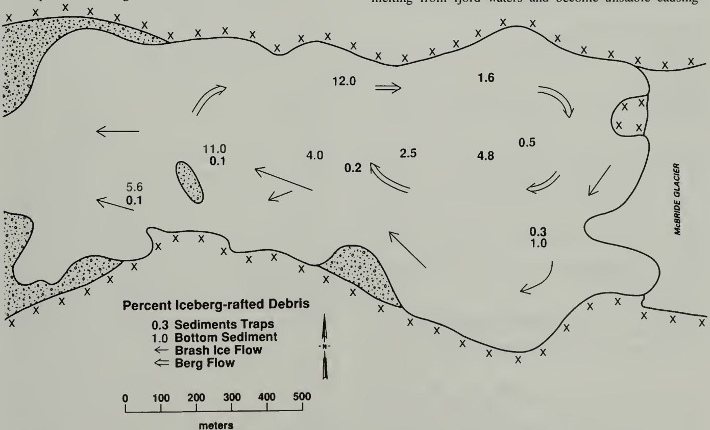
Fig. 2. Trajectories of calved ice within McBride Inlet (arrows). Berg movements are controlled by currents at 8 to 16 m depth, and brash ice is moved by surface currents and wind. Average concentrations of IBRD (numbers) are determined from sediment traps and bottom-sediment grabs.
