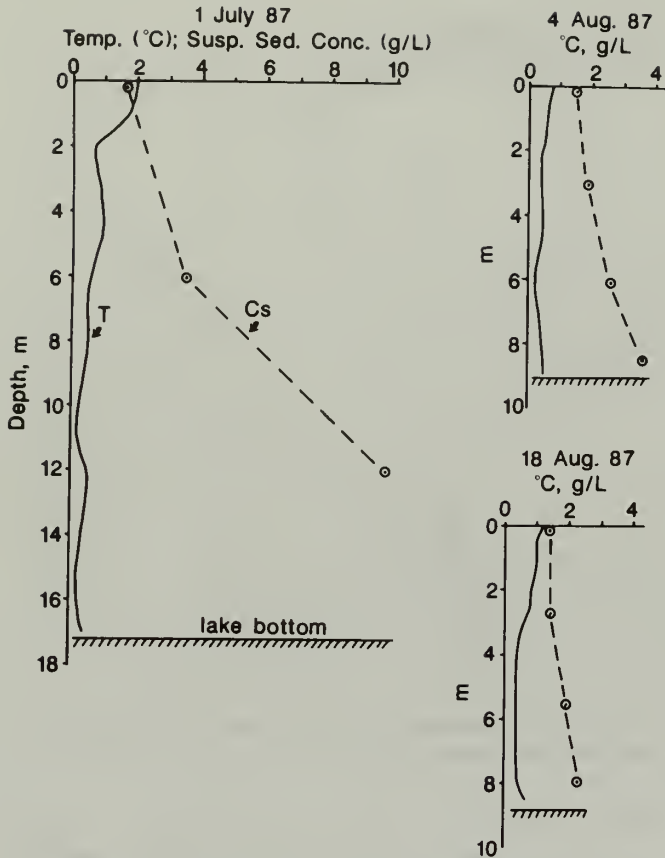
Fig. 3. Temperature profiles and suspended sediment concentrations at Loc. III (marked as "17.5 m" site in Fig. 2) on three successive dates. Note great decrease in depth between 1 July and 4 August, caused by rapid sedimentation associated with surge. Note also generally decreasing suspended sediment concentrations with time.
