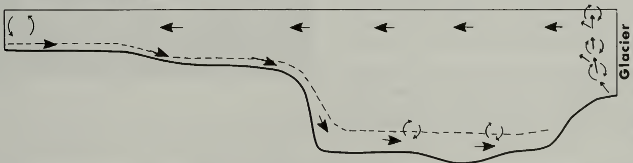
Fig. 4. Schematic diagram of flood tide circulation in McBride Inlet. Two types of circulation can occur, intermediate water renewal (A) during winter and spring and deep water renewal (B) during summer.
