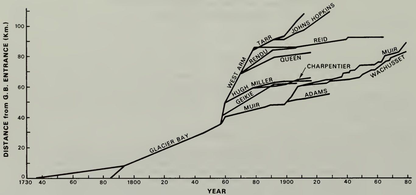
Fig. 1. Distance on a given year of tidewater fronts from the entrance of Glacier Bay. Slope of lines represents rate of retreat.
