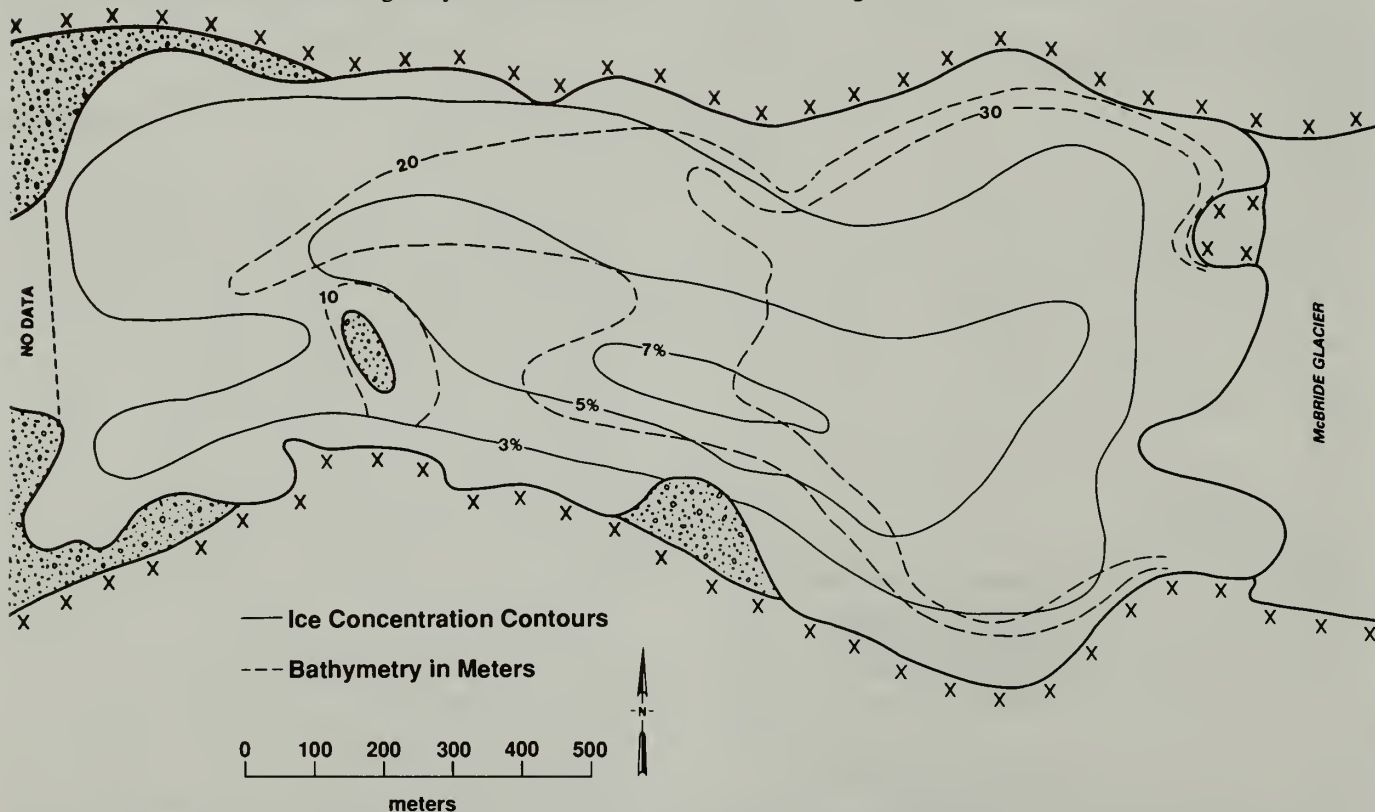
Fig. 3. Average proportions of water surface area covered by calved ice in McBride Inlet. Highest concentrations of ice occur where paths of bergs and brash ice overlap in the southwestern area of the ice-proximal basin. Depth contours show the sill where bergs ground during ebb tides on the west side of the ice-proximal basin.
