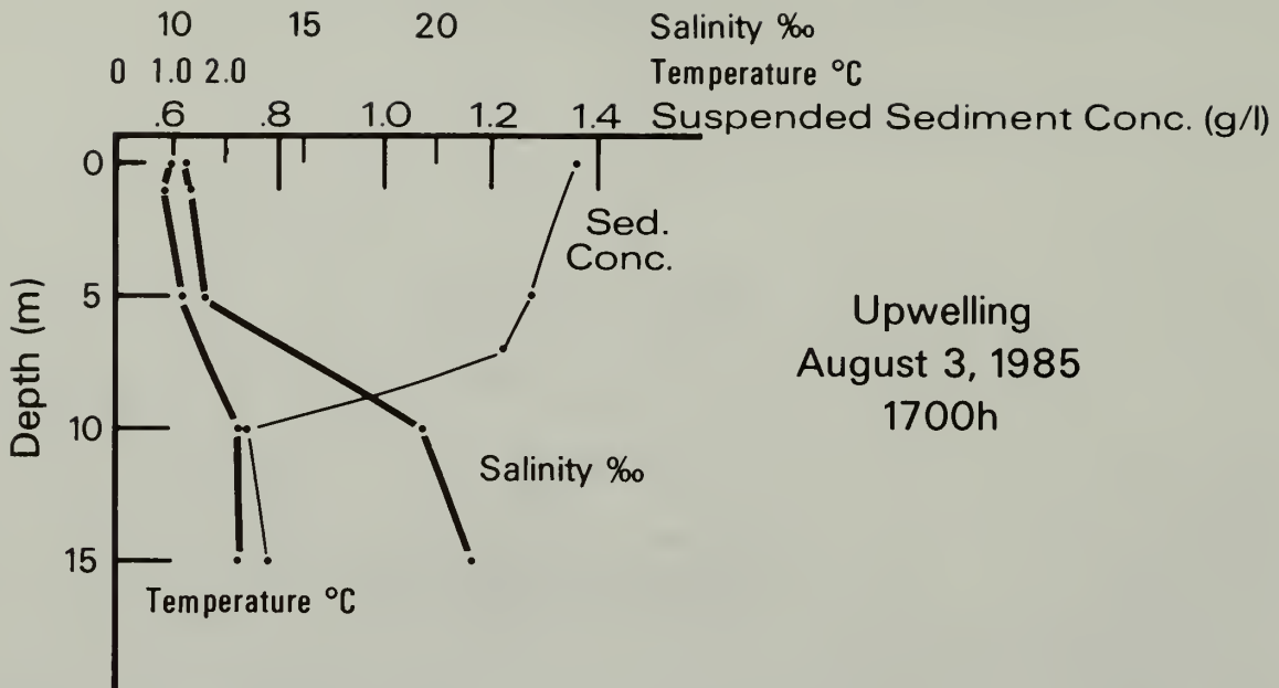
Fig. 2. Salinity, temperature and suspended sediment concentrations within the upwelling on August 3, 1985 at McBride Glacier.
