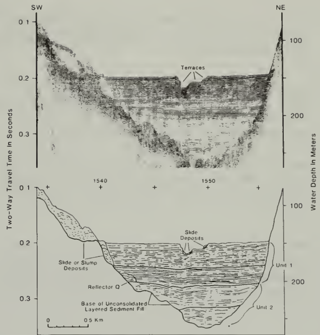
Fig. 3. Minisparker (500 J) profile and interpretive sketch from Queen Inlet showing terraces bordering main channel in mid-fjord. Vertical exaggeration, \times 9.3 . See Fig. 1 for location of profile.
