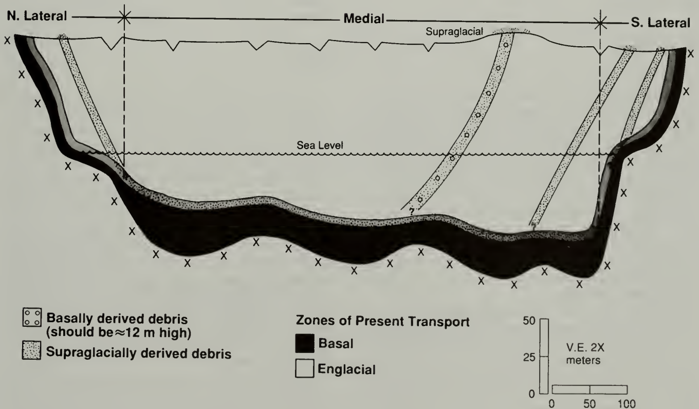
Fig. 1. Cross-section of the face of McBride Glacier showing sources of the debris that becomes iceberg-rafted.
