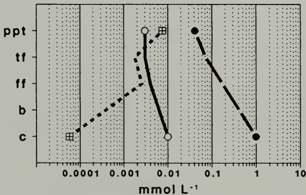
Fig. 3. Volume-weighted precipitation (ppt), volume-weighted throughfall (tf), and tension lysimeter free H + (from pH), NO 3 - , and total base cation concentration beneath the forest floor (ff) and at two mineral soil depths (b and c) in successional vegetation at South Berg.
