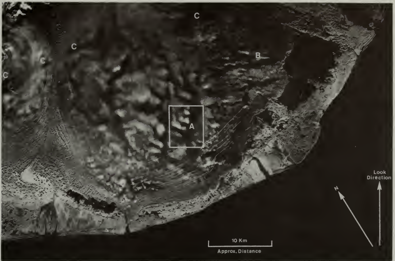
Fig. 1. Side-Looking Airborne Radar image of the lower two-thirds of Malaspina Glacier. The long narrow arcuate lines are moraines. The light and dark, irregular to rounded patterns represent topography highs and lows on the glacier's surface. The three types of surface patterns resemble glacially eroded valleys (A), dendritic morphology (B), and the surface expression of a fault (C). This X-band image was acquired on November 25, 1986, with a look direction of N. 30° E. The depression angle (the angle of microwave illumination below the horizontal) range across the image is from 9° in the southwest to 30° in the northeast. The area contained in the rectangle is shown in Figure 2.
