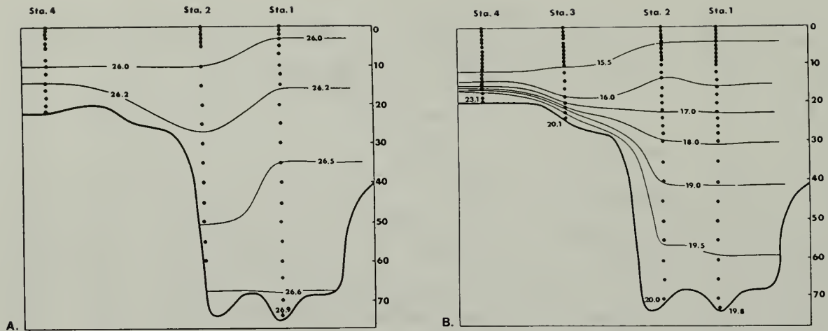
Fig. 5. Distribution of water density ( \sigma_t ) within McBride Inlet during intermediate water renewal (A) and deep water renewal (B). Data in (A) was collected at high tide on June 26-27, 1986.
