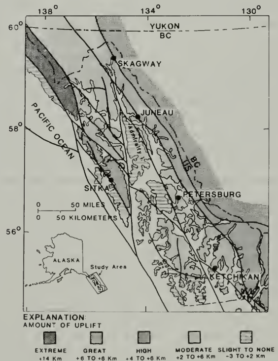
Fig. 4. Map showing generalized vertical movements of southeastern Alaska fault blocks. Displacements are relative either to depth of origin in the cases of metamorphic rocks and igneous rocks or to sea level in the case of volcanic rocks.
