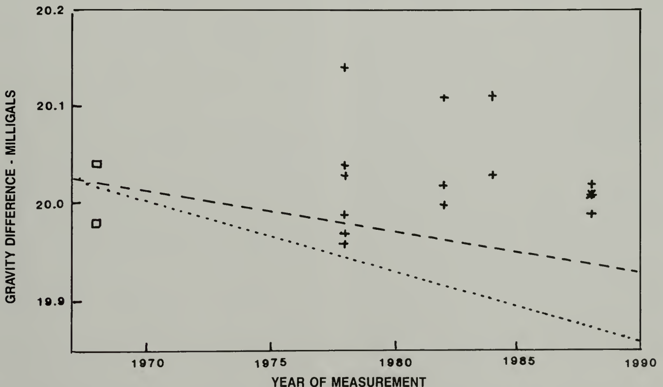
Fig. 3. Graph of measurements of the gravity difference between Juneau and Gustavus airports as a function of year of measurement. Dotted line indicates expected free-air gravity change (no addition of mass beneath uplifted station) of 2.35 cm/year for Gustavus relative to Juneau airport. Dashed line indicates expected Bouguer gravity change with addition of underlying infinite slab of mantle material having a density of 3.10 gm/cm 3 .
