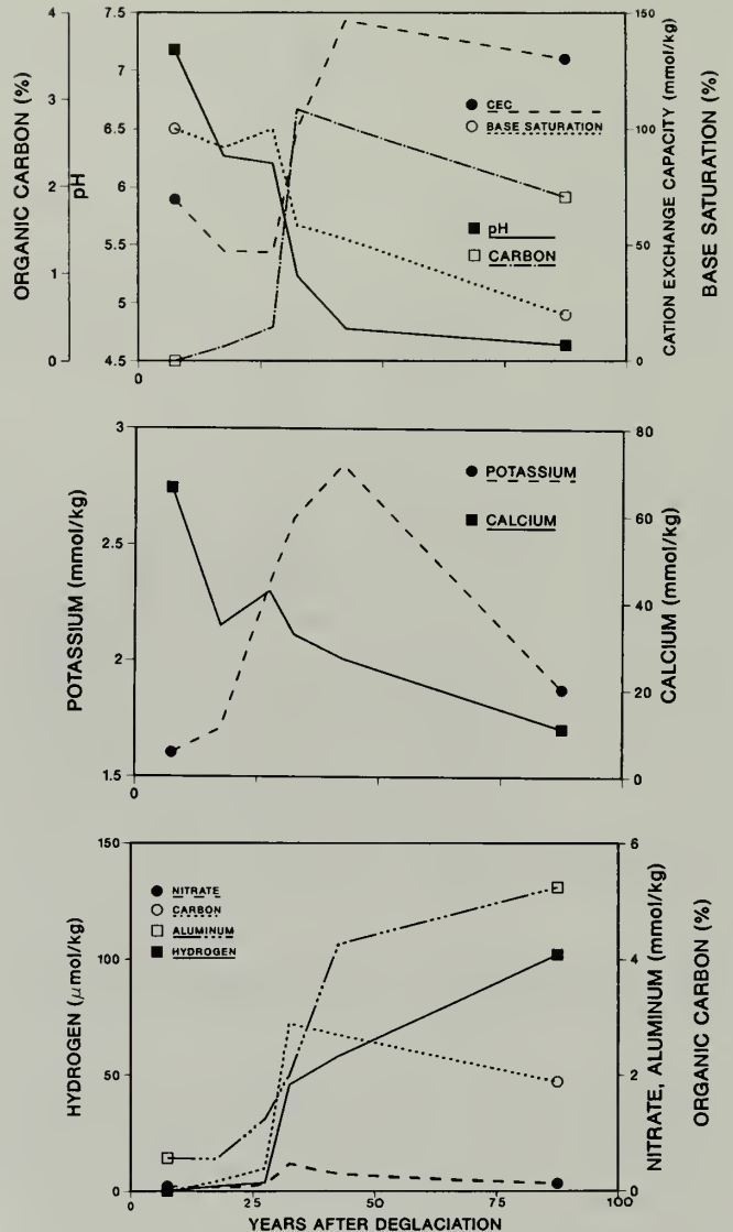
Fig. 2. Mean chemical characteristics of top 15-17 cm of mineral soil following deglaciation and before vegetation cover (0-30 years), beneath 10- and 24-year Alnus at Wolf Creek; and 55-year Populus-Alnus at South Berg.
