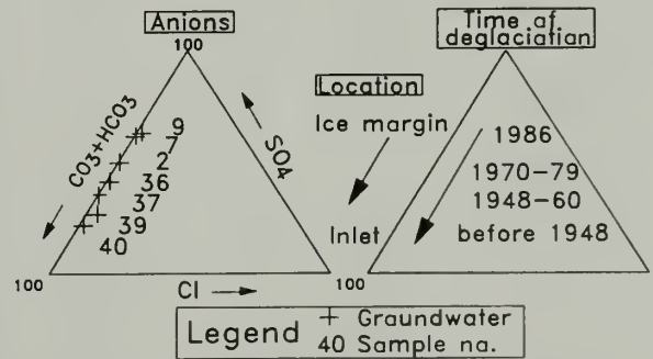
Fig. 3. Diagram demonstrating change in groundwater geochemistry from a calcium sulfate to a calcium bicarbonate water with increasing distance from the ice margin and increasing time since deglaciation.
