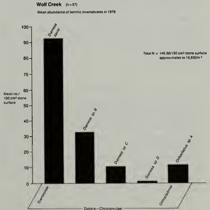
Fig. 2. Mean abundance of benthic invertebrates in 1978 from the representative sampling site in Wolf Creek.
