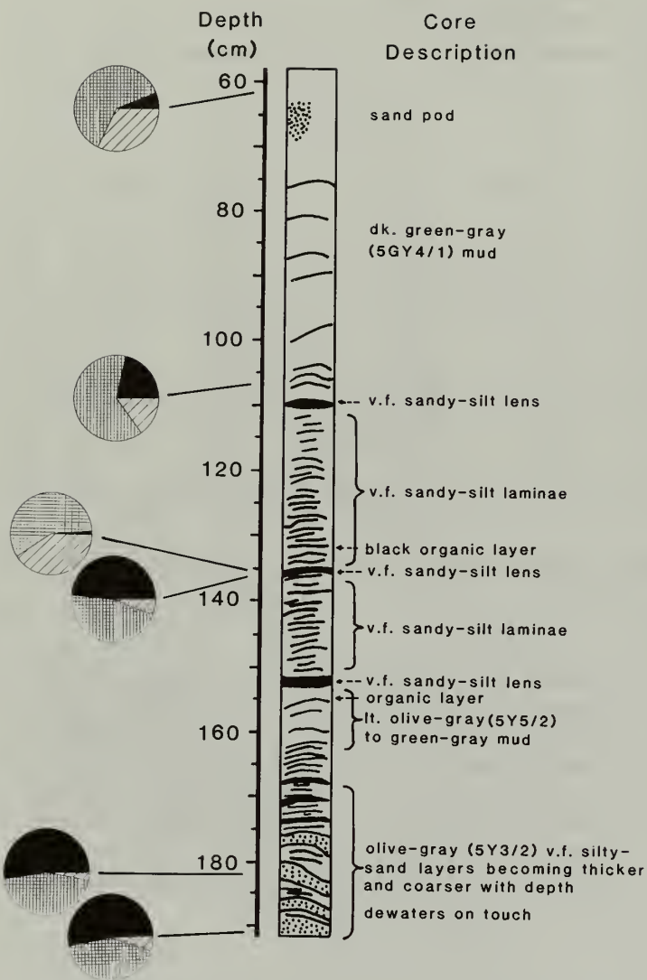
Fig. 2. Sketch of gravity core 54 collected from main channel in Queen Inlet at water depth of 150 m, and pie charts for subsamples showing percentages of sand (black), silt (squares), and clay (slanted lines). See Fig. 1 for location of core.
