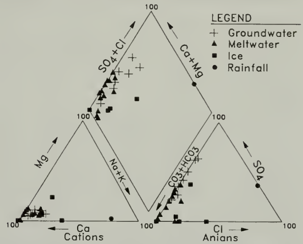
Fig. 2. Piper trilinear diagram showing percentages of cation and anion milliequivalents for all samples in the study area. Groundwater changes from a calcium sulfate to a calcium bicarbonate water with increasing distance from the ice margin.
