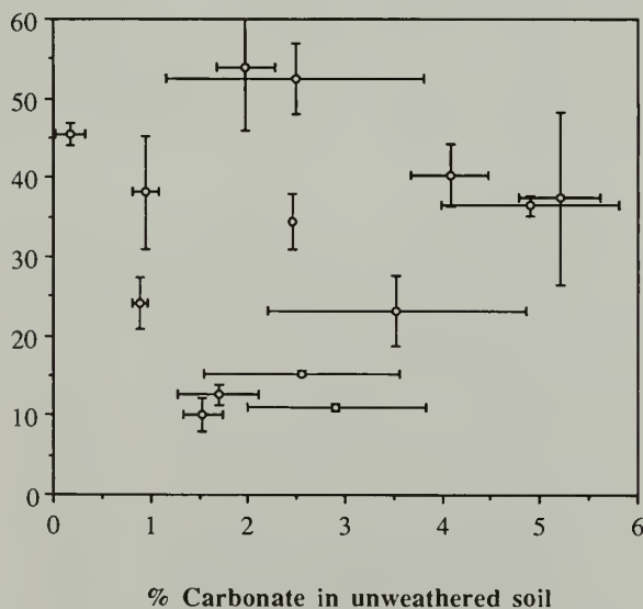
Fig. 4. Relationship between the carbonate content of unweathered soil samples and epilimnetic \text{Ca}^{+2} concentrations at study sites in the Muir Inlet area; error bars = \pm 1\sigma , representing 2-3 soil pits and 2-4 water samples (from consecutive years).
