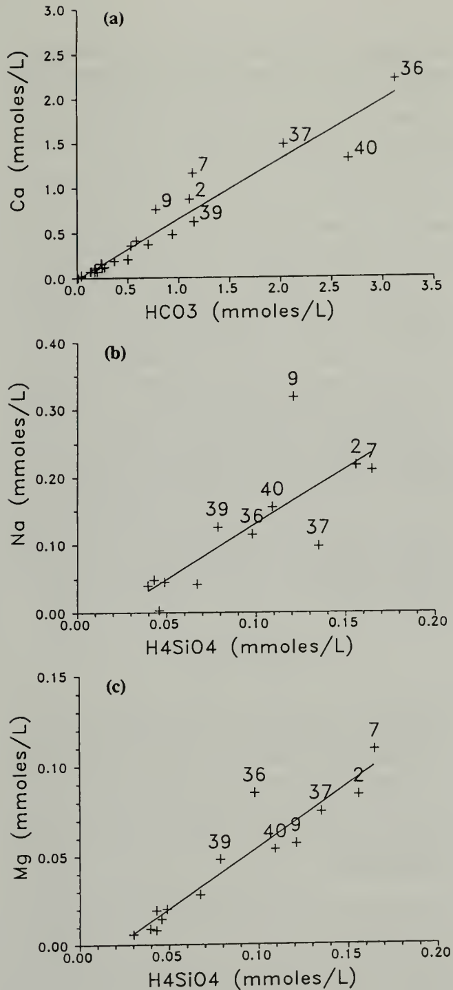
Fig. 4. (a) Plot of Ca and HCO 3 concentrations in mmoles/L. The strong relationship ( r^2 = 0.93 ) and nearly 1:2 (Ca:HCO 3 ) molar relationship suggest that calcite dissolution is the predominant reaction; (b) plot of Na and H 4 SiO 4 concentrations in mmoles/L. The 2:1 (Na:H 4 SiO 4 ) molar relationship suggests albite dissolution, but the weak correlation ( r^2 = 0.70 ) suggests incomplete dissolution of Na-silicates; (c) plot of Mg and H 4 SiO 4 concentrations in mmoles/L. The correlation ( r^2 = 0.84 ) suggests incomplete dissolution of Mg-silicates.
