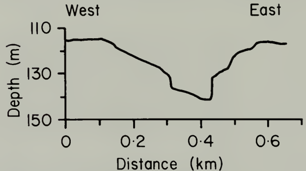
Fig. 2. Line drawing of acoustic profile of axial channel. Vertical exaggeration is 10X. See Fig. 1 for location.
