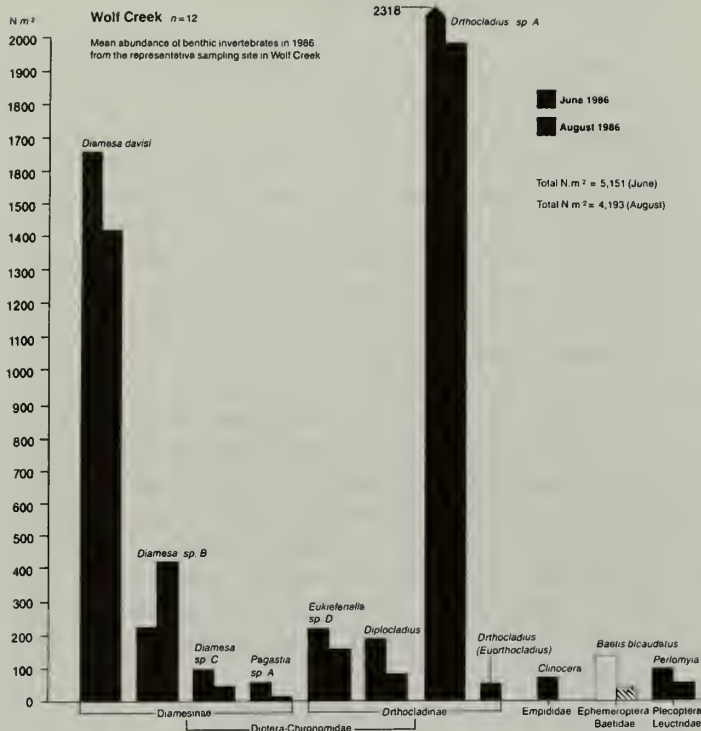
Fig. 3. Mean abundance of benthic invertebrates in 1986 from the representative sampling site in Wolf Creek.
