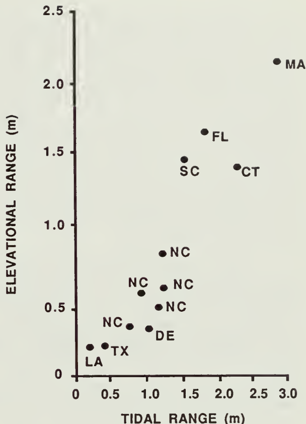
Figure 62. Elevation range of Spartina alterniflora along Atlantic and gulf coasts versus tidal range (Baumann 1980).
