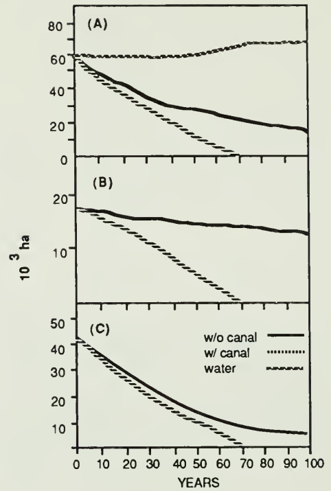
Figure 57. Conceptual model of natural and human-induced land loss (left) and the results of the simulation for total marsh area (A), streamslope marsh area (B), and inland marsh area (C) (reprinted, with permission, from Cleveland et al. 1981, copyright Elsevier Scientific Publishing Co.).
