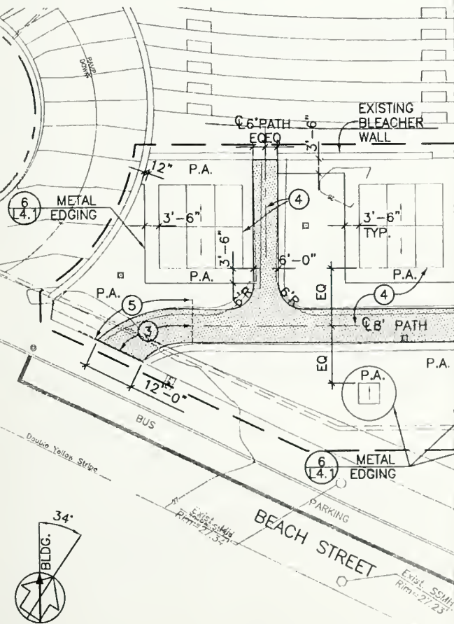
2 (L1.0) LANDSCAPE LAYOUT - CENTER AREA
