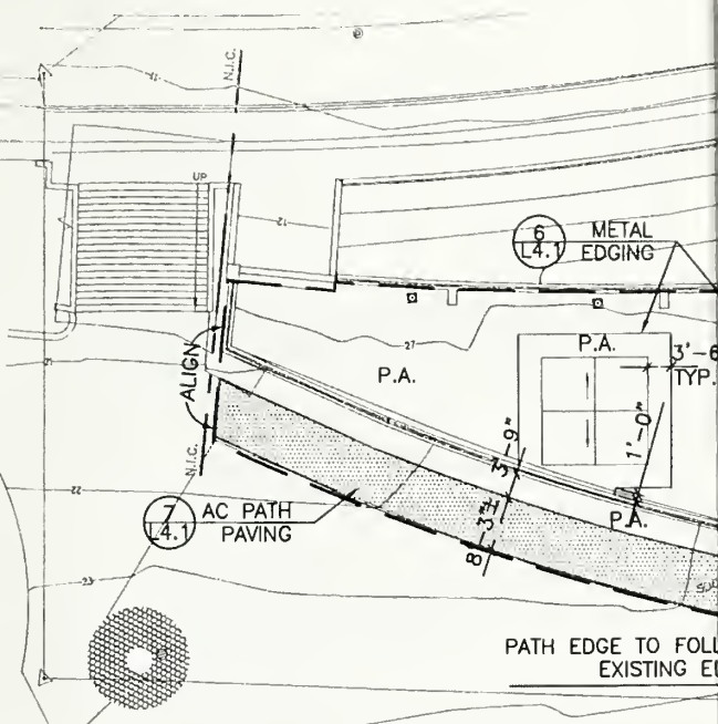
1 (L1.0) LANDSCAPE LAYOUT - WEST AREA
