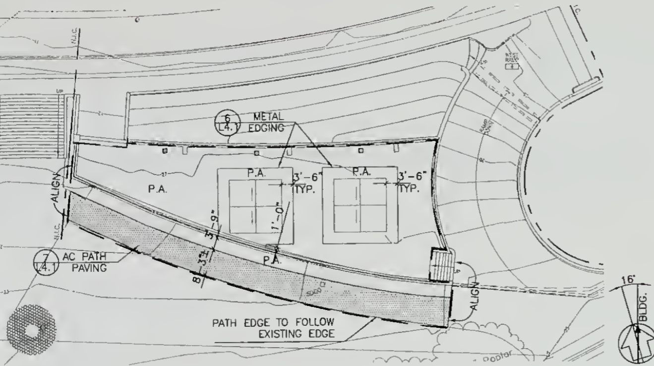
1 LANDSCAPE LAYOUT - WEST AREA L1.0
