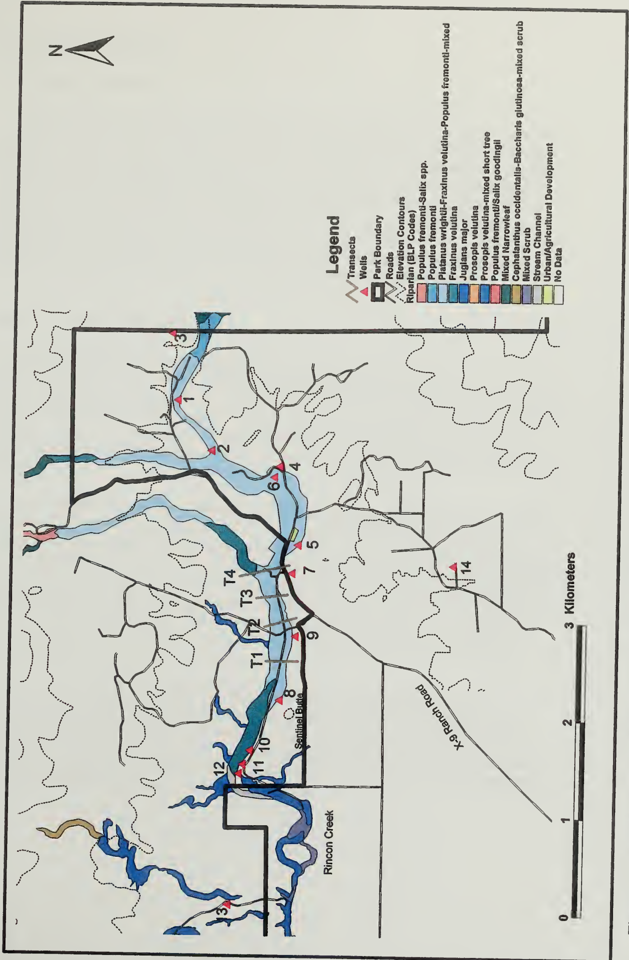
Figure 17. Middle basin riparian areas: Rincón Creek.
