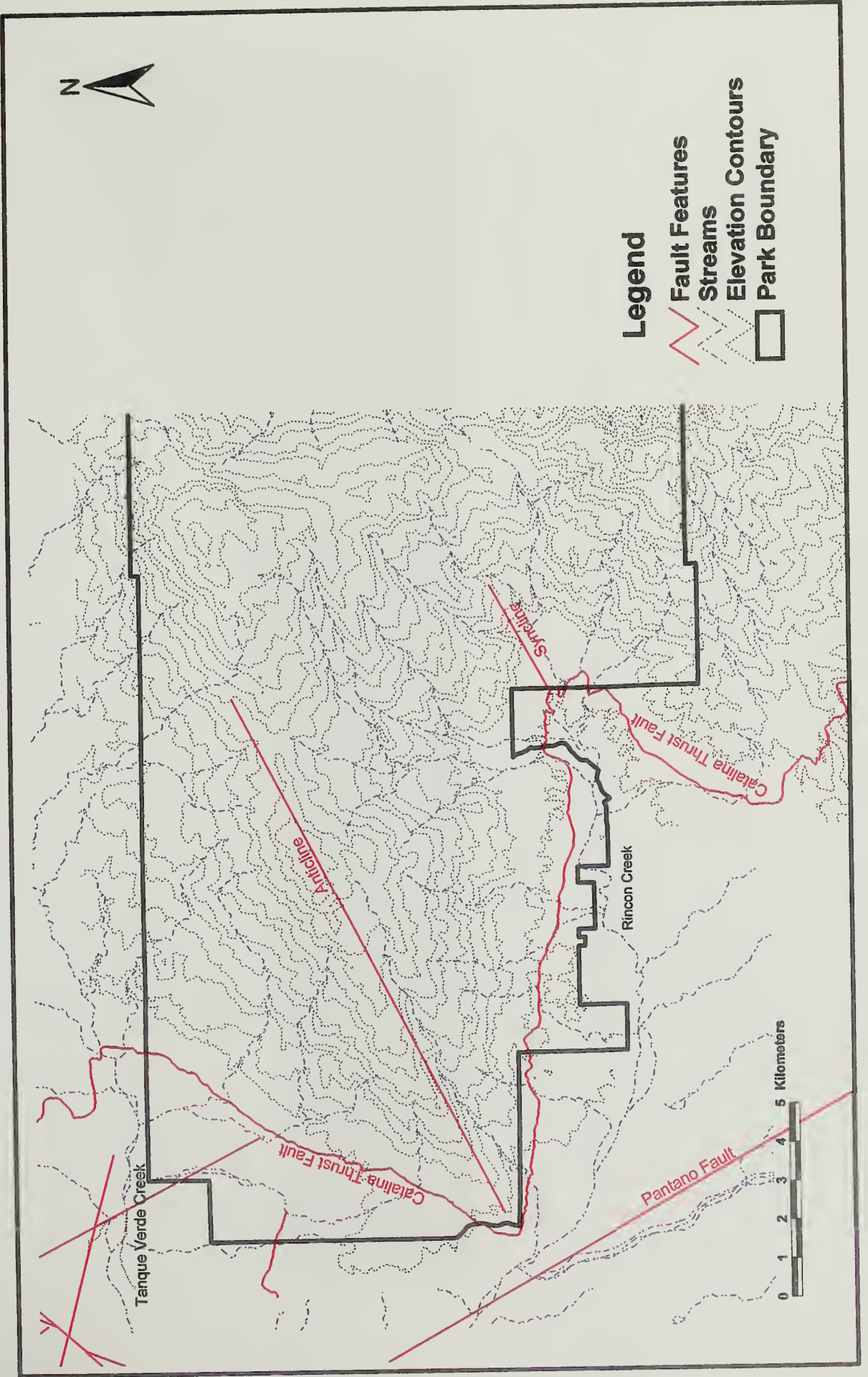
Figure 3. Major Faults in the vicinity of Rincón Creek.
