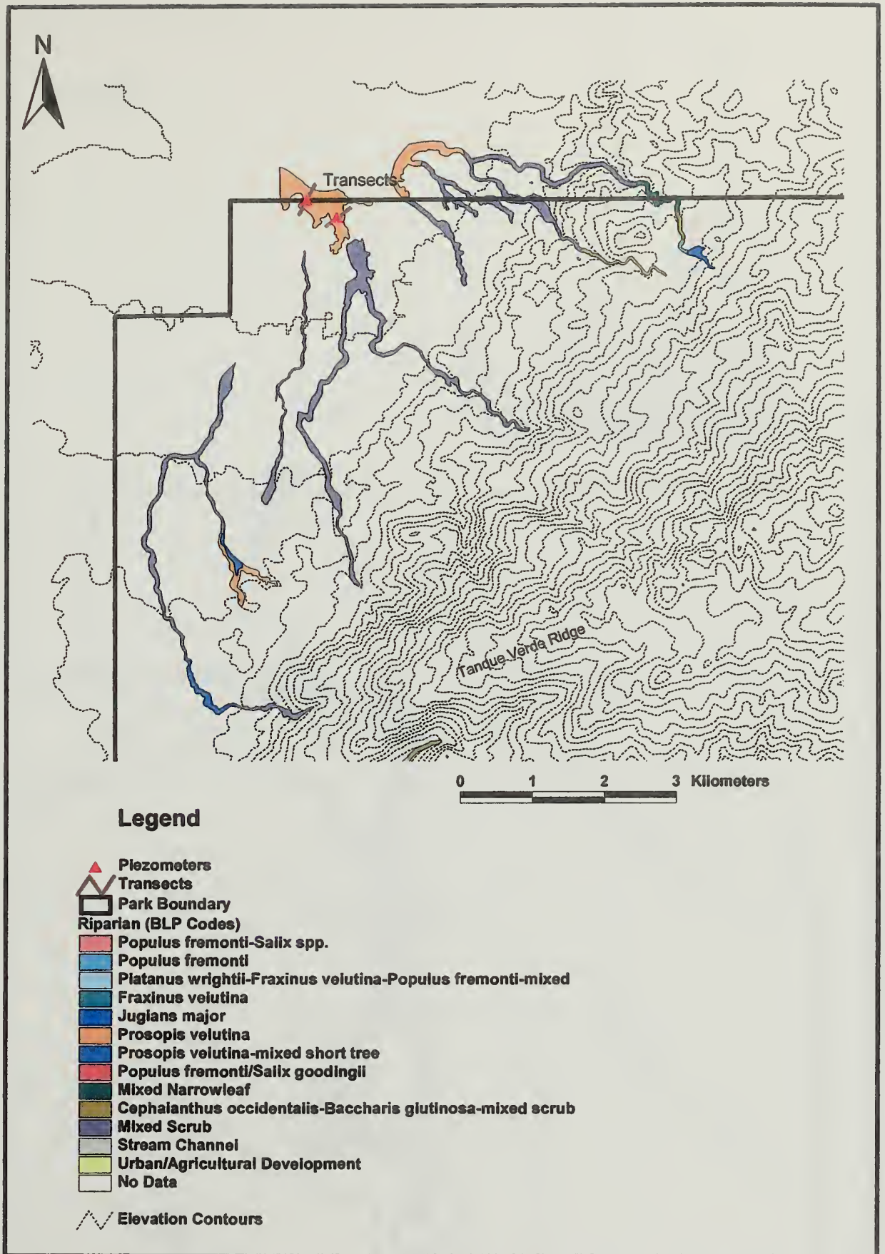
Figure 16. Riparian areas: Tanque Verde Creek tributaries.
