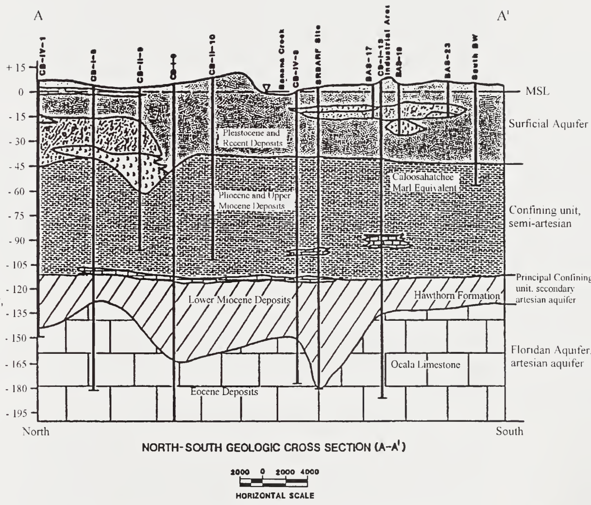
Figure 18 - North-South Geologic Cross-Section
