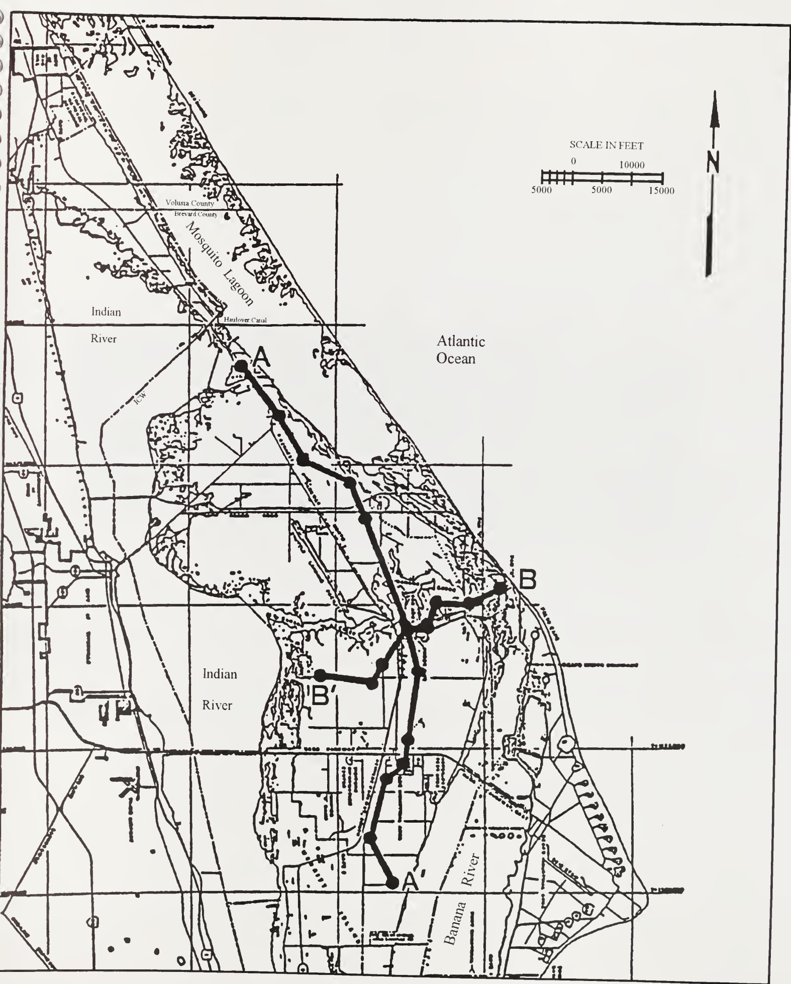
Figure 16 - Soil Boring Locations For Geologic Cross-sections
