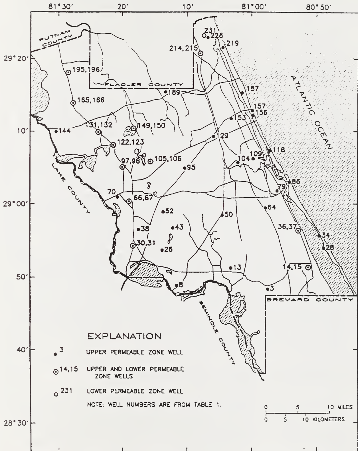
Figure 19: Well Locations (from Belanger et al. 1997)
