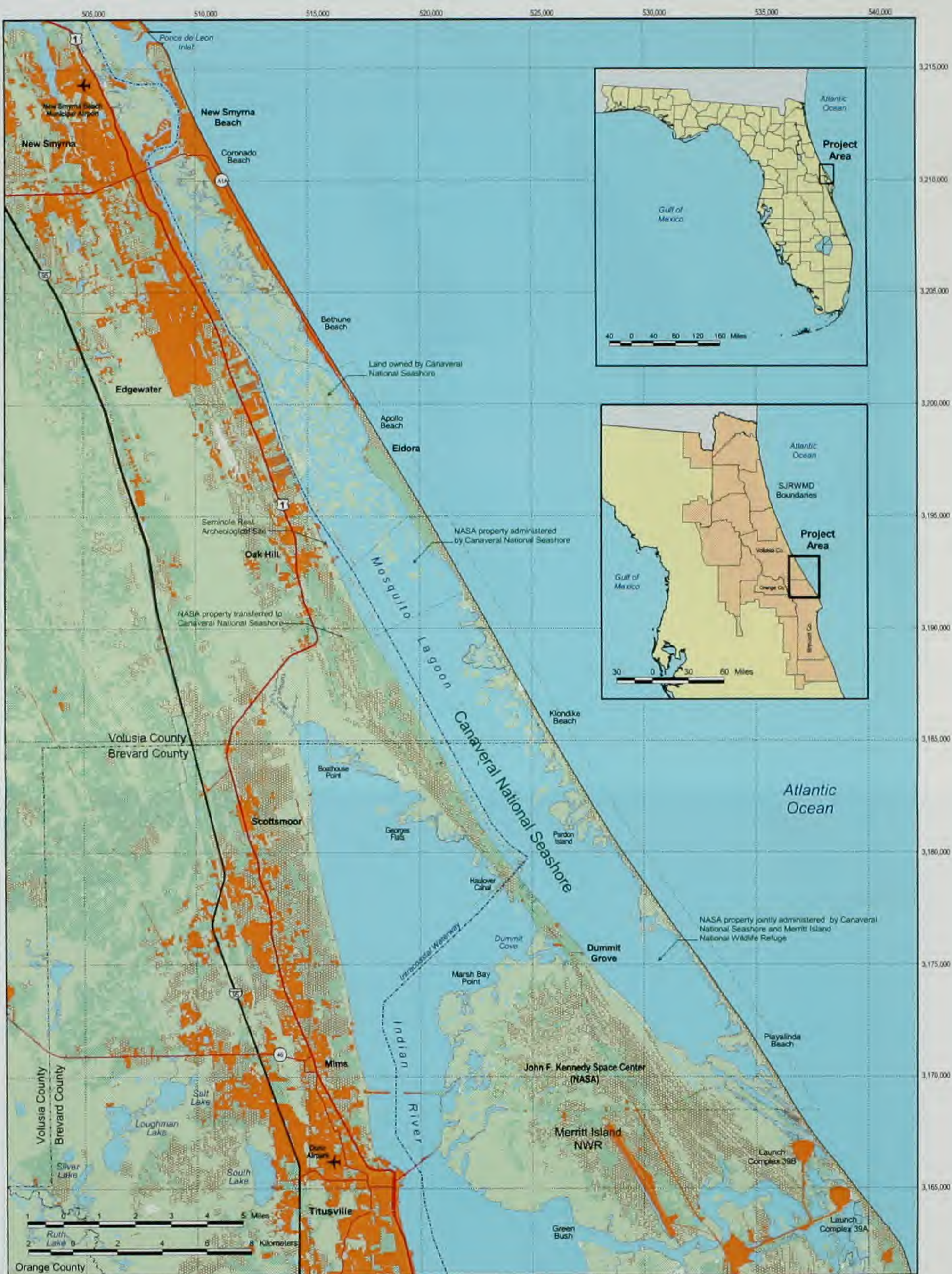
Figure 4. Land Use 1995
