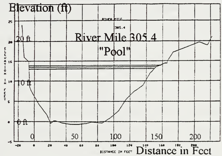
Figure 4.5.a. Shoal, run, and pool habitat types in the Chattahoochee River, Buford Dam and Peachtree Creek (after Nestler et al., 1984).
