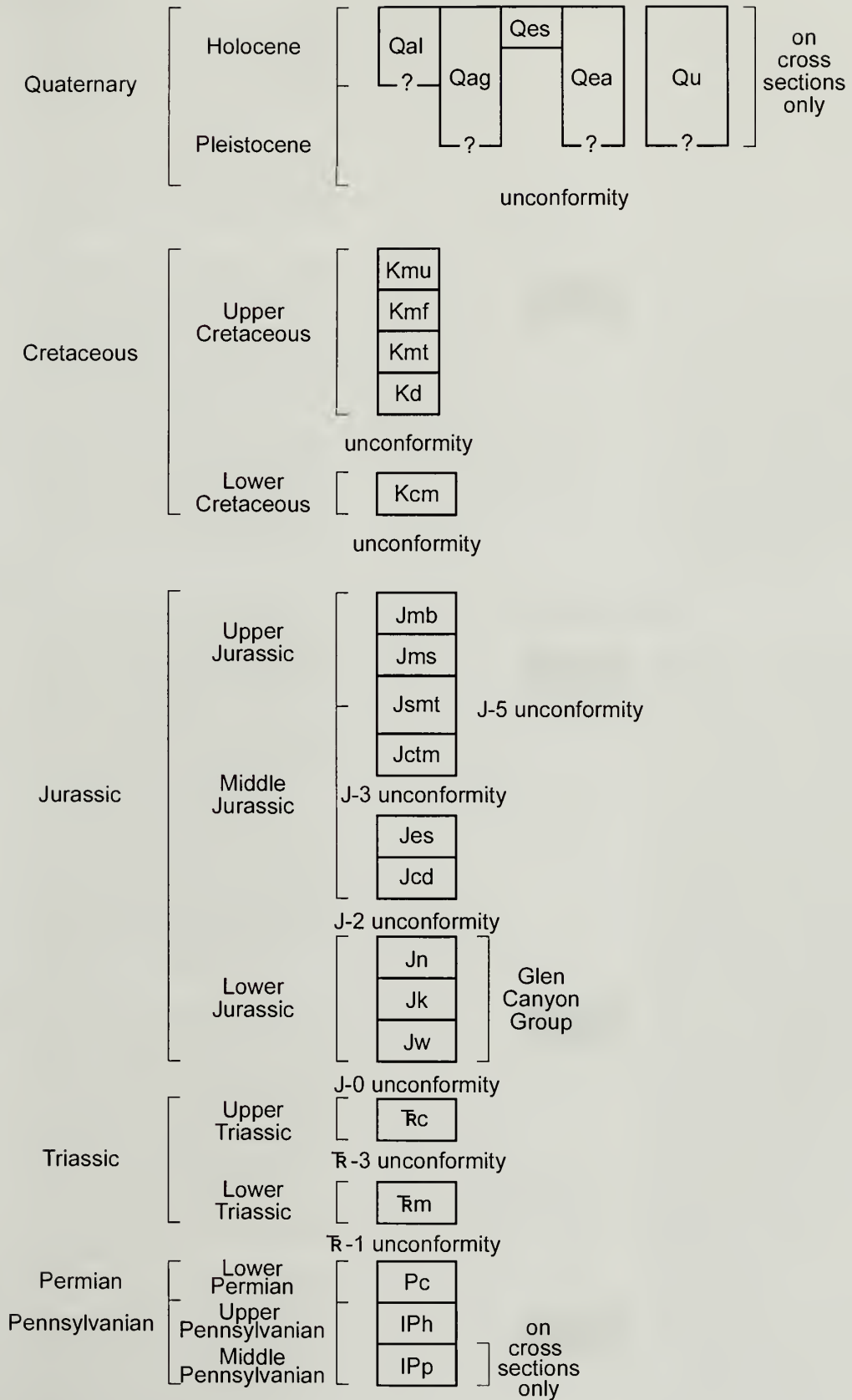
Figure A.2. Correlation of geologic units.
