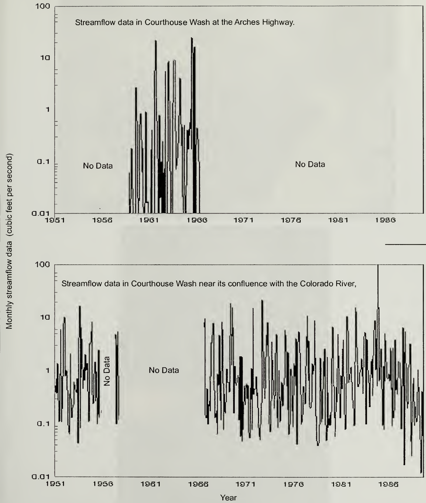
Figure 10. Hydrographics of Courthouse Wash at Arches Highway and near its confluence with the Colorado River (U.S. Geological Survey [2002b]).
