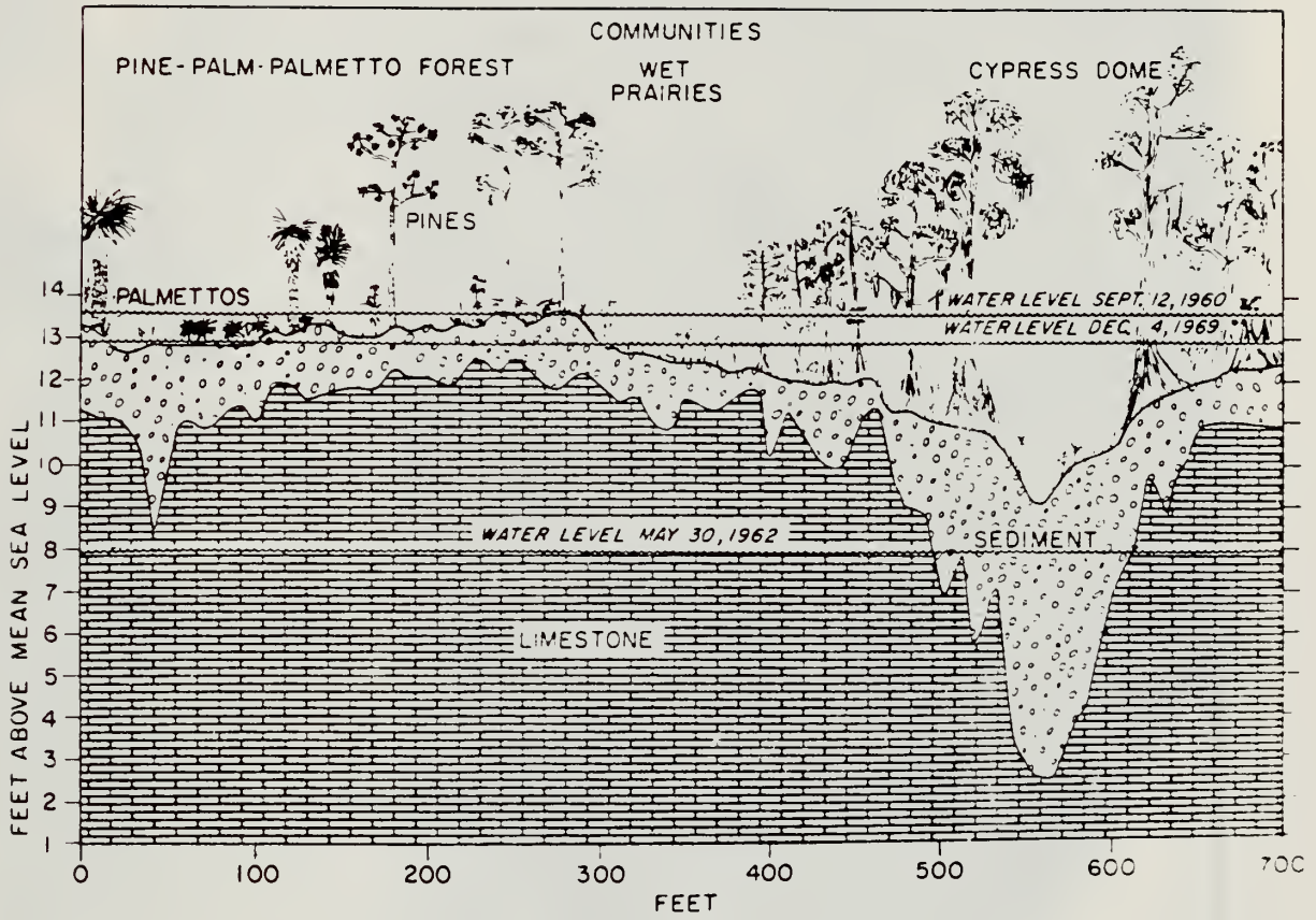
Figure 2-9. Vegetal transect in the Big Cypress showing pine-palm-palmetto forest through a cypress-tree community.
