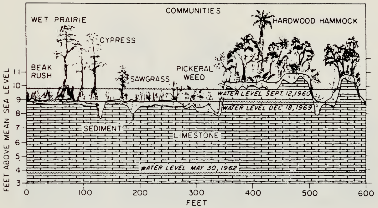
Figure 2-6. Vegetal transect in the Big Cypress showing wet prairie into a hardwood hammock.
