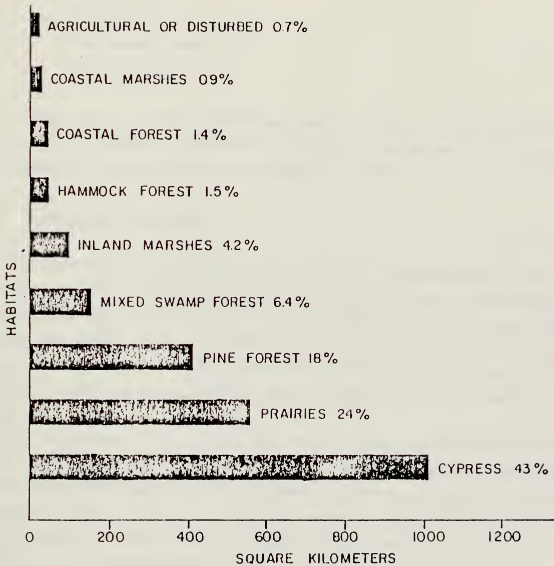
Figure 2-2. Areas of major habitats in the Big Cypress National Preserve (McPherson, pers. comm.).
