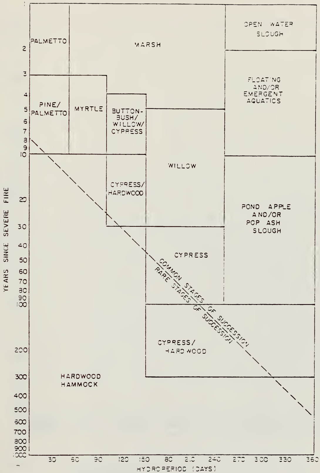
Figure 2-3. Successful patterns and rates in inland plant communities in South Florida (Duever et al., 1976).
