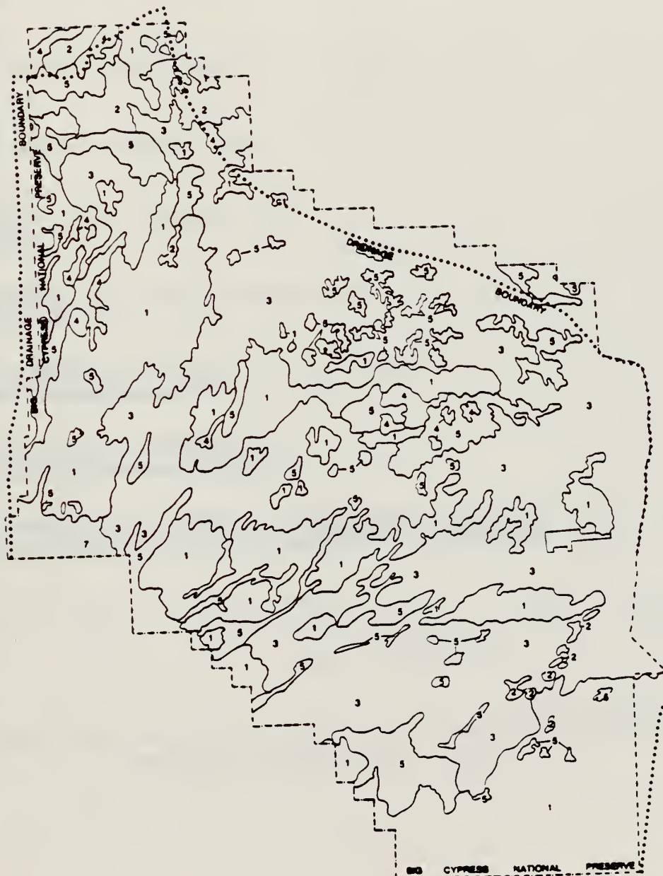
Figure 2-1. Land cover in the Big Cypress National Preserve.
