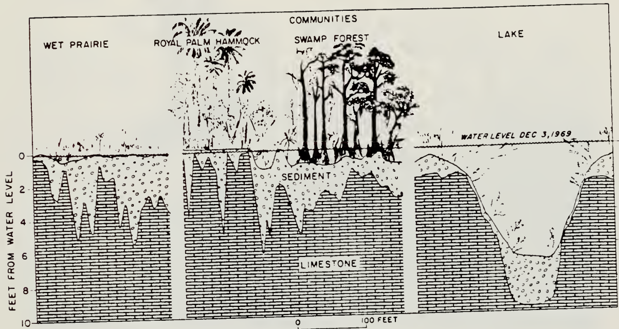
Figure 2-7. Vegetal transect in the Big Cypress showing wet prairie, hammock, swamp forest, and lake in the Fakahatchee Strand.
