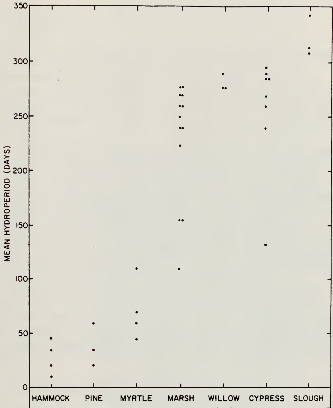
Figure 2-4. Mean hydroperiods for 43 sites at Corkscrew Swamp Sanctuary over a 14-year period.
