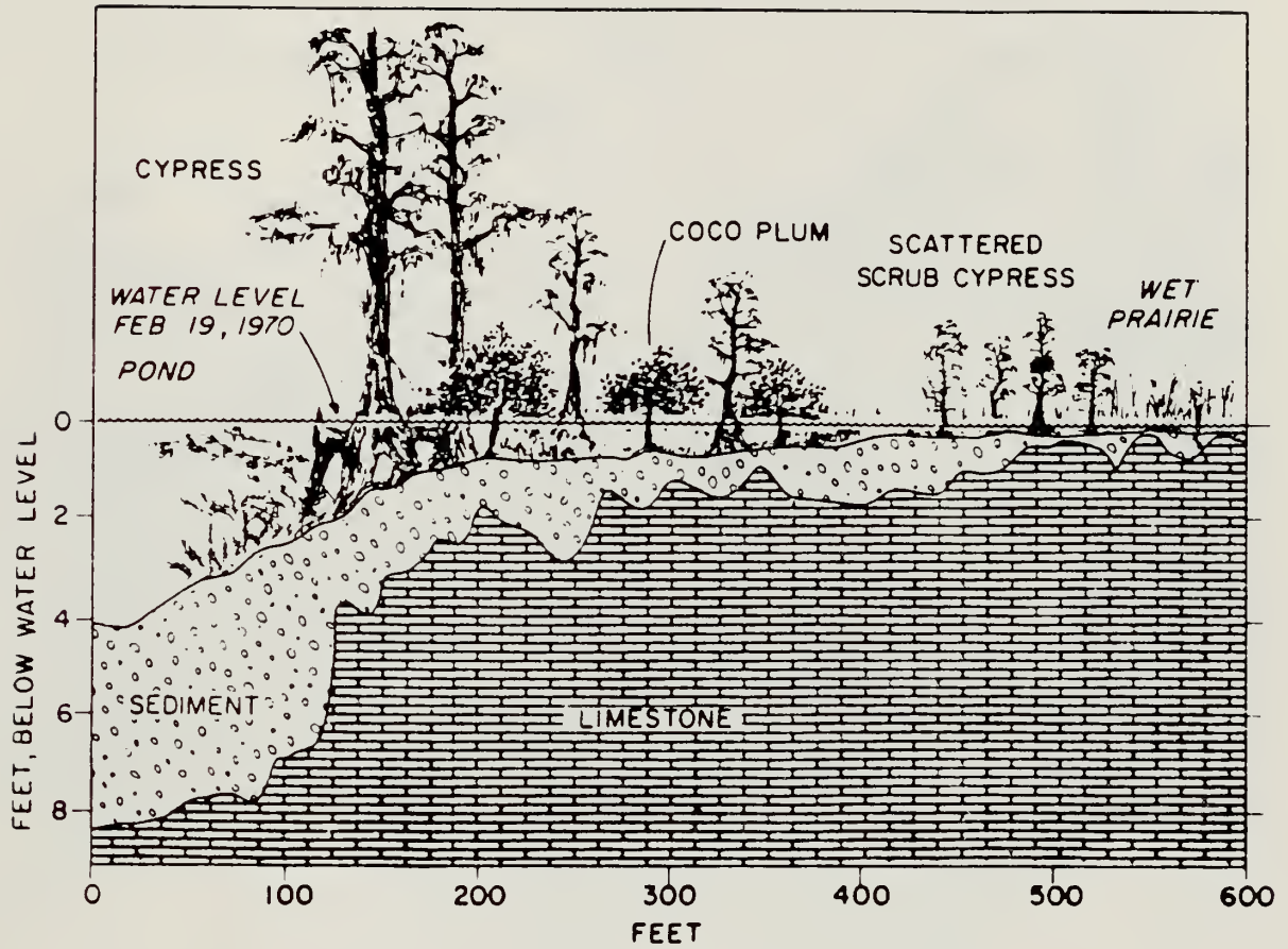
Figure 2-8. Vegetal transect in the Big Cypress showing wet prairie into a cypress strand.
