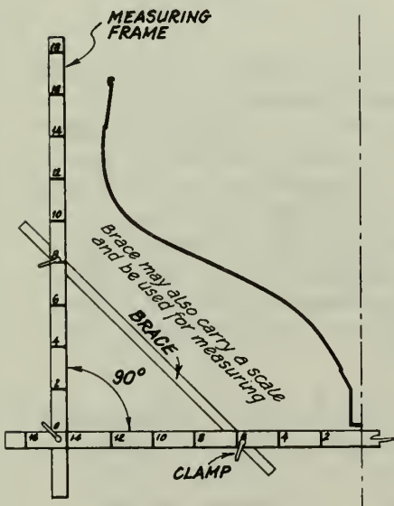
Fig. 4.2.16 Taking Sections with External Measuring Frames
