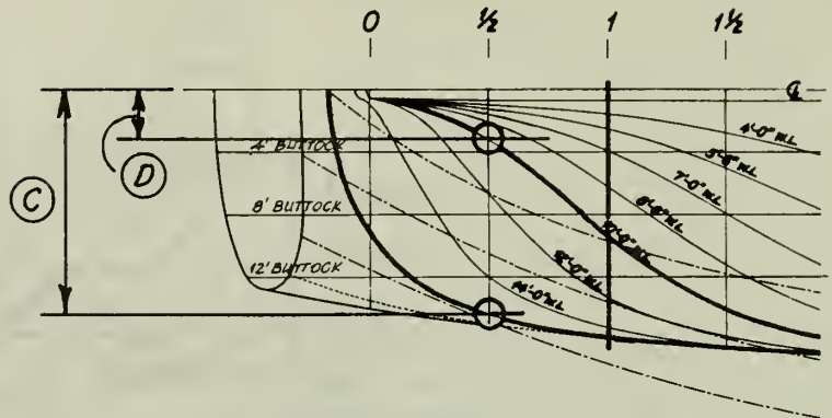
HALF-BREADTH PLAN
