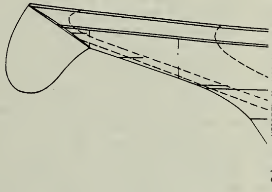
Schooner MILDRED V. NOONAN, HAMMS No. 2-46 Sheet 2 of 2
