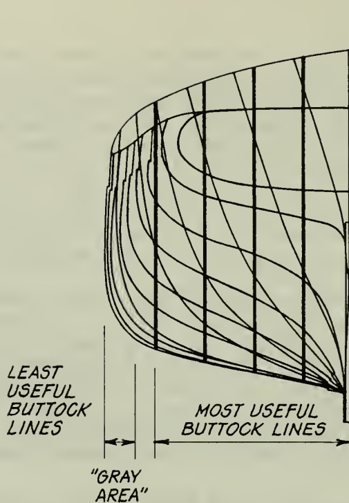
Fig. 4.5.34 Choosing Buttock Line Intervals
