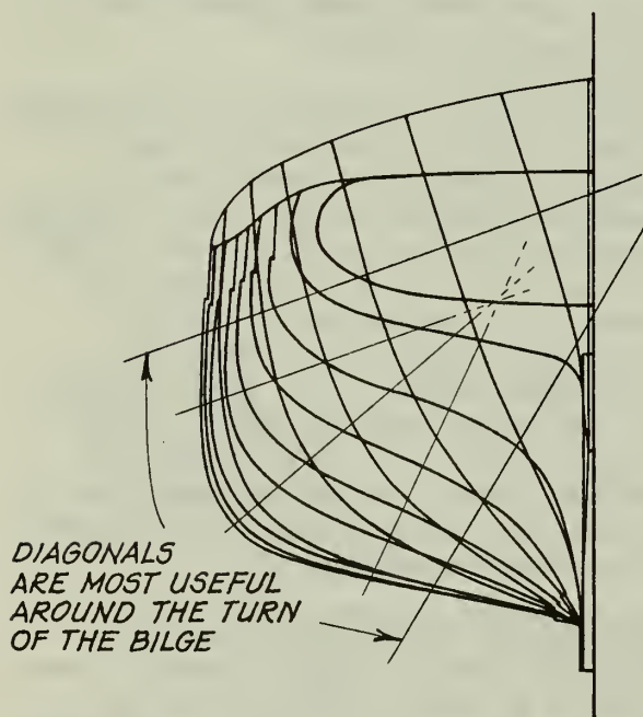
Fig. 4.5.35 Choosing Diagonals
