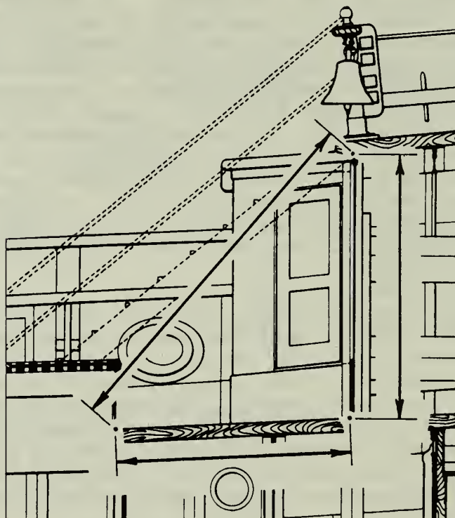
Fig. 4.2.36 Measuring Inclined Features
