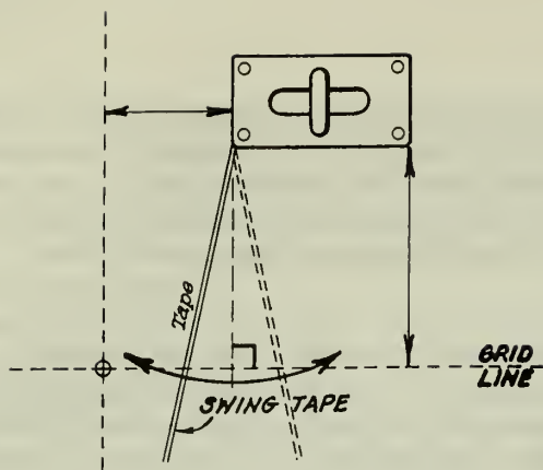
Fig. 4.2.27 Offsets from Grid Lines
