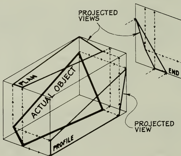
Fig. 4.2.25 Projected vs. Actual Dimensions
