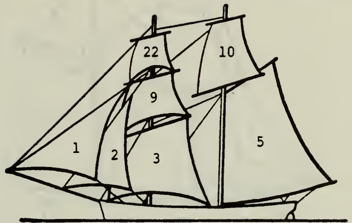
BRIGANTINE (archaic)
