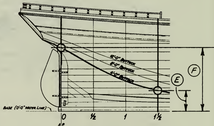
SHEER PLAN
