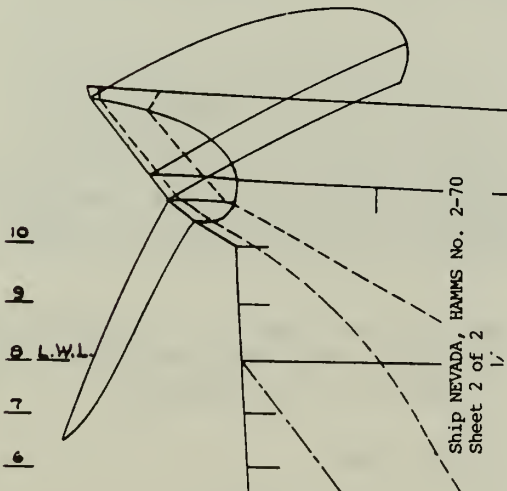
Fig. 4.5.29 Transom Expansions
