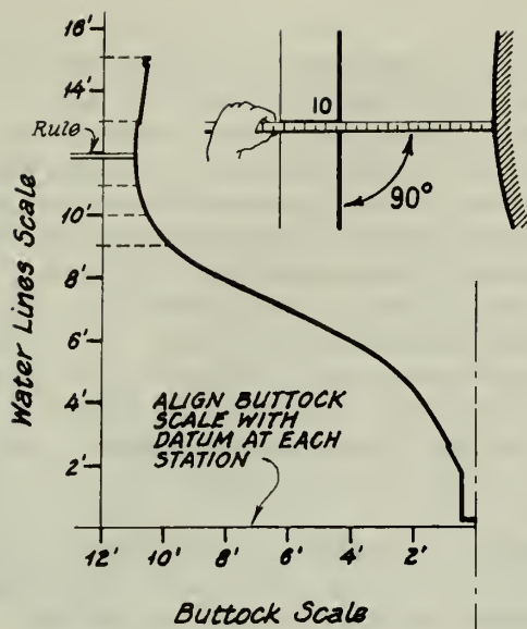
Fig. 4.2.17 Points with a Stick Rule
