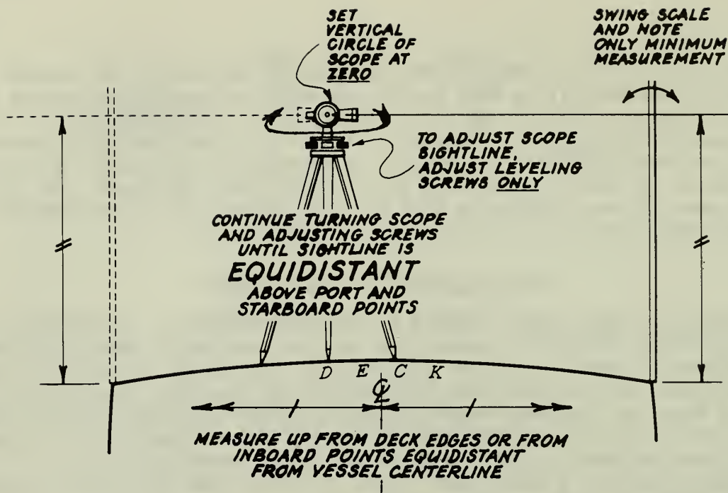
Fig. 4.2.35 "Leveling" Transit Port and Starboard
