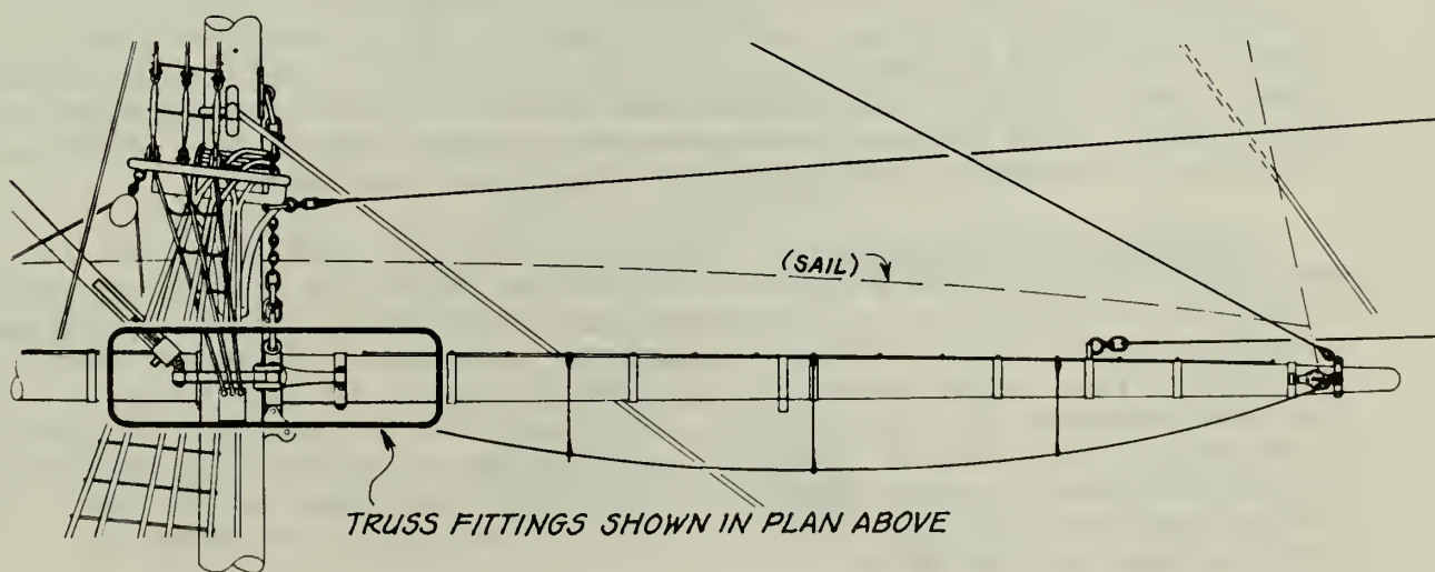
Fig. 4.5.45 How to Draw Braced Yards in an Outboard Profile
