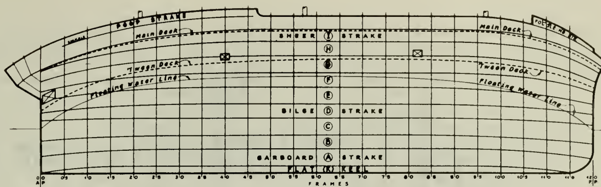
Fig. 4.2.31 Shell Expansion Plan
