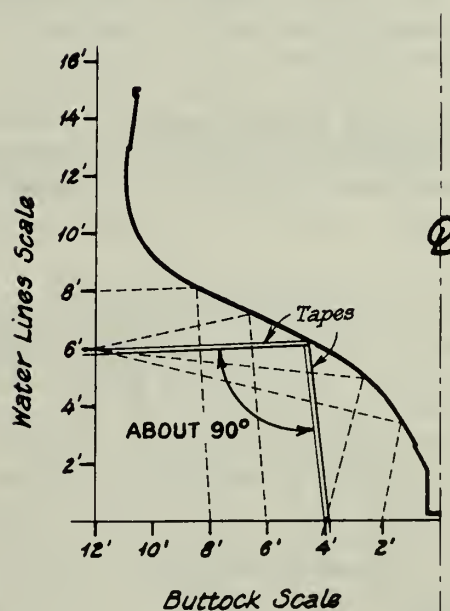
Fig. 4.2.20 Points by Quadrangulation
