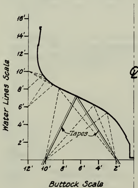
Fig. 4.2.19 Points by Triangulation
