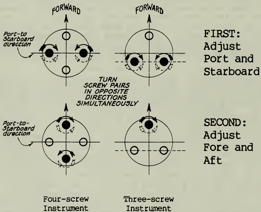
Fig. 4.2.34 Adjusting Leveling Screws
