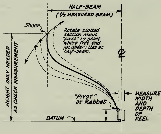
Fig. 4.2.12 Locating Section with Rabbet and Half-breadth
