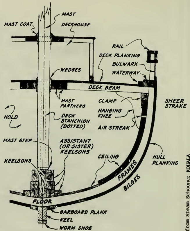
Section through Wooden Vessel
