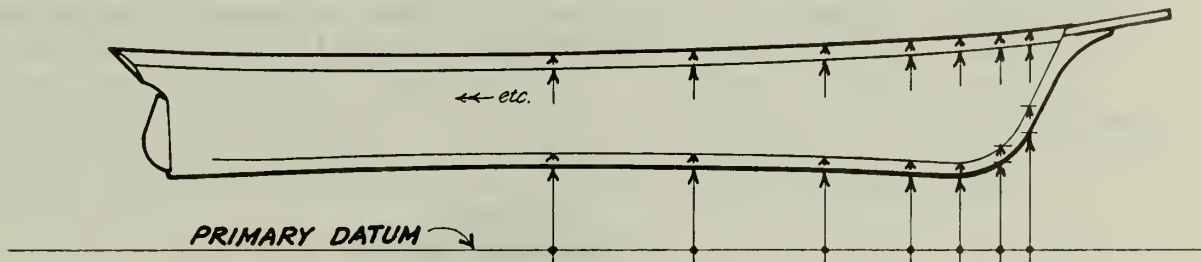
Fig. 4.2.10 Using an Independent Datum Line
