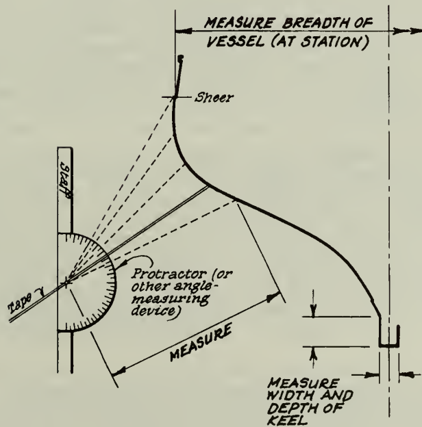
Fig. 4.2.24 Taking Sections with Range and Bearing
