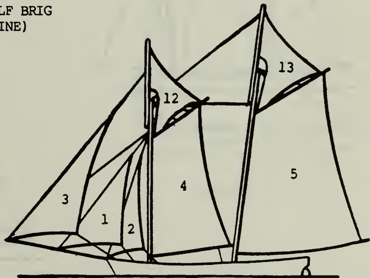
SCHOONER (Some examples had 3, 4, 5, 6 and 7 masts)
