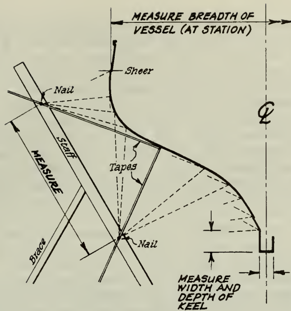
Fig. 4.2.23 Taking Sections with Staff and Tapes
