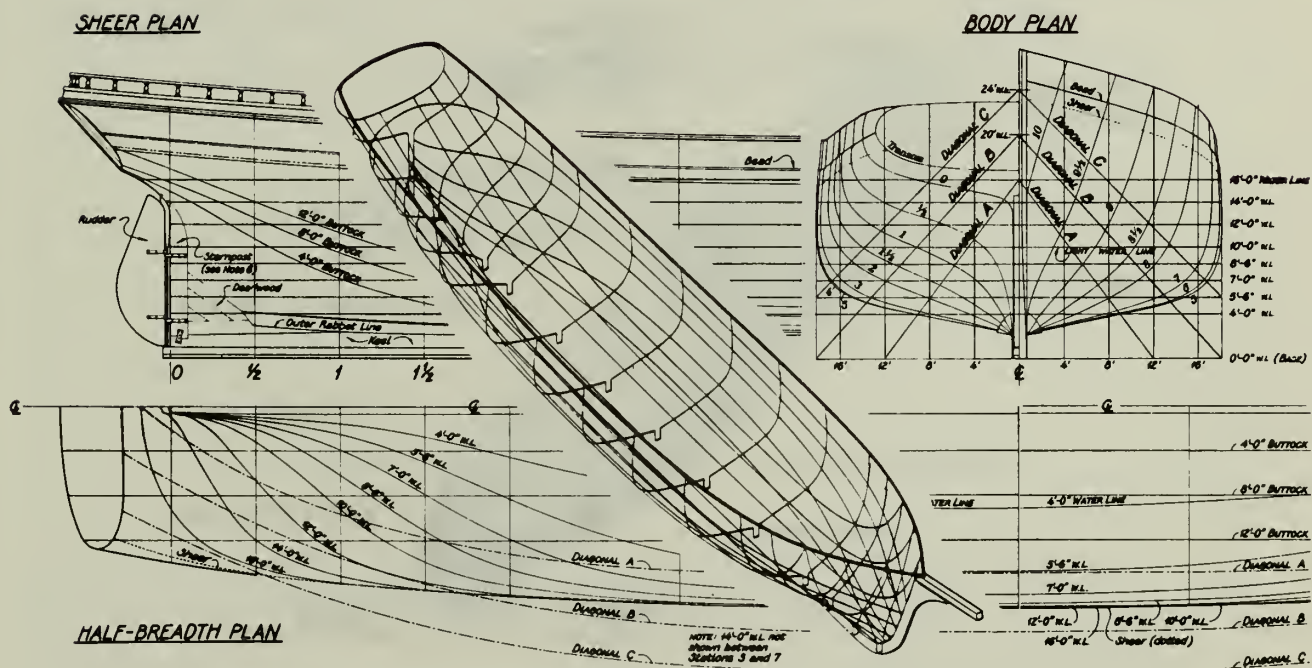
Fig. 4.1.2 The "Lines" or Contours of a Hull
