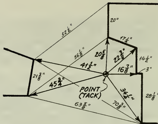
Fig. 4.2.28 Using Arbitrary Triangulation Points
