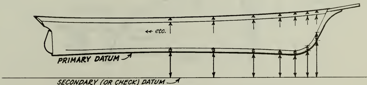
Fig. 4.2.11 Using Keel as Datum Line
