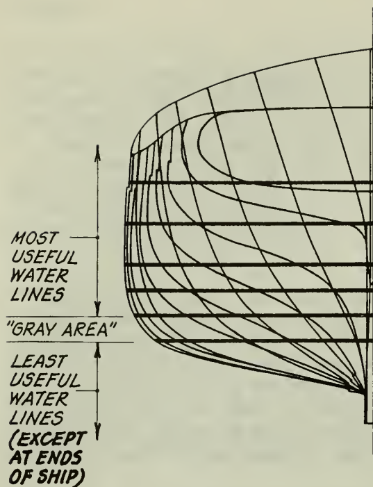
Fig. 4.5.33 Choosing Water Lines Intervals
