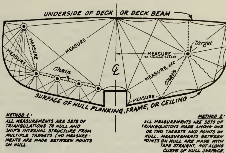
Fig. 4.2.15 Lines (Sections) from Inside a Hull
