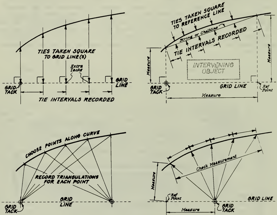
Fig. 4.2.30 Measuring Curved Features in Plan
