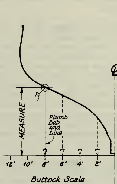
Fig. 4.2.18 Points with a Plumb Bob
