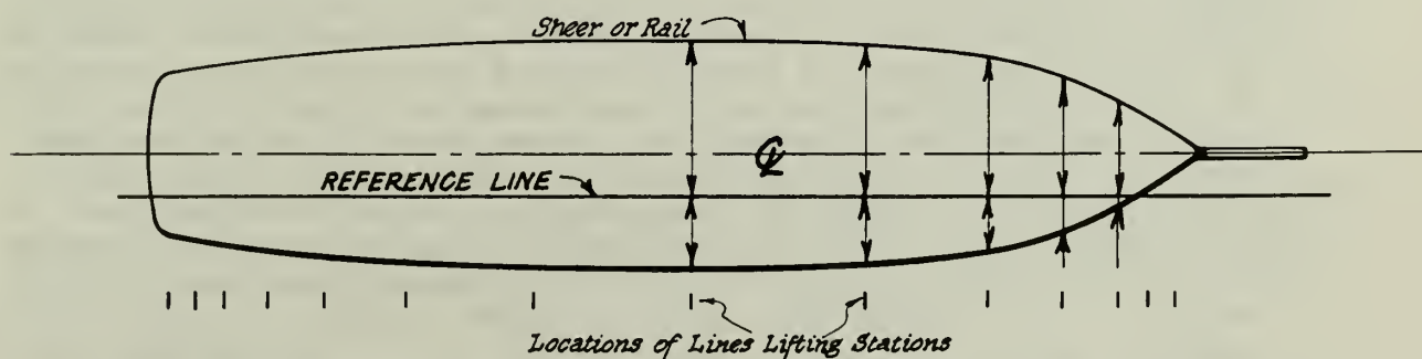
Fig. 4.2.13 Reference Line for Taking Beam Measurements
