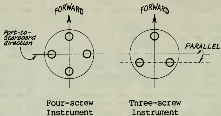
Fig. 4.2.33 Lining Up Transit Leveling Screws With Ship Coordinates
