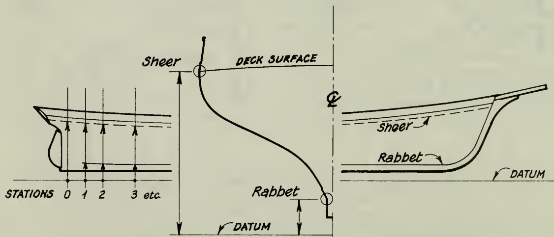
Fig. 4.2.21 Measuring Sheer and Rabbet Lines
