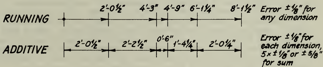
Fig. 4.2.1 Running vs. Additive Measurements
