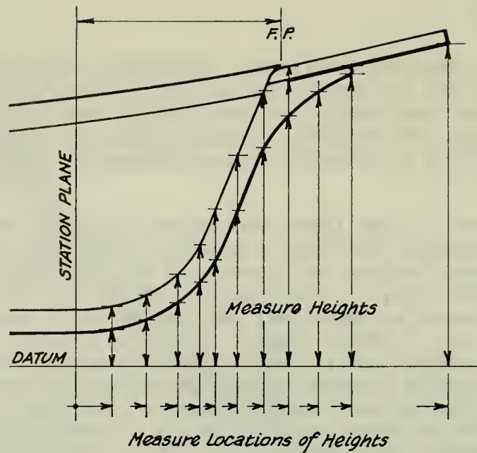
Fig. 4.2.9 Taking Profile of Stem (Triangulations or quadrangulations also useful; see Figs. 4.2.19-20)
