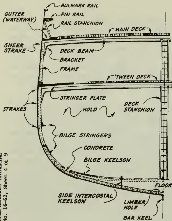
Section through Metal Vessel
