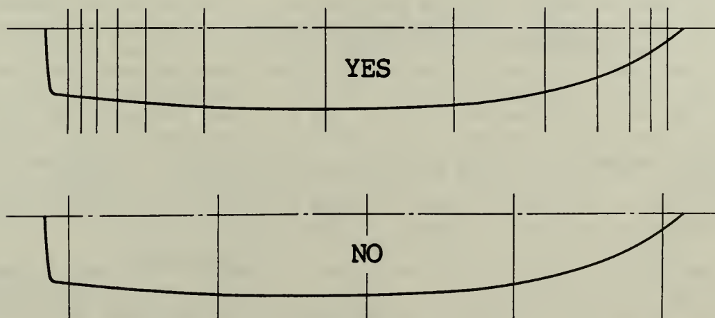
Fig. 4.2.8 Location of Stations
