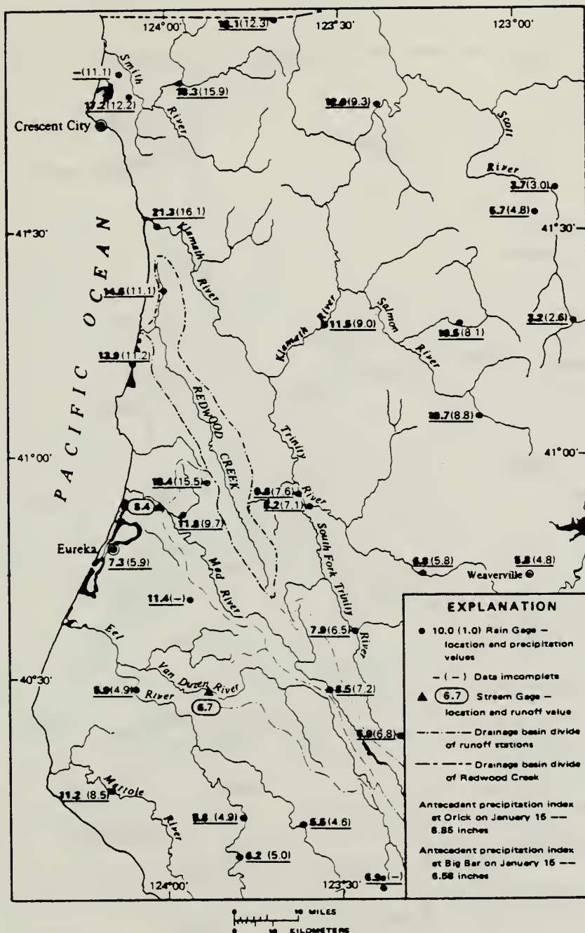
FIGURE 2. Precipitation and runoff, in inches, during the flood-producing storm of January 16-20, 1953 in north-western California. Numbers outside of parentheses are rainfall totals for the storm, and numbers within parentheses are rainfall totals for the three-day period, January 17-19, 1953.
