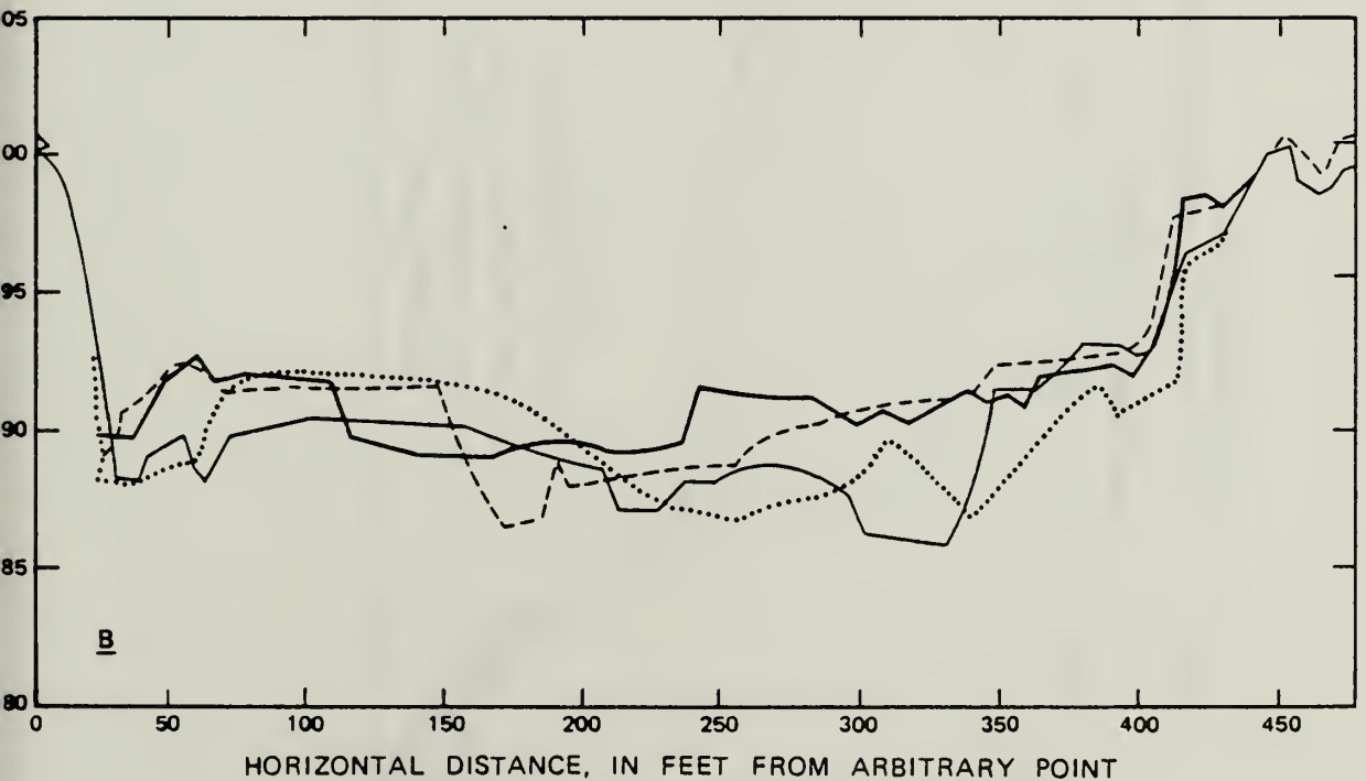
FIGURE 9. — Recent changes in stream-channel geometry along Redwood Creek. A. Mouth of gorge near southern boundary of park (1973 channel probably reflects aggradation during winter of 1971-1972); B. "Canoe Crossing Flat" downstream from mouth of Harry Wier Creek (Overbank deposition took place only in March 1975).
