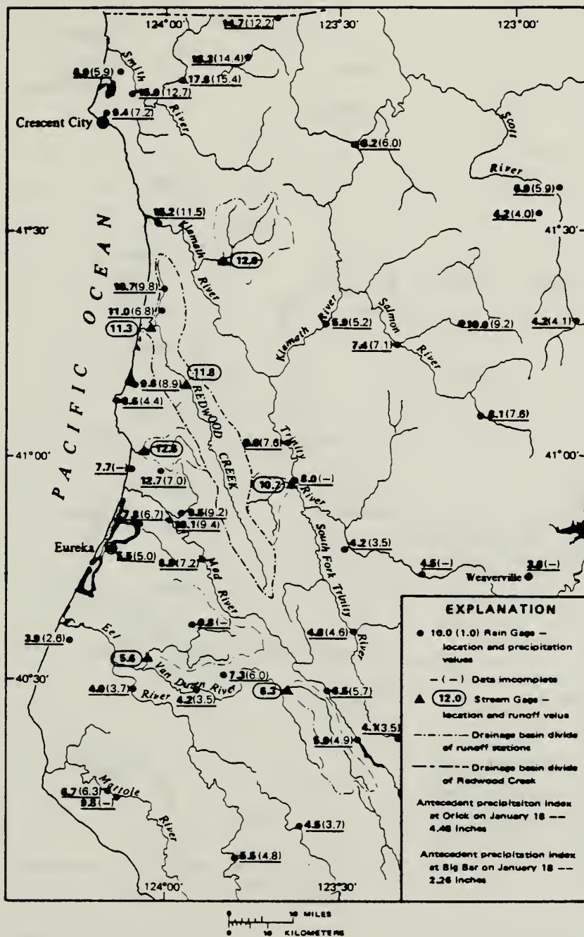
FIGURE 6. Precipitation and runoff, in inches, for the flood-producing storm of January 19-24, 1972 in northwestern California. Numbers outside of parentheses are rainfall totals for the storm, and numbers within parentheses are rainfall totals for the three-day period, January 21-23, 1972.
