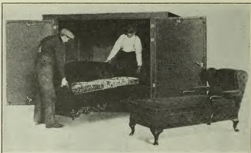
FIGURE 30.—A fumigating room installed by the Bureau of Entomology. This room is 8 by 10 by 6 feet, of steel construction, equipped with an exhaust fan connected with a galvanized-iron pipe through which the fumigant is blown to the roof of the building. The room is installed on the second floor of a 3-story building, and the exhaust pipe runs up the outside of the building. Gas in lethal strength has been held in this room for a number of days. Similar good rooms from the standpoint of tightness and good results can be built of wood, cement, or brick
