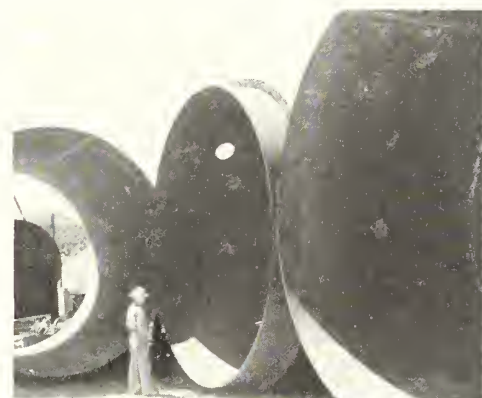
Shasta's huge power pipes.
