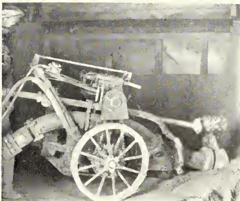
The cement unloading monster.
