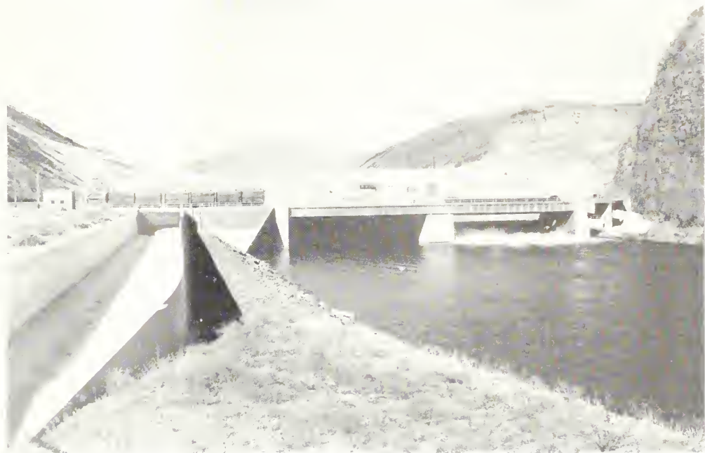
Looking north over dam from Northern Pacific Railway. Left to right: Auxiliary power and transformer house, fish screens and bench flume, dam and control house center, fish ladder and road
