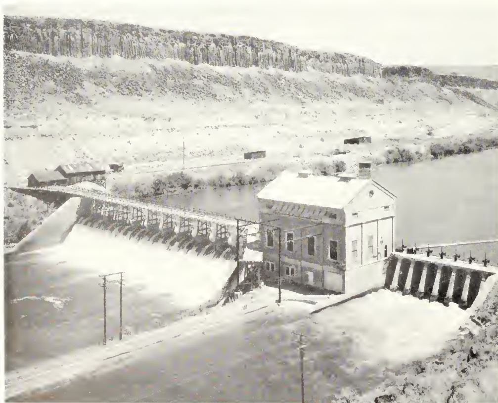
Boise diversion dam and power plant
