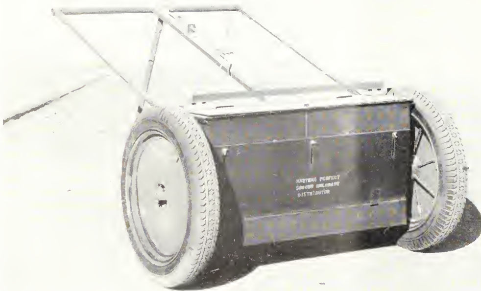
Figure 4.—Applicator for spreading dry sodium chlorate for weed control. This two-wheeled chassis is easier to manipulate than the single-wheeled one
