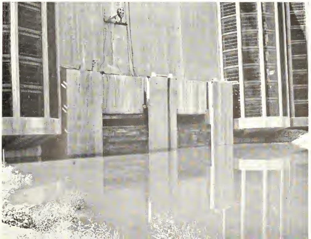
Upstream face of Marshall Ford Dam, showing the reservoir at elevation 550. The power plant was under construction when this exposure was made
