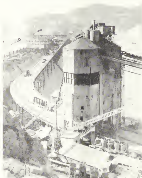
Concrete mixing plant. Concrete is hauled in buckets by cars on the trestle and placed in final position by cranes
