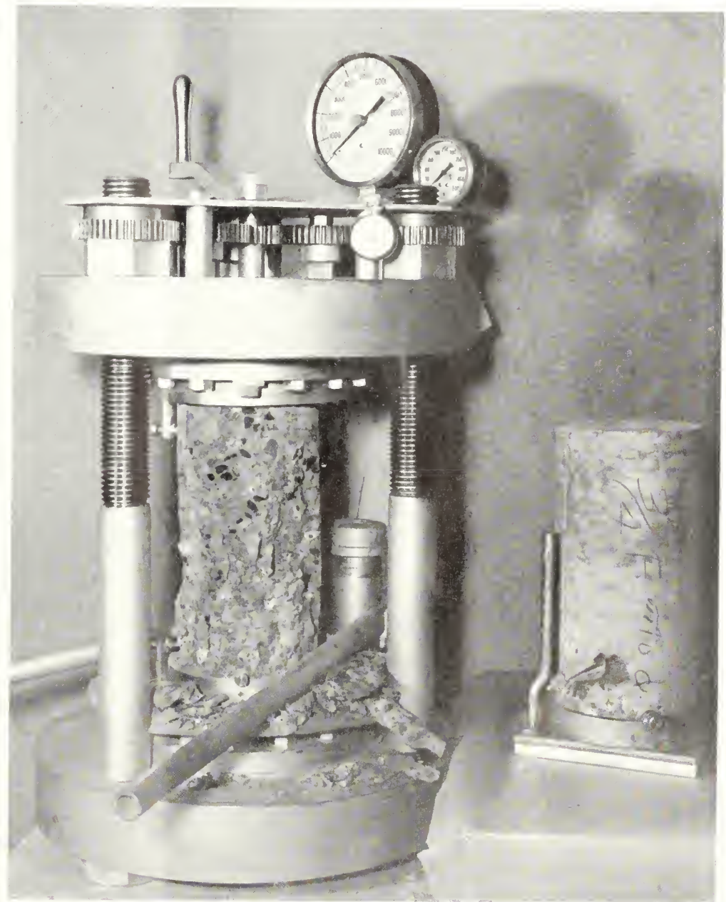
Small size, 300,000-pound capacity hydraulic compression machine
