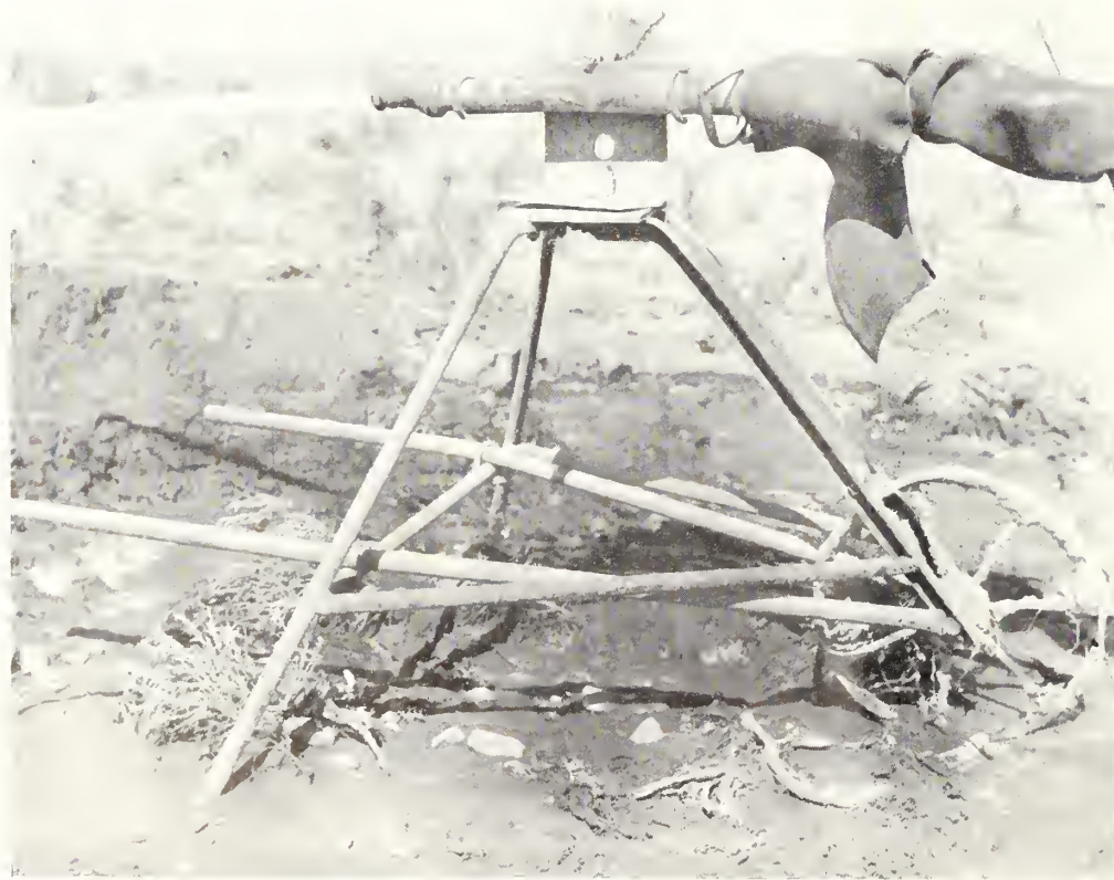
The plate at the top of the wheelbarrow stand permits moving the nozzle sidewise or up and down
