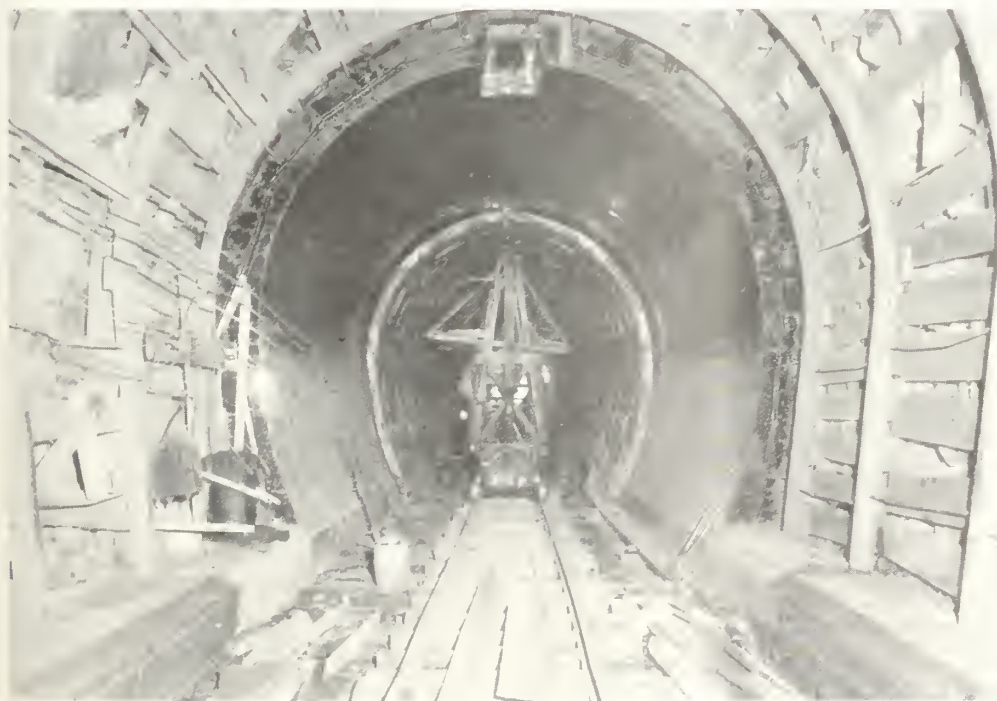
Showing curb construction and arch joint in Tunnel No. 5
