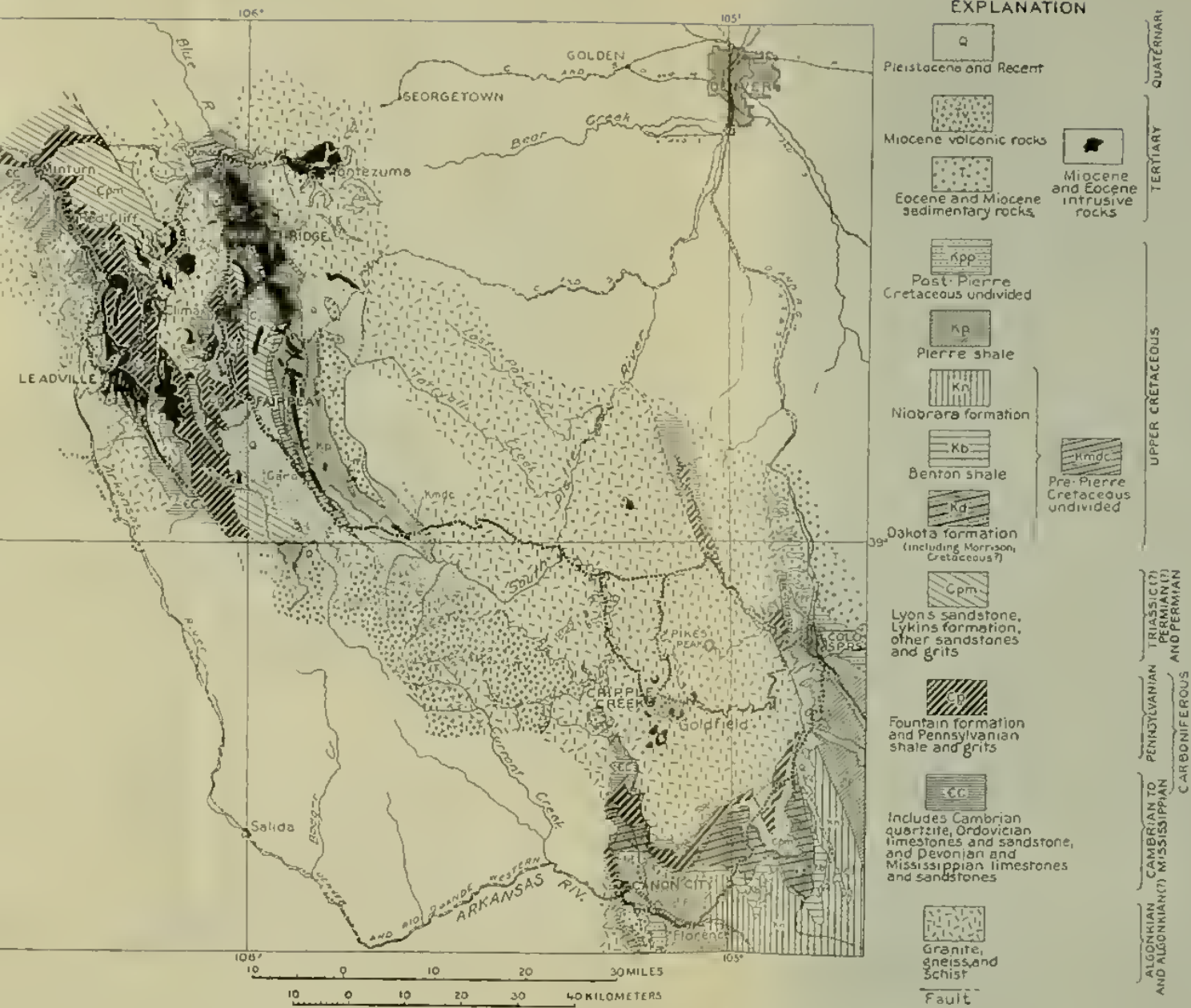
GEOLOGIC MAP SHOWING ROUTE OF EXCURSIONS 2 AND 3 FROM MINTURN TO COLORADO SPRINGS
