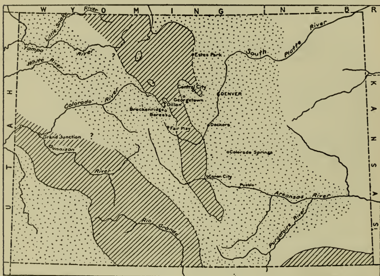
FIGURE 3.—Paleogeography of the Permian rocks of Colorado at beginning of Triassic time. Ruled areas, highlands; stippled areas, Pennsylvanian and Permian rocks. (From Colorado Sci. Soc. Proc., vol. 12, No. 4, fig. 3, 1929)
