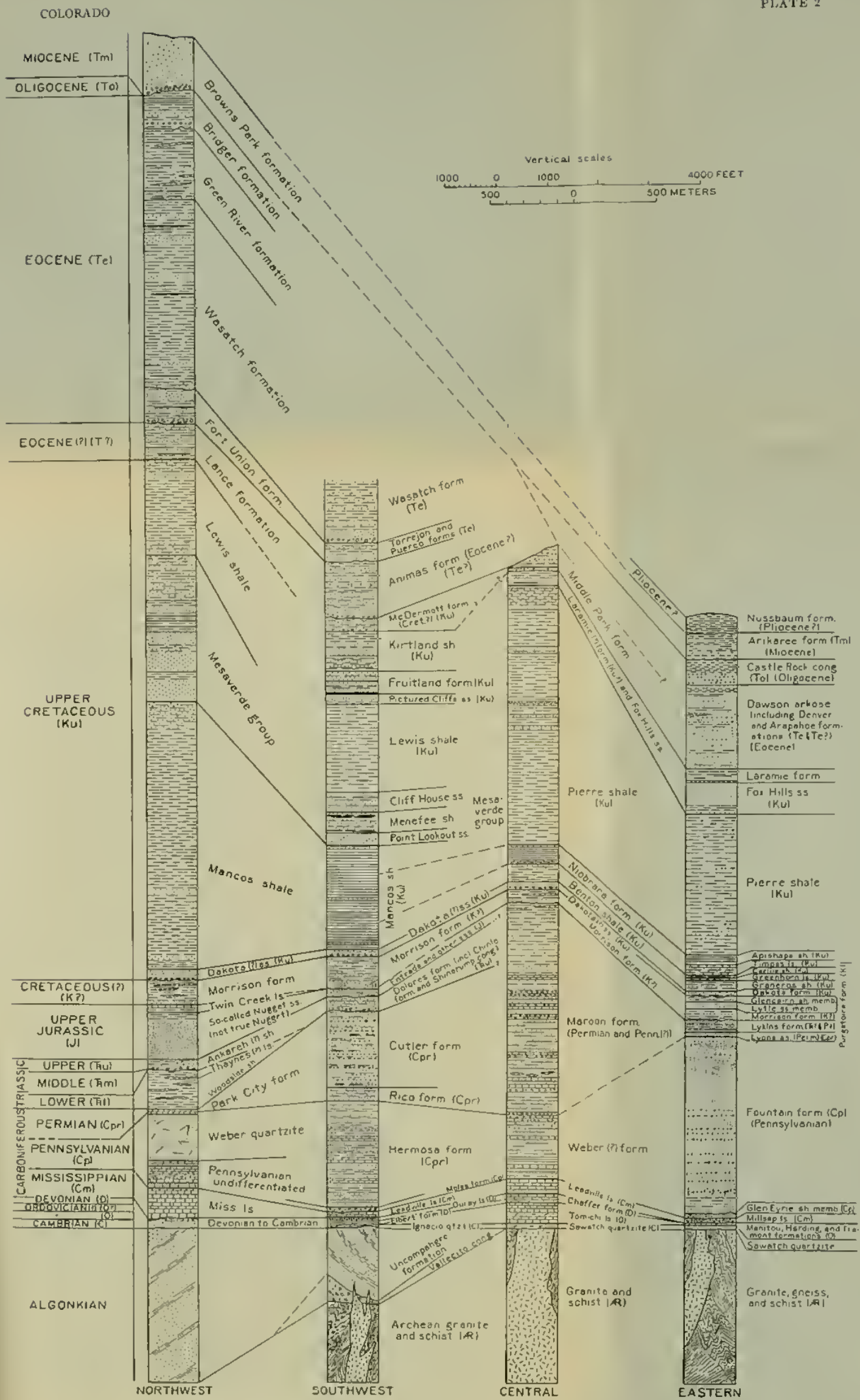
GENERALIZED COLUMNAR SECTIONS FOR COLORADO
