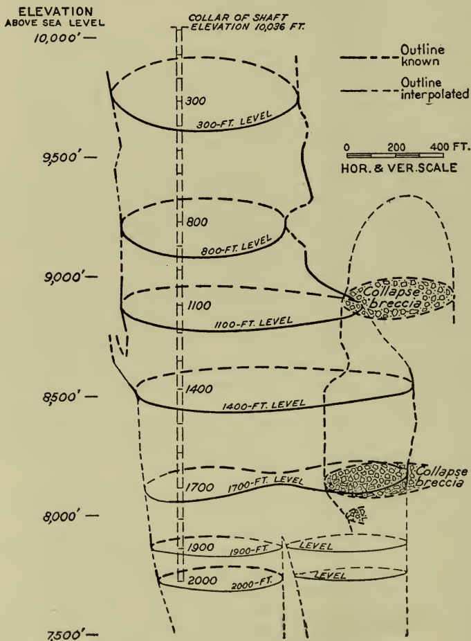
FIGURE 27.—Outline of Cresson pipe of basaltic breccia
