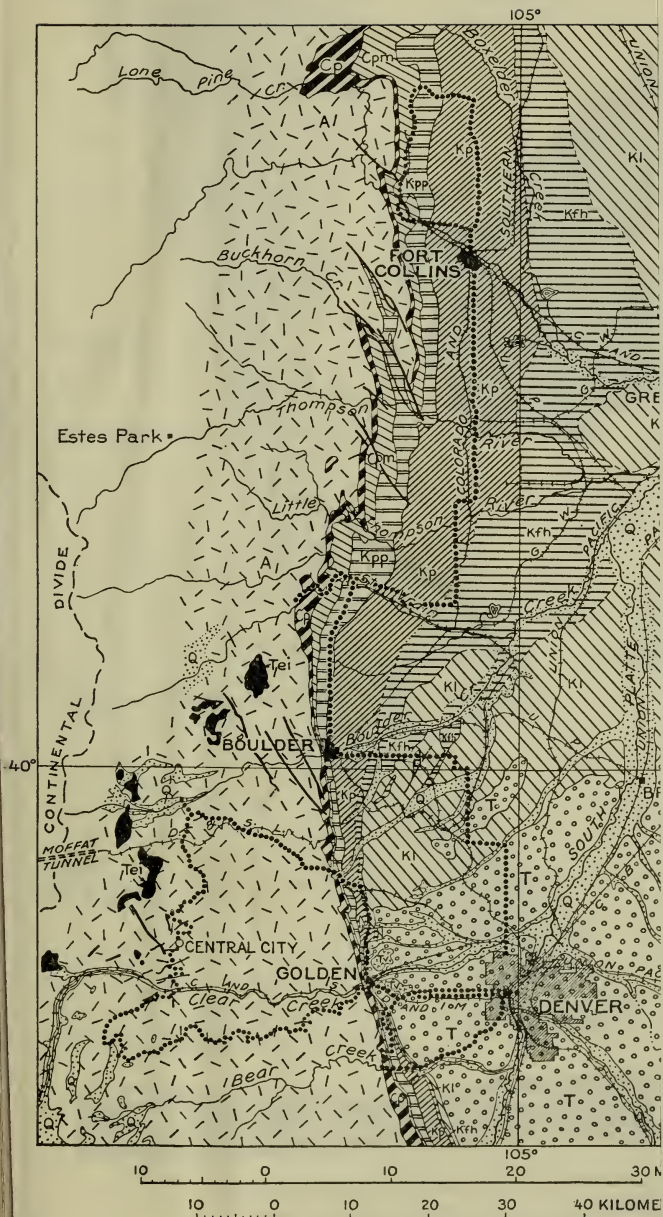
GEOLOGIC MAP SHOWING ROUTE OF EXCURSIONS DENVER AND FORT COLLINS
