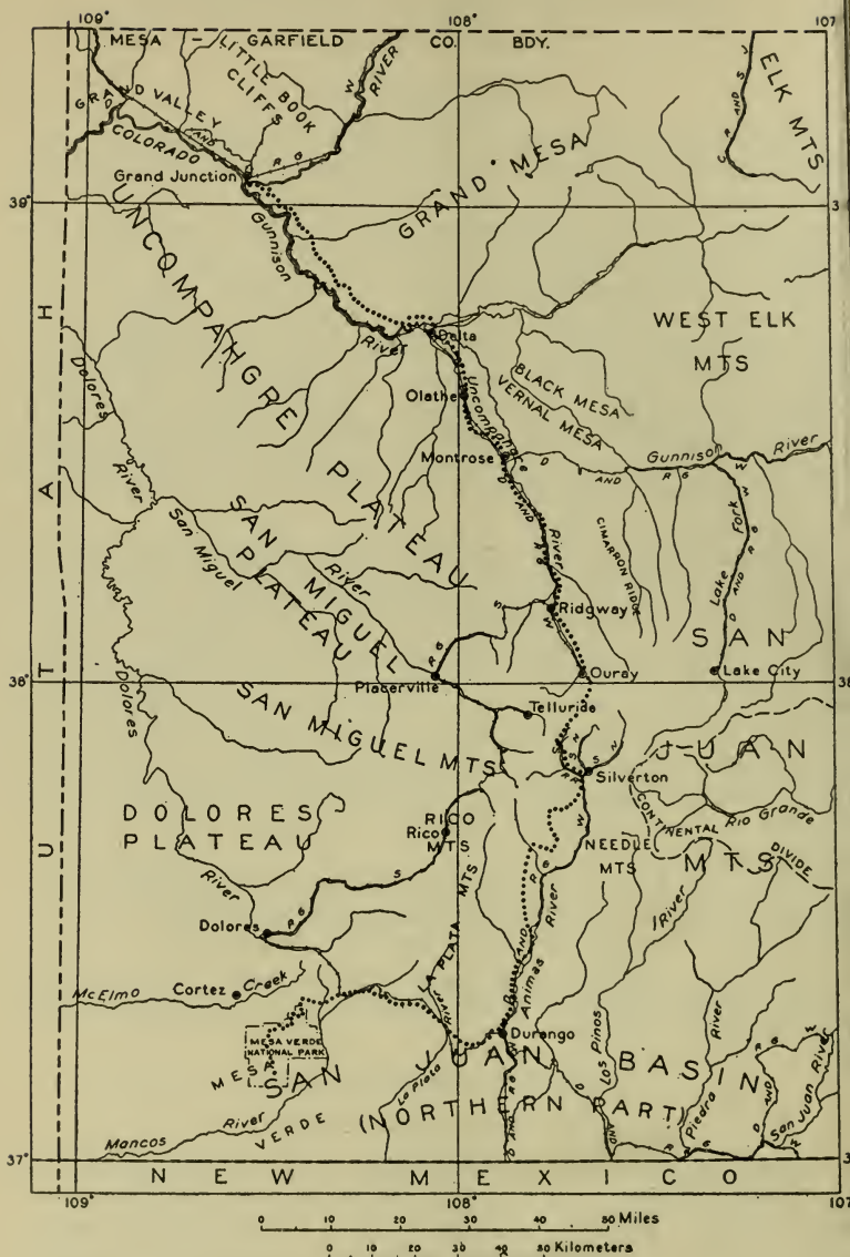
FIGURE 5.—Principal physiographic features of southwestern Colorado
