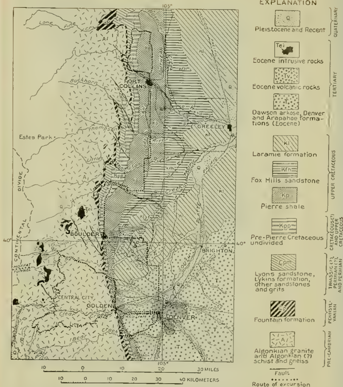
GEOLOGIC MAP SHOWING ROUTE OF EXCURSIONS FROM DENVER AND FORT COLLINS
