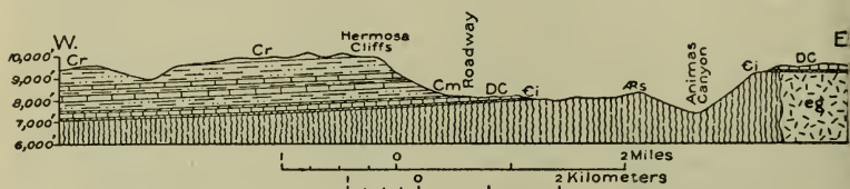
FIGURE 14.—Geologic section from slope south of the Needle Mountains west across the Animas Canyon to the Hermosa Cliffs, about a mile (1.6 kilometers) south of the Ignacio Reservoir. Ars , Archean schist; eg , Eolus granite (Cambrian?); Ci , Ignacio quartzite (Cambrian); DC , Elbert formation (Devonian) Ouray limestone (Devonian), and Leadville limestone (Mississippian); Cm , Molas formation (Pennsylvanian); Ch , Hermosa formation (Pennsylvanian); Cr , Rico formation (Permian). After Cross (10)
