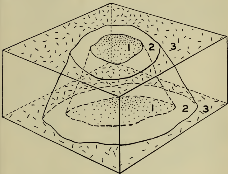
FIGURE 21.—Stereogram showing the general relations of the different zones at Climax. 1, Highly silicified core; 2, ore zone with chiefly moderately silicified granite; 3, slightly altered granite grading into unaltered granite
