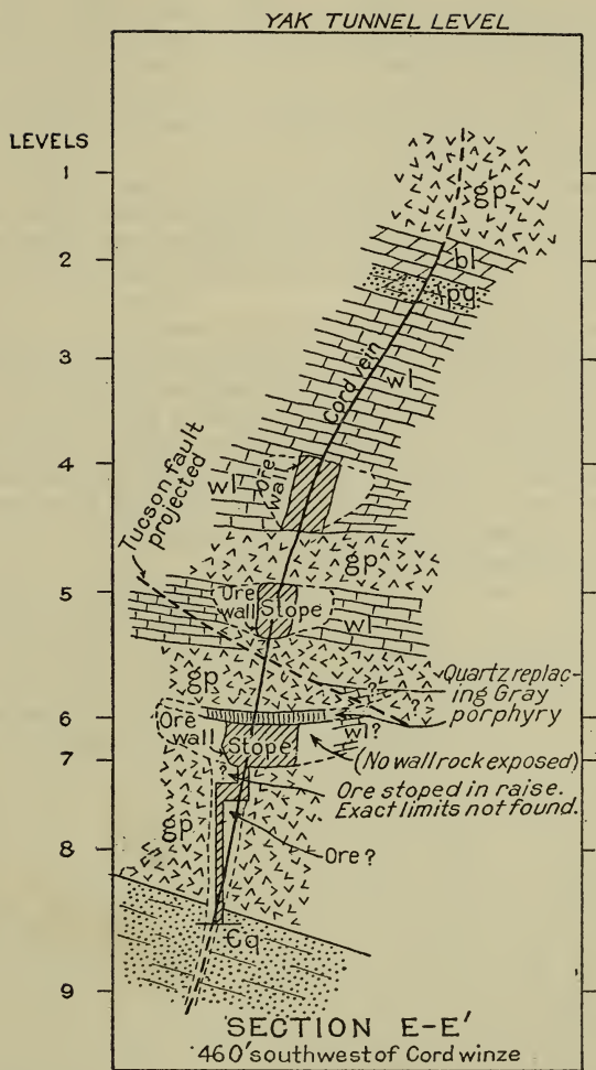
FIGURE 19.—Cross sections of ore bodies along the Cord vein, Iron Hill. gp, Gray porphyry; bl, Leadville ("Blue") limestone; pq, Parting quartzite; wl, "White" limestone; Cq, Cambrian sediments. After Emmons, Irving, and Loughlin (12, fig. 23)
