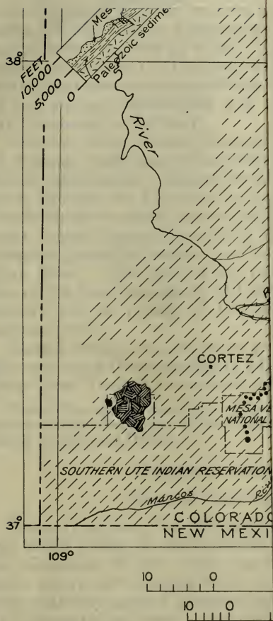
GENERALIZED GEOLOGIC MAP EXCURSION IN SOUTHEASTERN COLORADO
