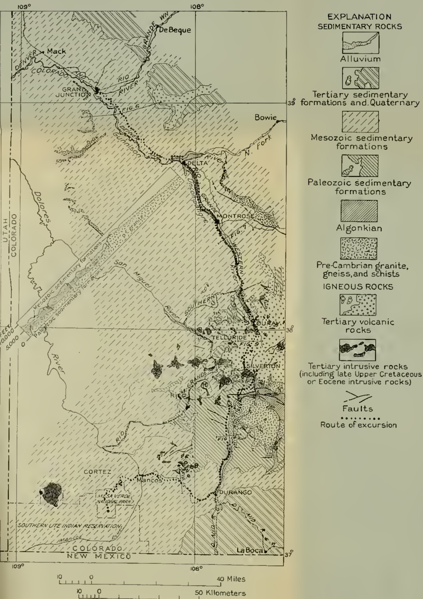
GENERALIZED GEOLOGIC MAP AND SECTION SHOWING ROUTE OF EXCURSION IN SOUTHWESTERN COLORADO
