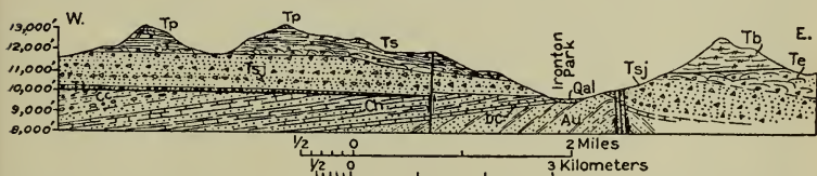
FIGURE 9.—Geologic section across Ironton Park. After Cross, Howe, and Spencer (13), with additions. Au, Uncompahgre formation; DC, Devonian (Ouray) and Mississippian (Leadville) limestones; Ch, Hermosa formation; Cc, Cutler formation; Tt, Telluride conglomerate; Tsj, San Juan tuff; Ts, undivided Silverton volcanic series; Te, Eureka rhyolite of Silverton volcanic series; Tb, Burns latite of Silverton volcanic series; Tp, Potosi volcanic series; Qal, alluvium
