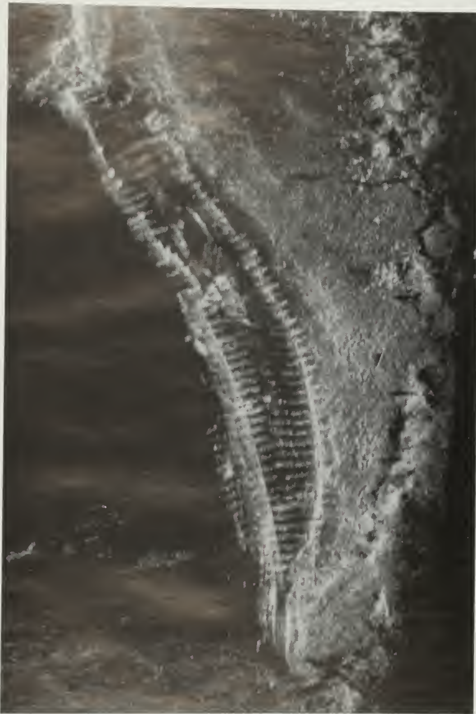
Figure 16. Sonograph of E. C. Waters' site showing hull features and surrounding bottom areas. Curvature is the result of the survey vessel's path. E. C. Waters' bow is at the bottom of the image.
