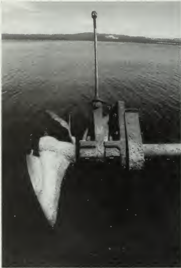
Figure 5.41. View north, starboard side of adjustable stern bearing assembly (center) and propeller (left). NPS photo by John Brooks.
