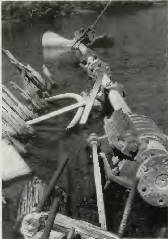
Figure 5.34. View west of E. C. Waters' propulsion system. The engine bed is in the foreground, the thrust bearing is in the middle foreground and the propeller shaft and the propeller is in the background. NPS photo by John Brooks.
