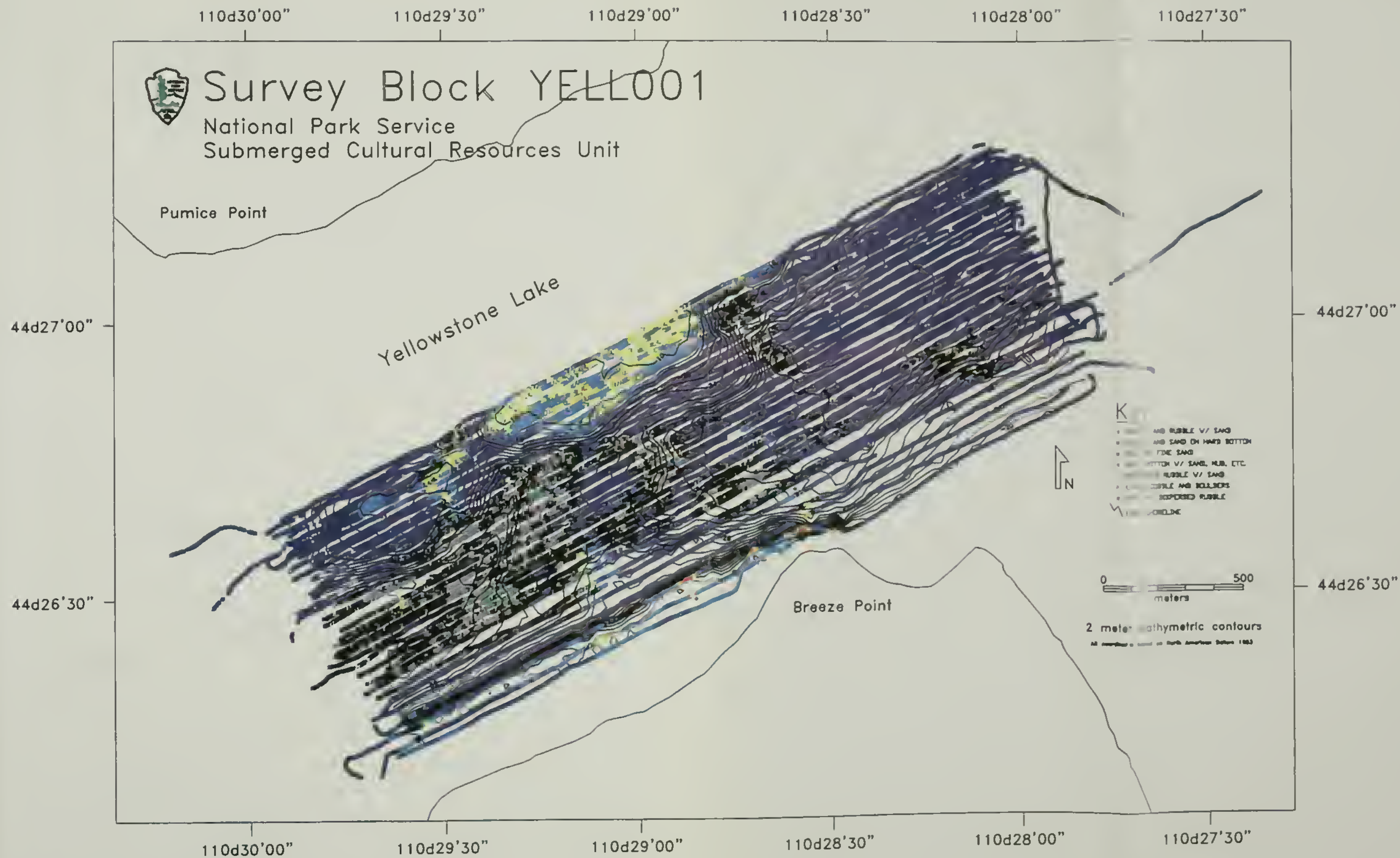
Figure 8. Raw RoxAnn data, survey block YELL001.
