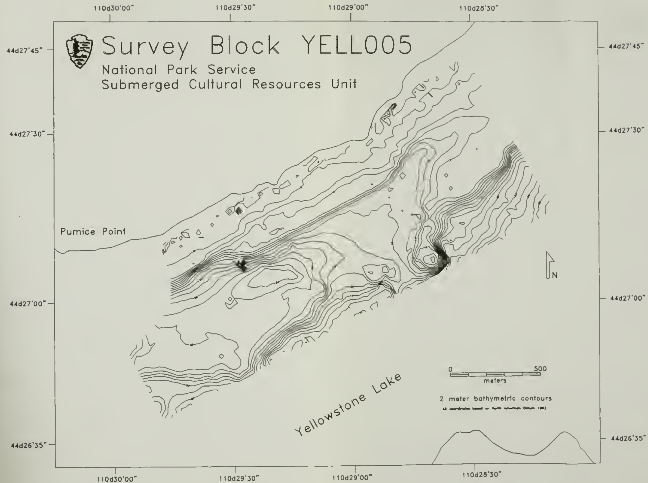
Figure 19. Two meter bathymetric contours, survey block YELL005.
