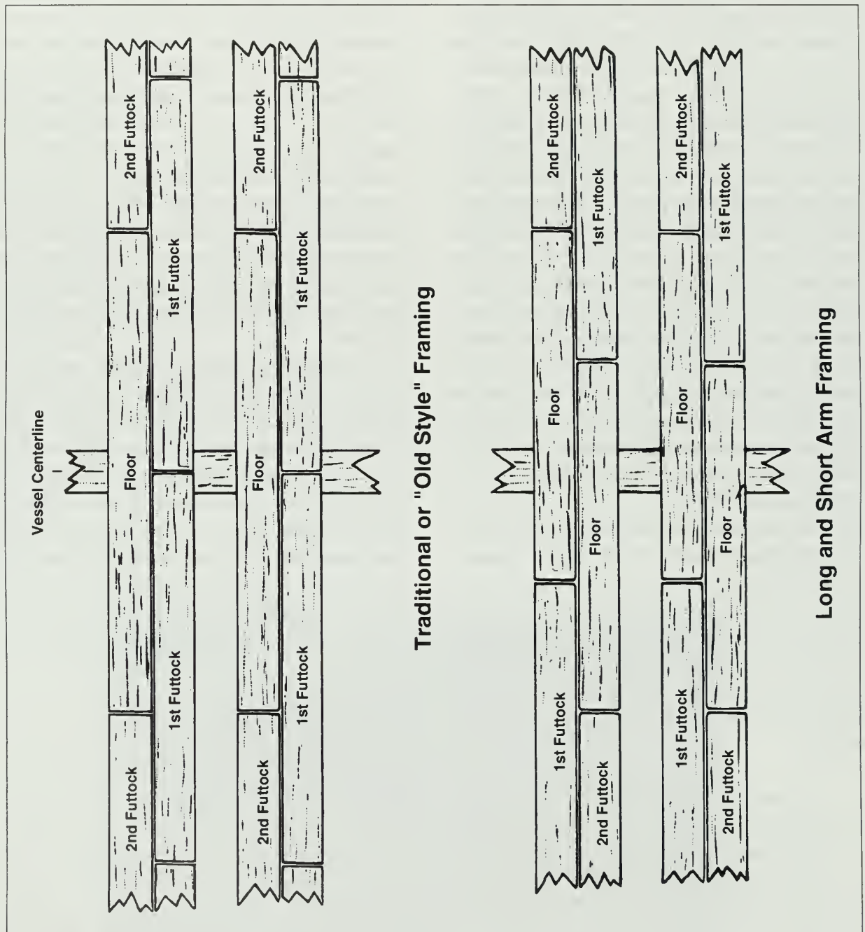
Figure 5.30. Different styles of framing a wooden vessel. Drawing by Matt Russell.
