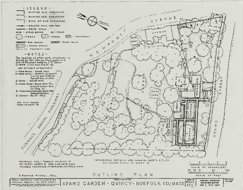
HABS DRAWING OF ADAMS SITE, 1936.
