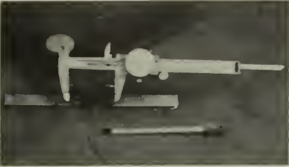
A custom made gauge system. The machinist's calipers have been modified by putting a small hole in each jaw. The holes fit over the stainless steel cones of the gauge points during reading. One set of calipers is used to read numerous gauge points at one site. Caliper accuracy is checked by taking readings on stainless steel rods of known length.
