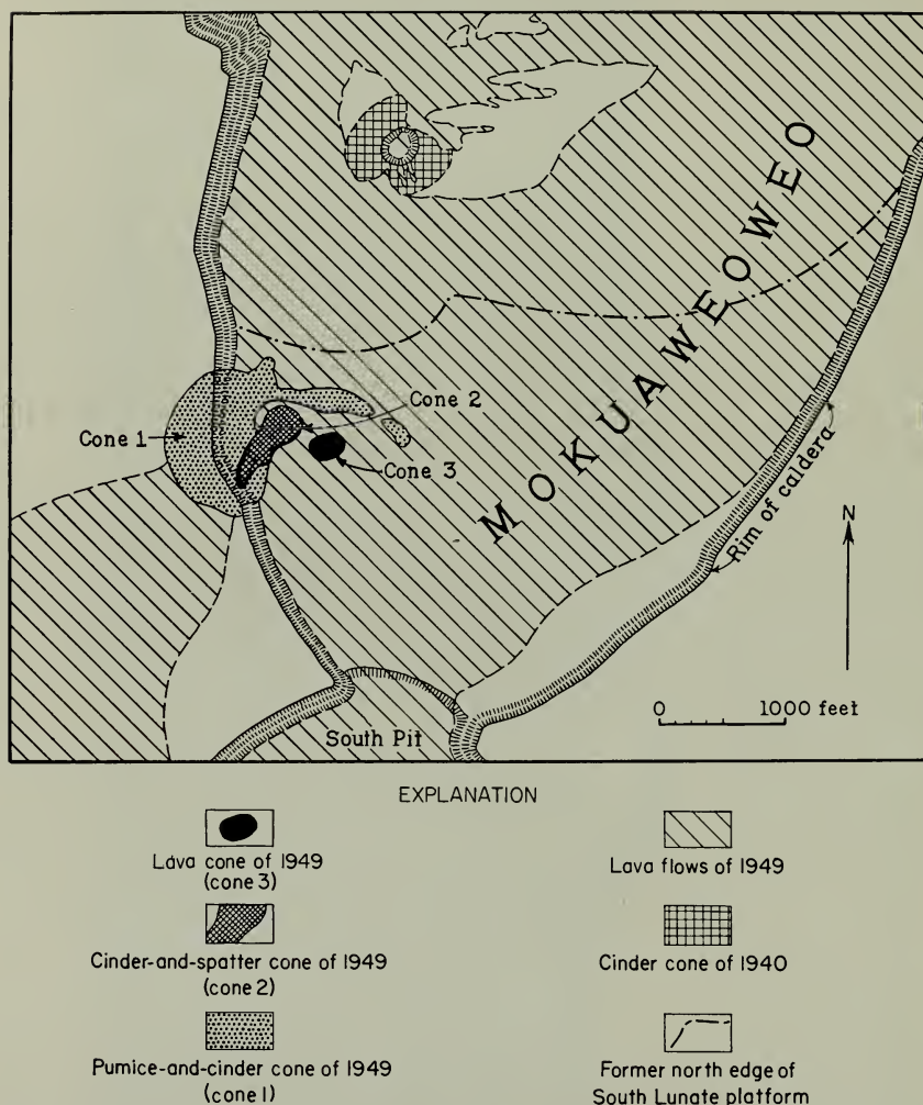
FIGURE 9.—Sketch map of the southern part of Mokuaweoweo caldera, Mauna Loa, Hawaii, on June 3, at the end of the 1949 eruption.
