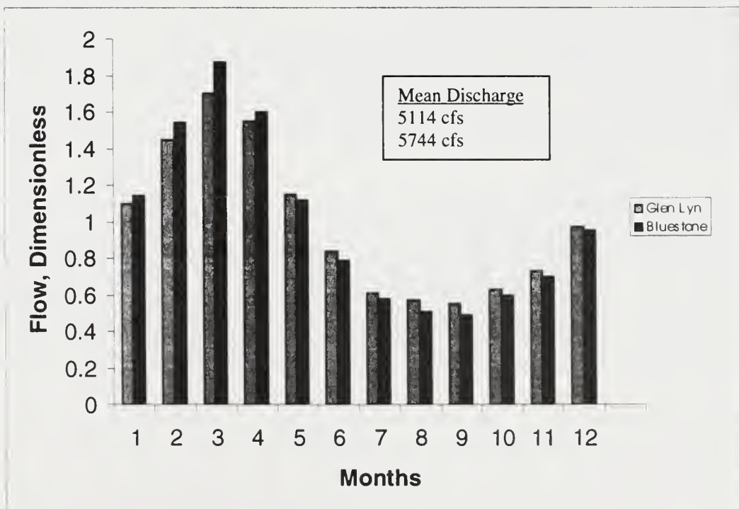
Figure 10. Mean monthly flows for the New River, 1949 – 1983, after completion of Bluestone Dam. After Flug (1987).
