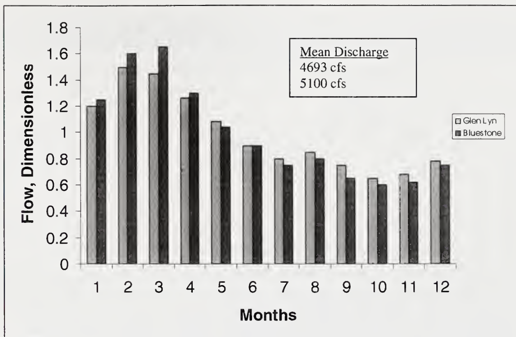
Figure 11. Mean monthly flows for the New River, 1939-1948, after completion of Claytor Dam, but before completion of Bluestone Dam. After Flug (1987).
