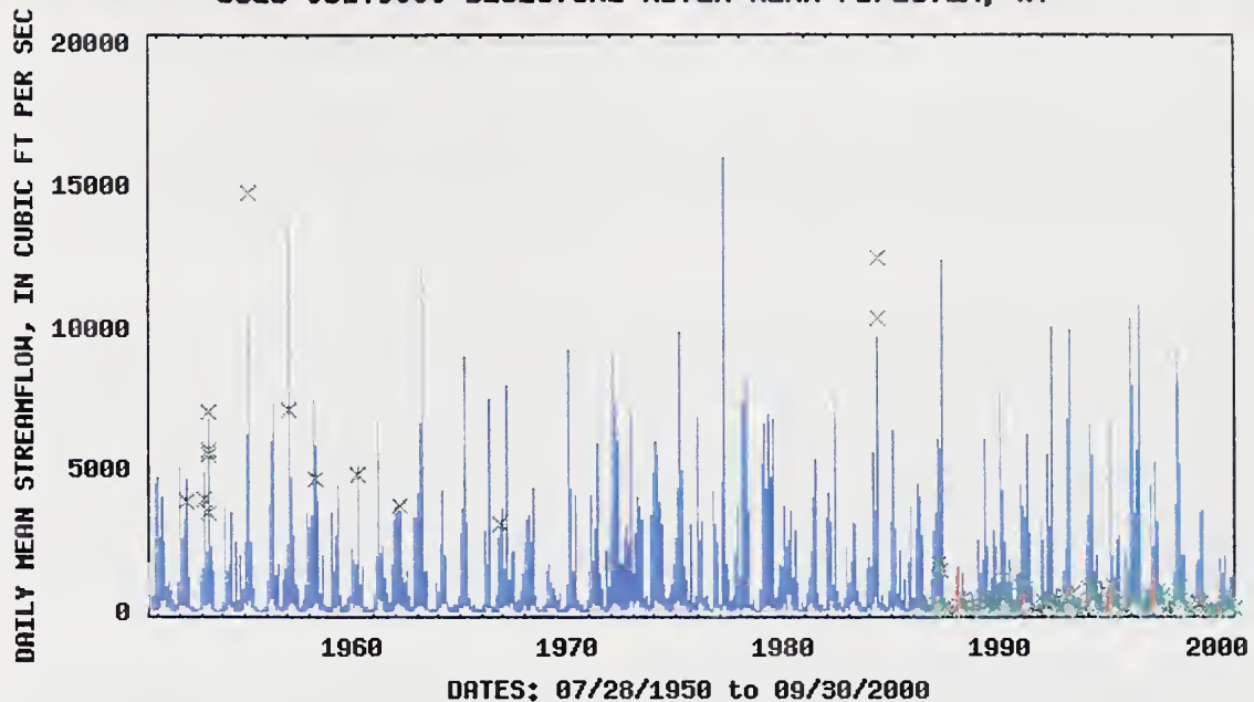
Figure 15. Daily streamflow values for Bluestone River near Pipestem, WV.
