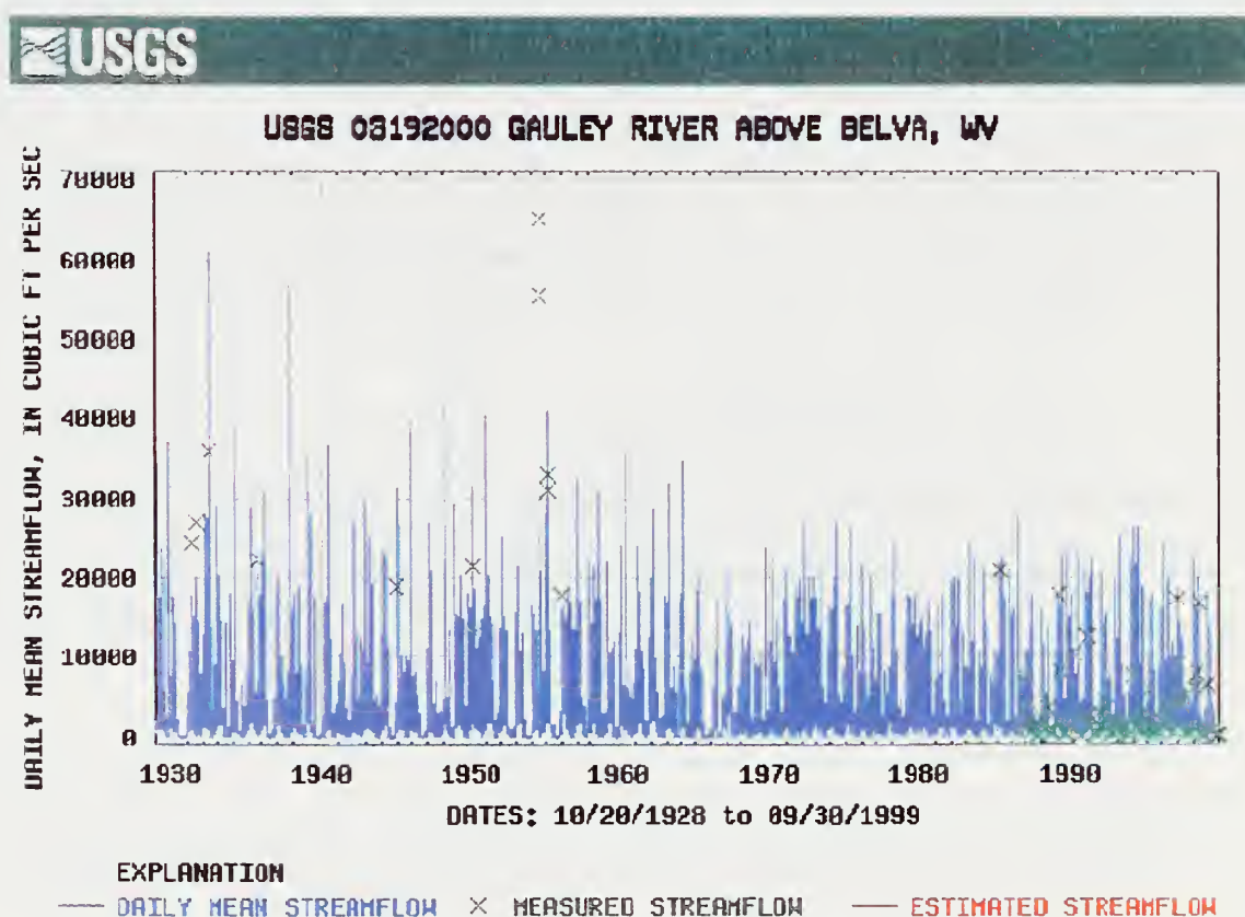
Figure 14. Daily streamflow values for Gauley River above Belva, WV (03192000). After > http://www.usgs.gov > .
