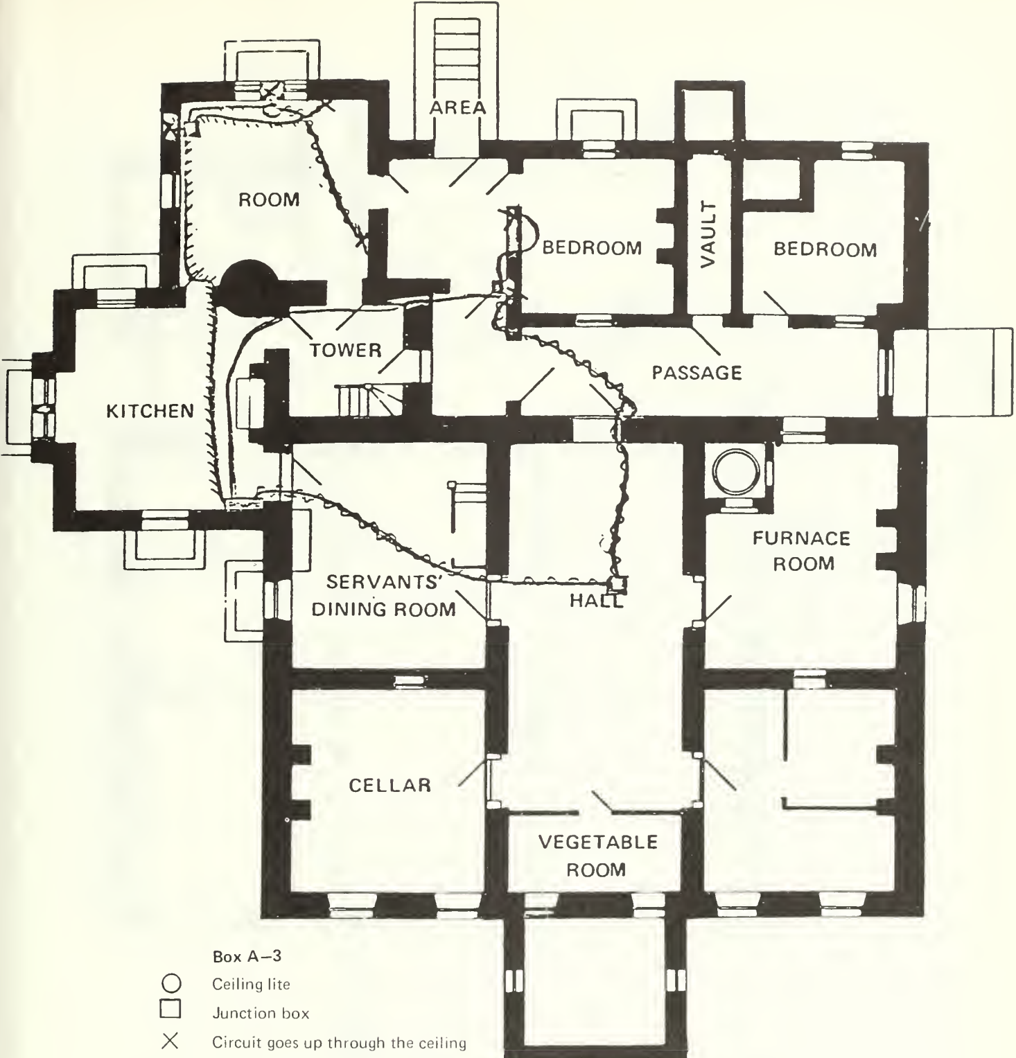
Basement Plan
