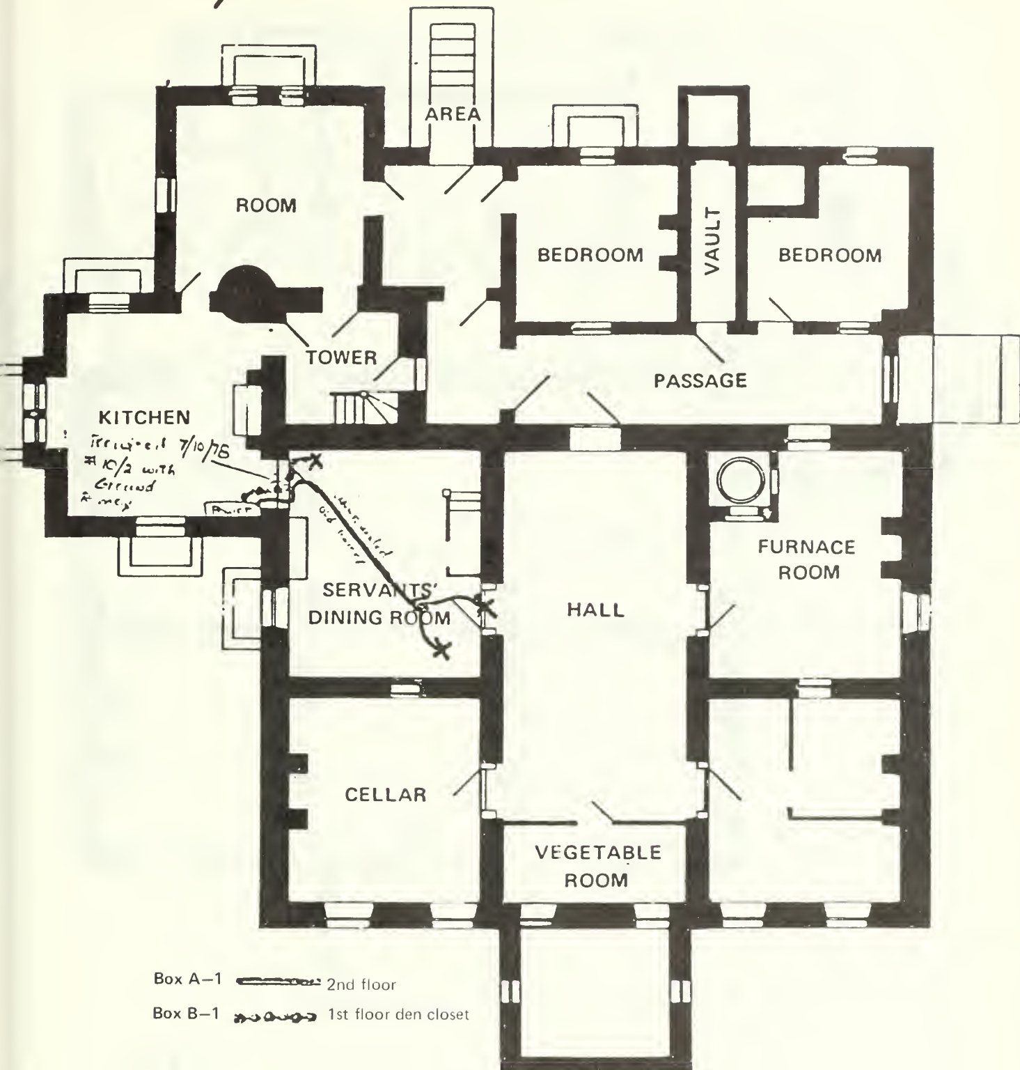
Basement Plan
