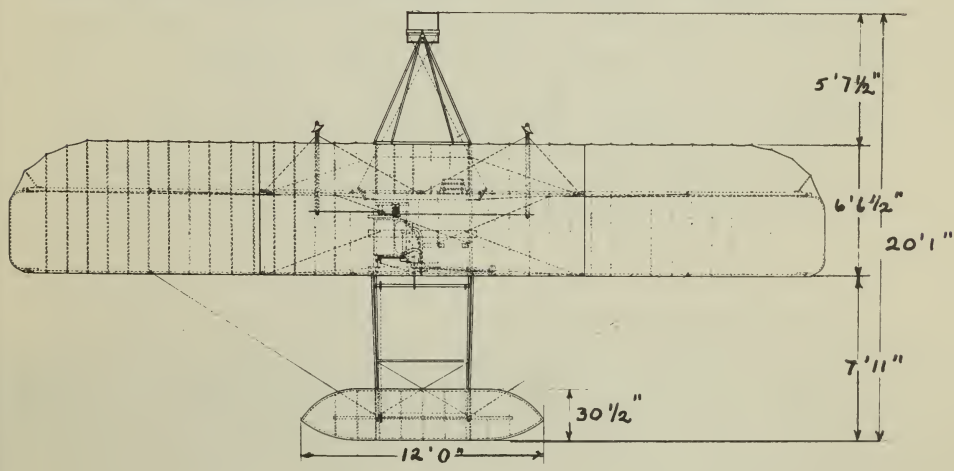
Opposite page and below: Plans of the Wright Brothers 1903 plane and photographs of front and side views of the plane. Plans, courtesy, Smithsonian Institution.
