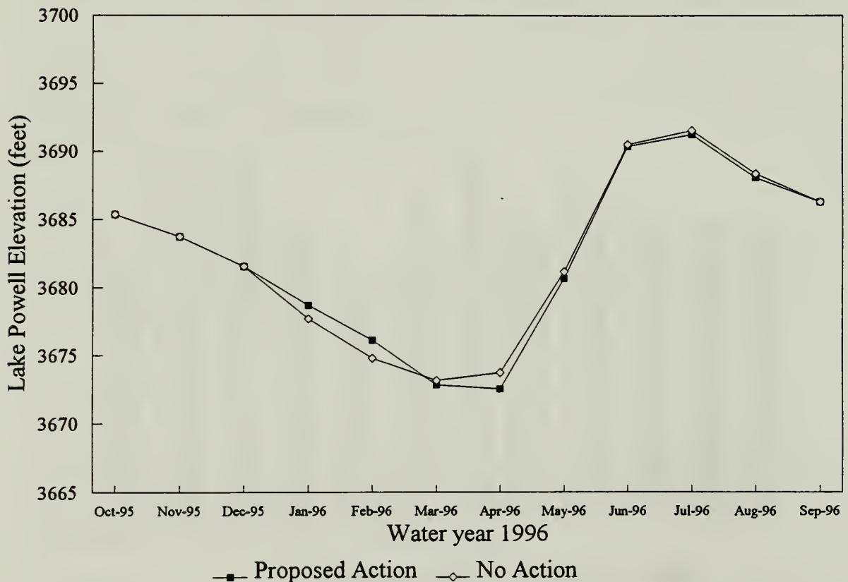
Figure 5.—Comparison of Lake Powell elevations throughout the year and between the No Action and Proposed Action Alternatives. The difference in lake elevations between the two alternatives is greatest at the end of February and April, but only by 1.3 and 1.0 feet, respectively.
