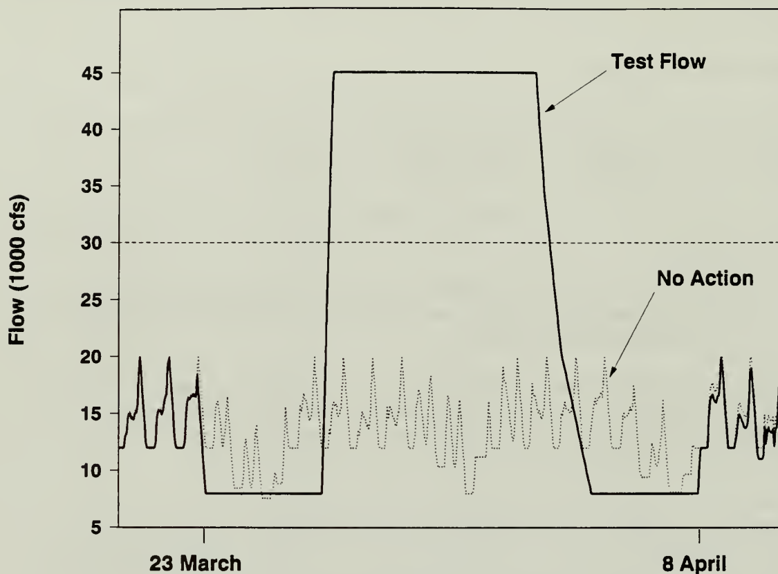
Figure 2.—Hydrograph of beach/habitat-building test flow.
