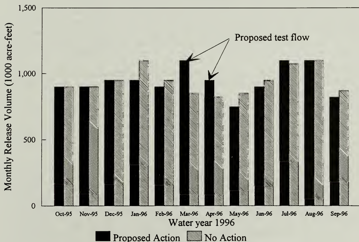
Figure 4.—Comparison of monthly release volumes under the No Action and Proposed Action Alternatives. The greatest difference would occur in January, March, and April; no difference would occur during October through December.
