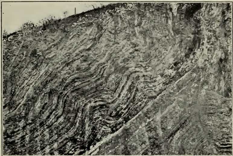
A. GRAY CHERTY SHALE IN LOWER MEMBER OF MODELO FORMATION OF SANTA MONICA MOUNTAINS
