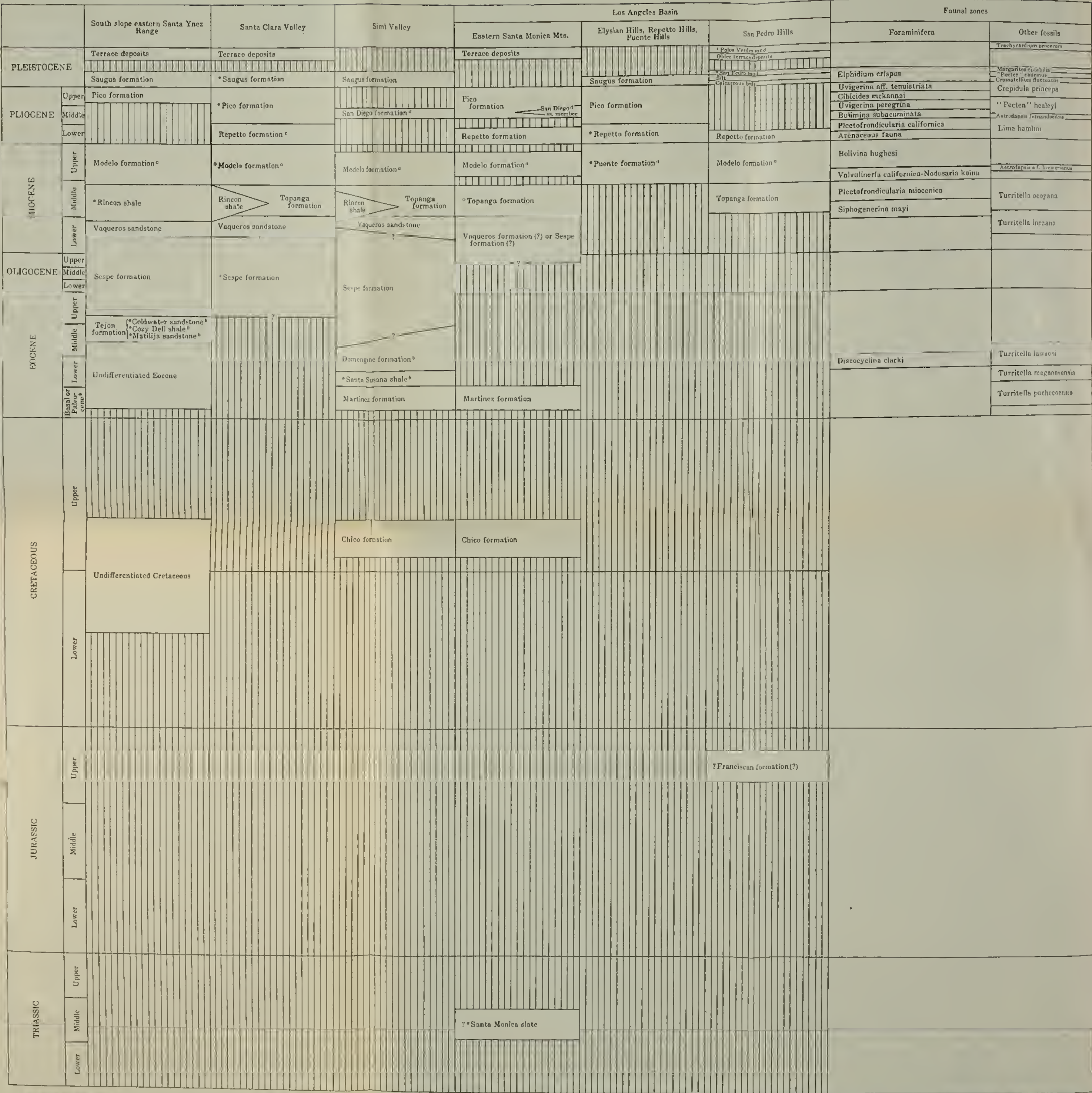
SEDIMENTARY DEPOSITS IN AREAS COVERED BY EXCURSIONS IN COASTAL REGION OF SOUTHERN CALIFORNIA
