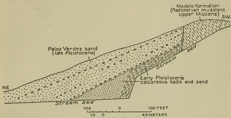
FIGURE 5.—Section exposed in fifth ravine west of WALTERIA, at north edge of San Pedro Hills
