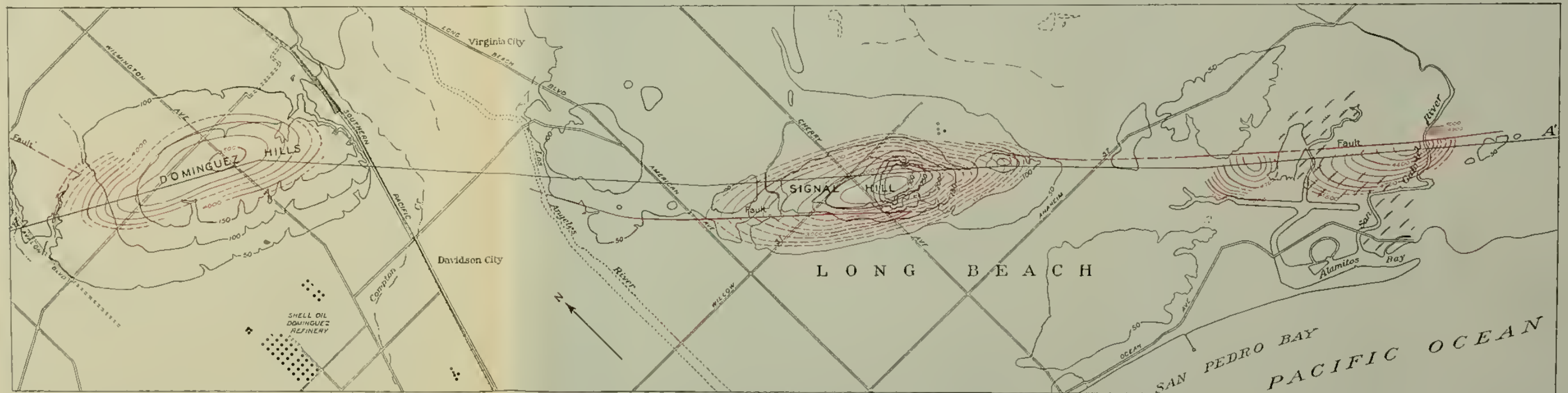
TOPOGRAPHIC MAP WITH STRUCTURE CONTOURS AND STRUCTURE SECTION OF THE DOMINGUEZ, LONG BEACH, AND SEAL BEACH OIL FIELD
