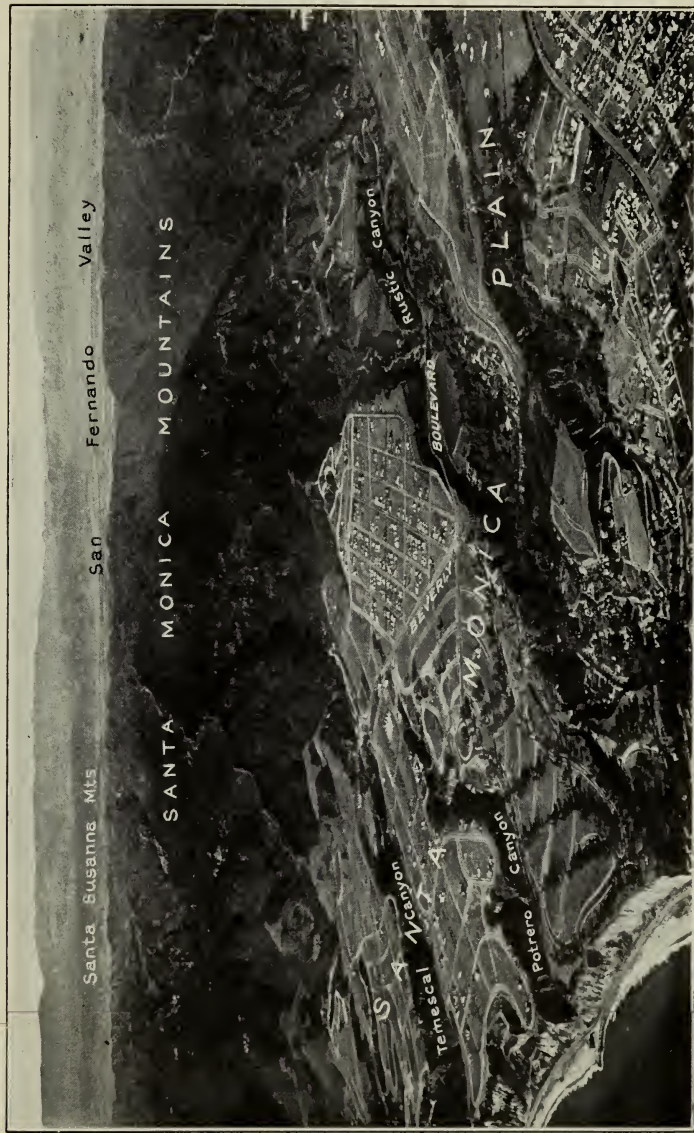
AIRPLANE VIEW OF SANTA MONICA MOUNTAINS
