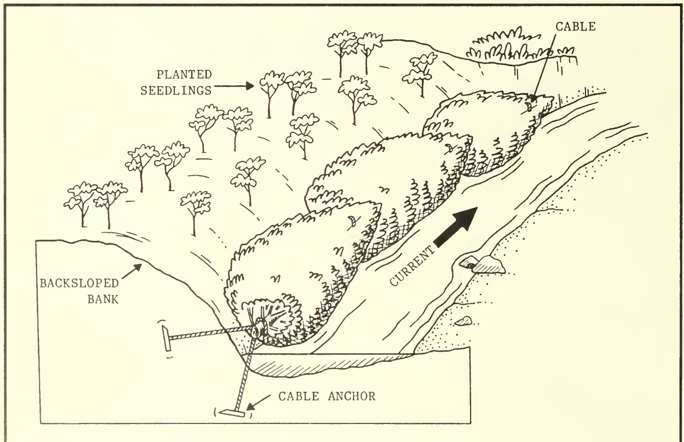
Schematic representation of cedar tree revetment shows anchoring method, orientation relative to current, and revegetation of back-sloped bank and riparian buffer.
