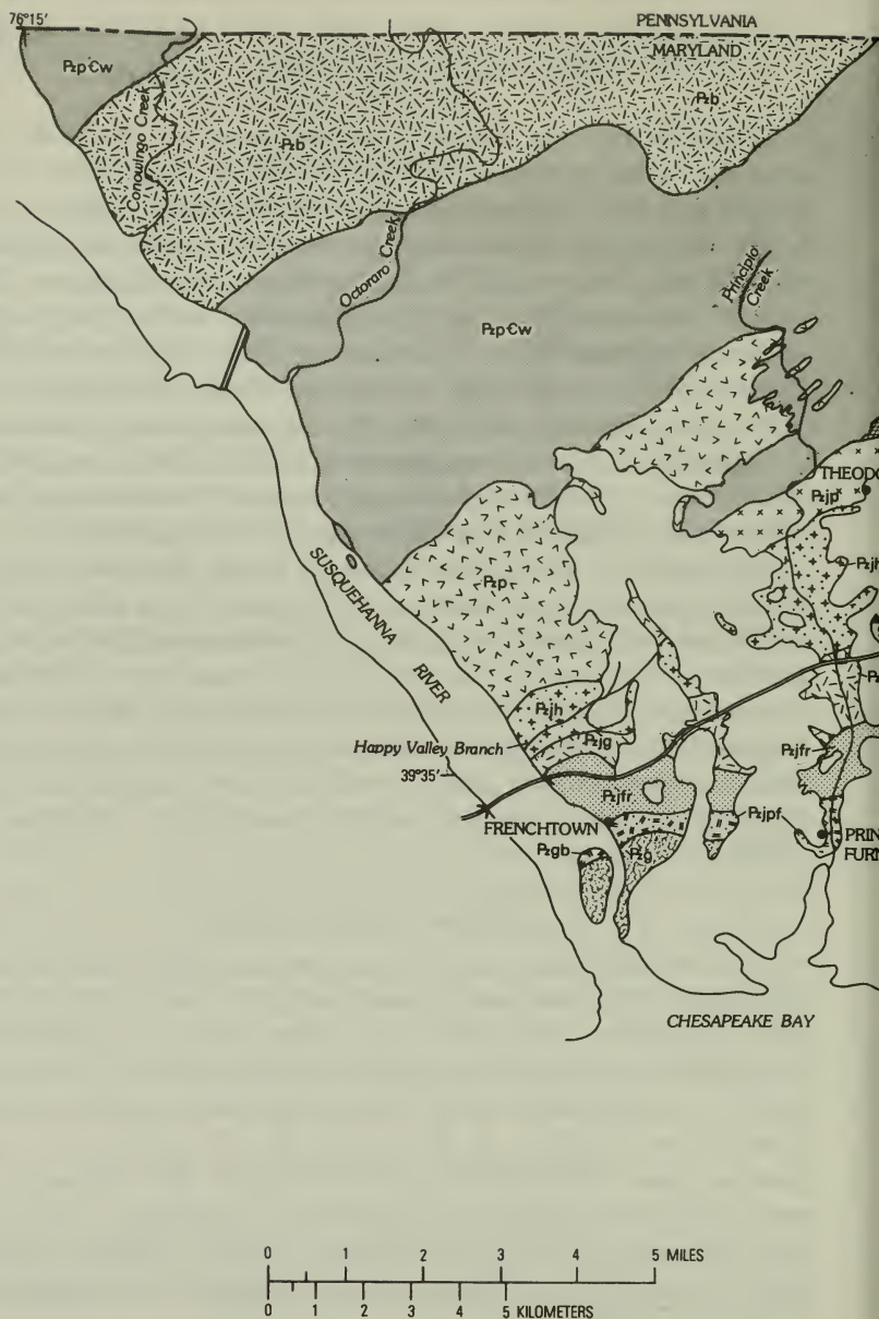
FIGURE 3.—Generalized geologic map of Cecil County, Md., showing members of the James Run Formation.
