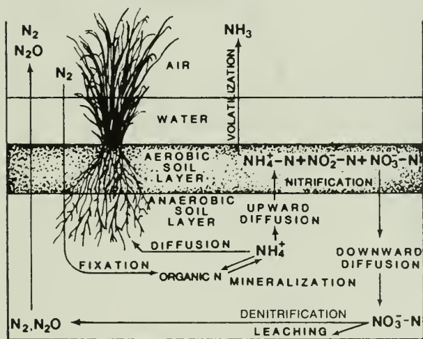
Figure 63. A schematic outline of the redox zones in a submerged soil showing some of the N transformations (Copyright. Reprinted from "Nitrogen in Agricultural Soils," 1982, with permission of the American Society of Agronomy). The aerobids layer has been drawn thick for clarity. In reality, it is seldom over 1-2 mm in flooded marshes.
