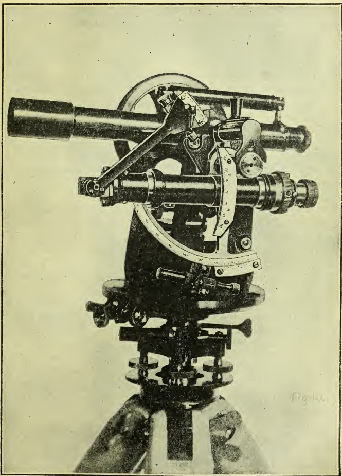
FIG. 10.—Direct sighting through the auxiliary telescope, with the mirror swung to a central position, and showing the striding level on the latitude axis.
