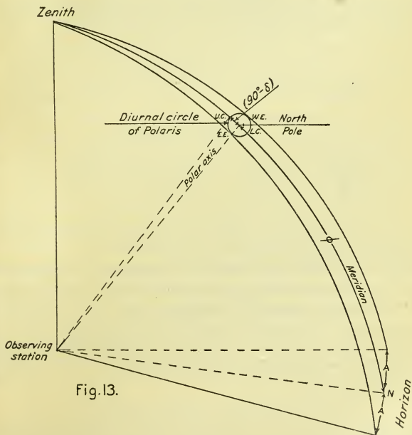
the meridian and vertical planes tangent to the diurnal circle of Polaris as viewed from outside of the celestial sphere.
