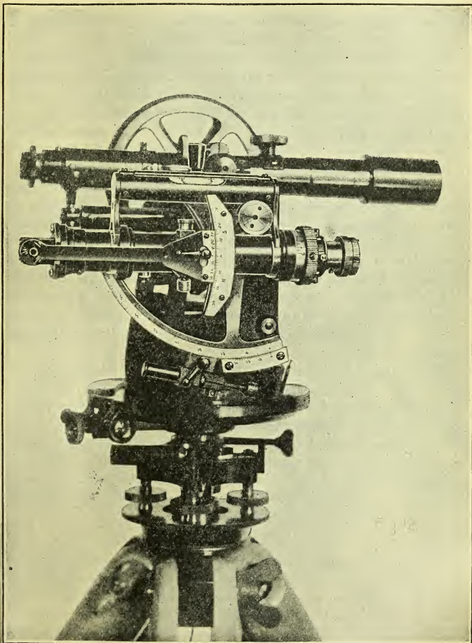
FIG. 12.—The striding level on the auxiliary telescope.
