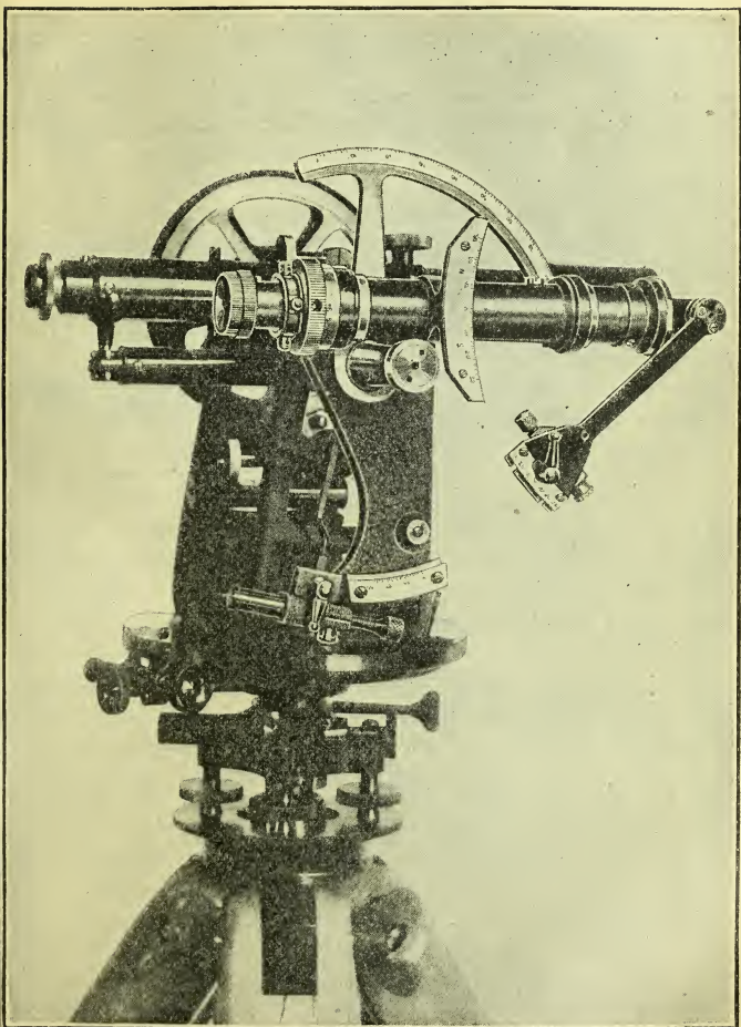
FIG. 11.—The auxiliary telescope in reversed position.
