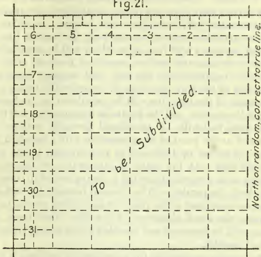
STANDARD PARALLEL
