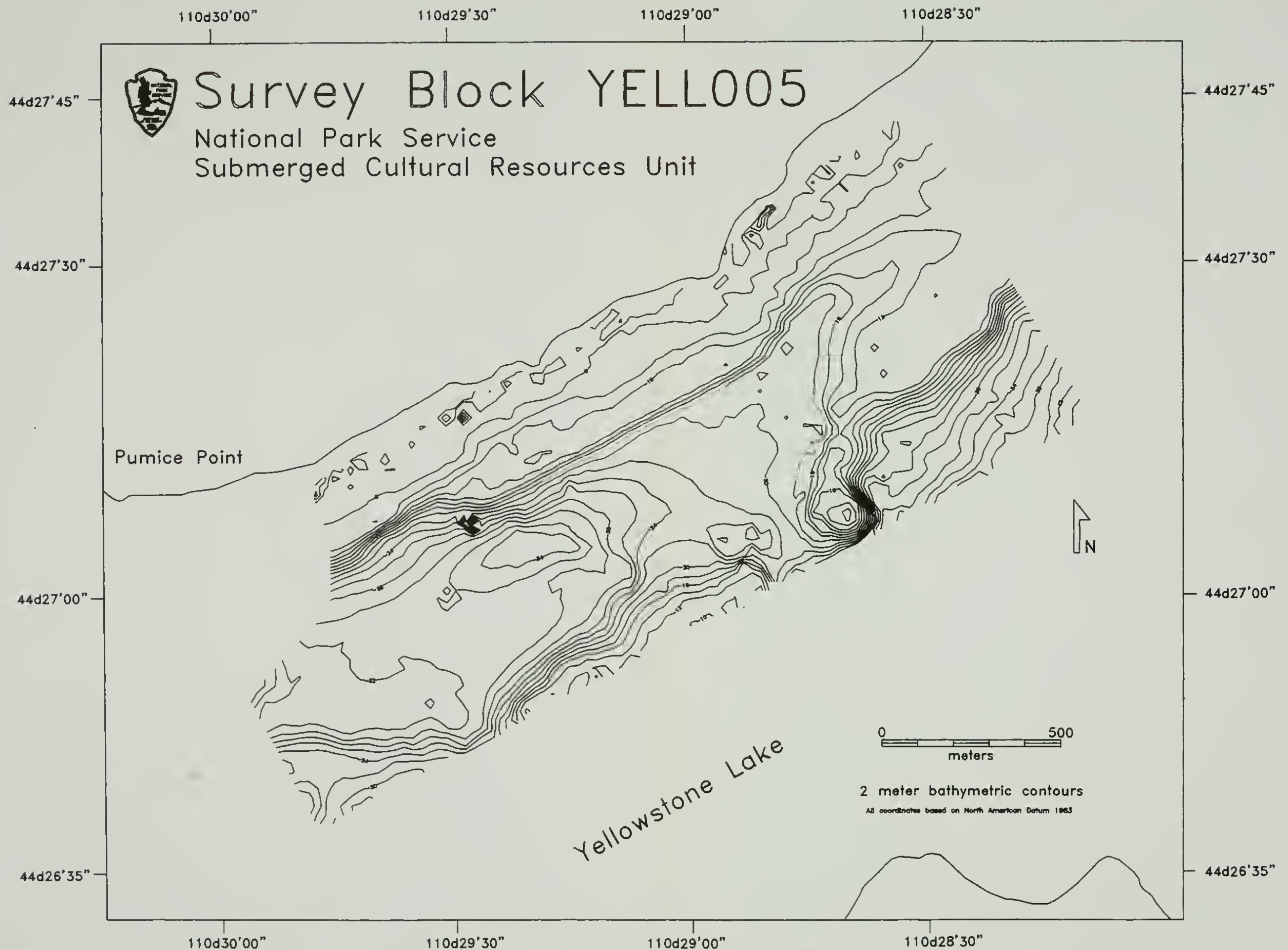
Figure 19. Two meter bathymetric contours, survey block YELL005.
