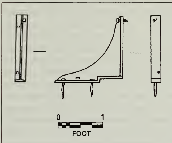
Figure 5.32. Side and end views of boiler saddle. Drawing by Jim Bradford.
