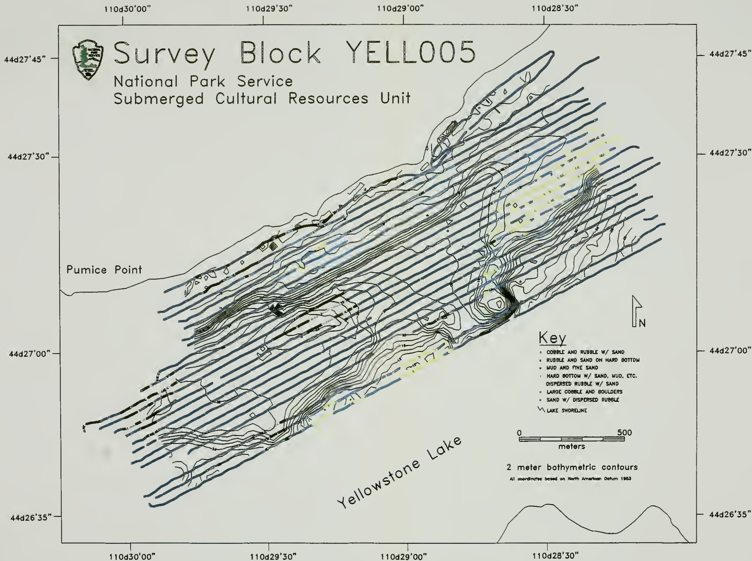
Figure 9. Raw RoxAnn data, survey block YELL005.
