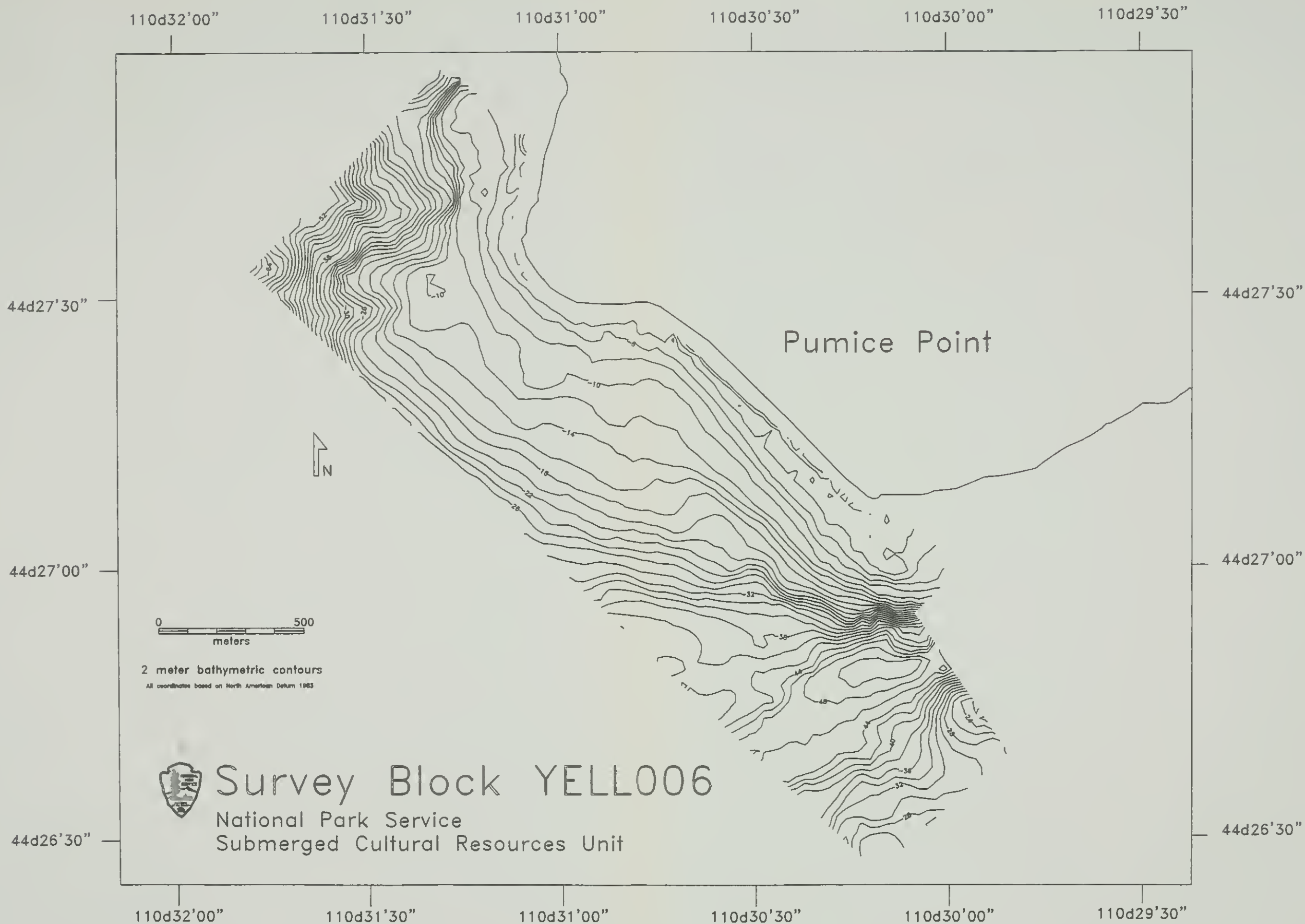
Figure 20. Two meter bathymetric contours, survey block YELL006.
