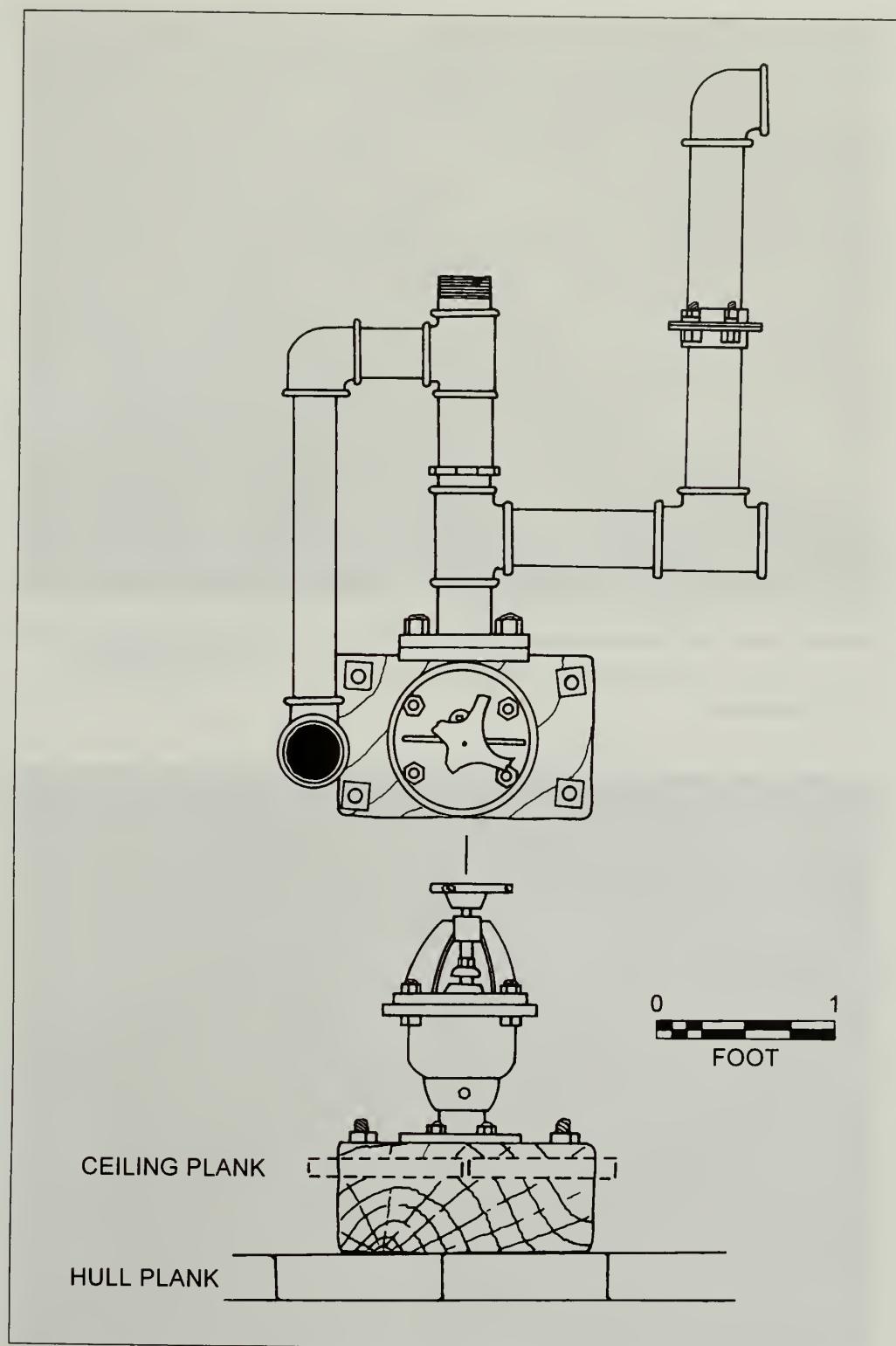
Figure 5.43. Plan view and aft elevation of the globe valve with intake pipes. Drawing by Jim Bradford.
