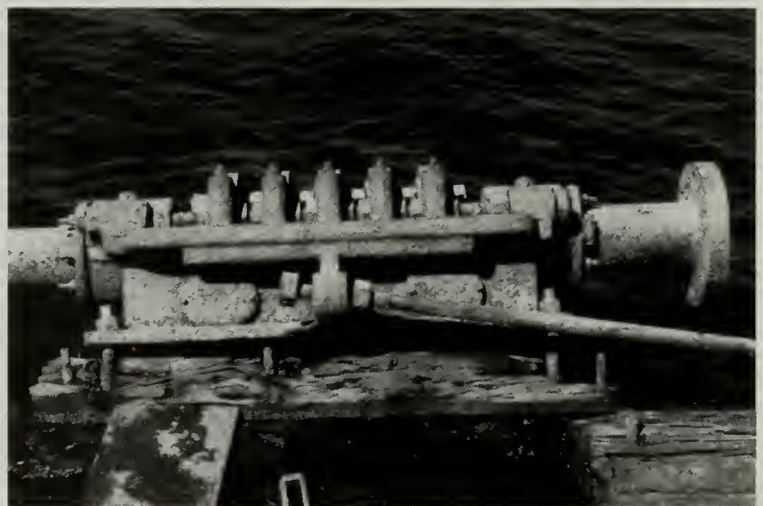
Figure 5.35. Starboard side of thrust bearing. NPS photo by Jim Bradford.
