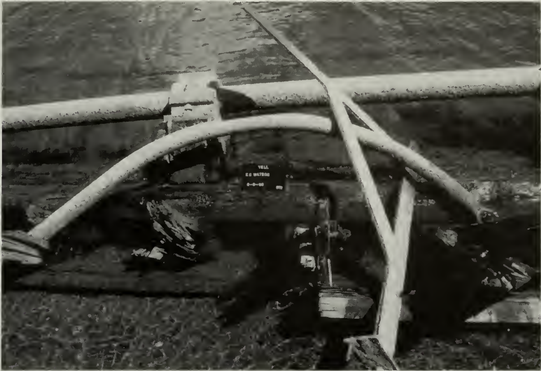
Figure 5.49. Davit (left) and support bracket (right) within E. C. Waters' wreckage. NPS photo by Brett Seymour.
