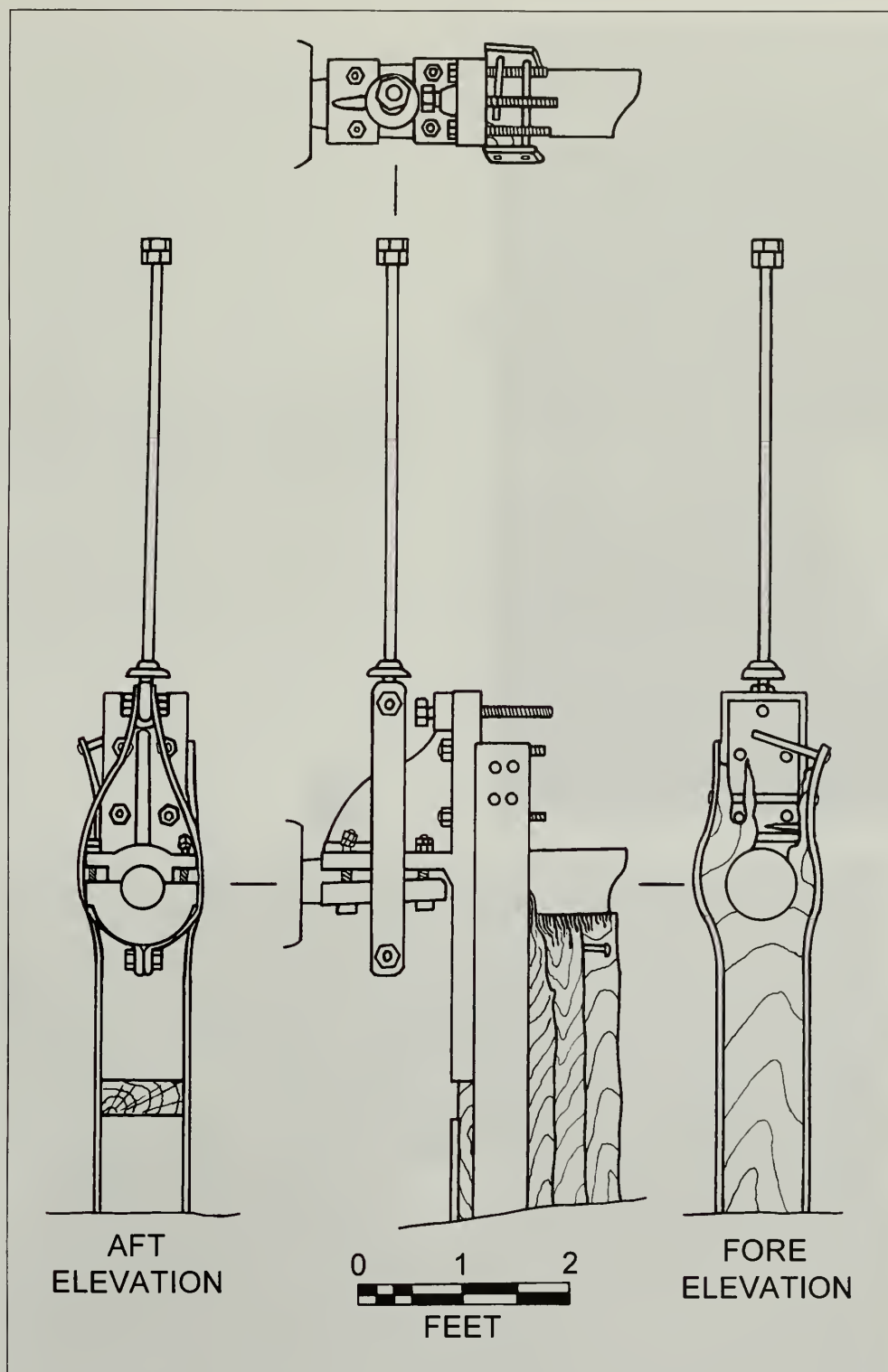
Figure 5.40. Plan, starboard elevation, fore and aft views of adjustable stern bearing assembly. Drawing by Jim Bradford.
