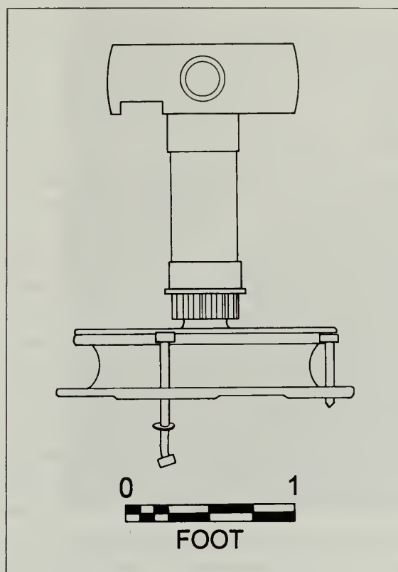
Figure 5.46. Scale drawing of E. C. Waters' capstan. Drawing by Matt Russell.
