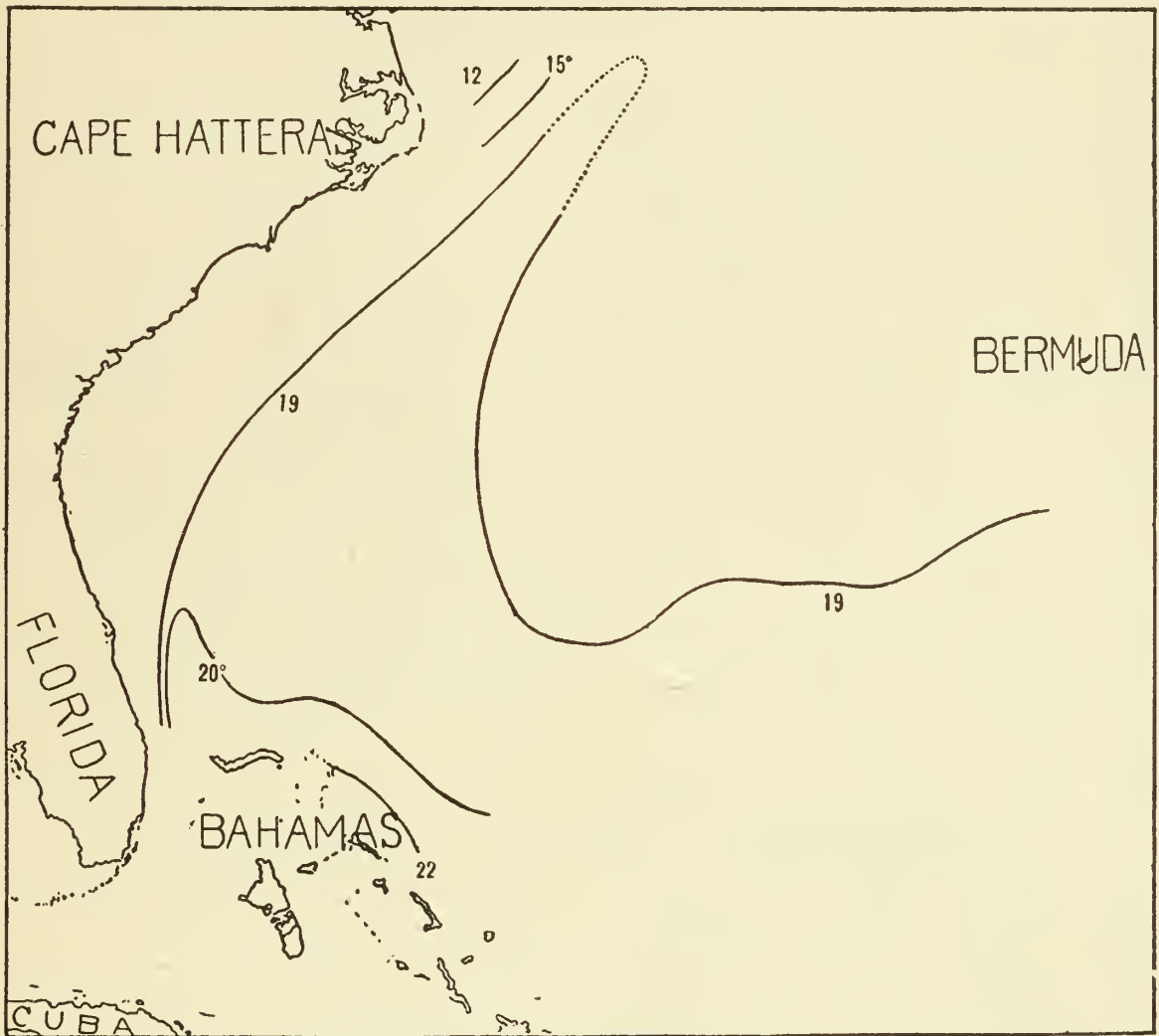
FIG. 17.—Temperatures at 200 meters.
