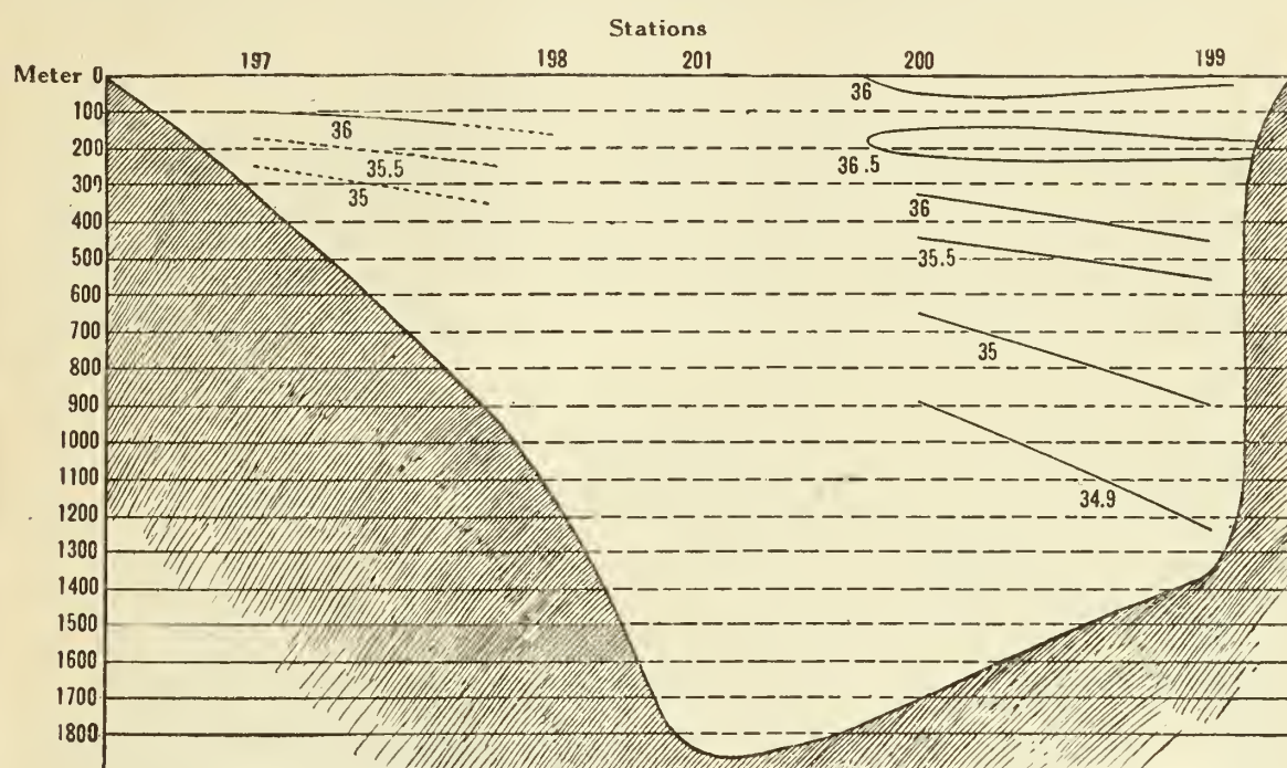
FIG. 25.—Salinity profile, Key West-Habana.
