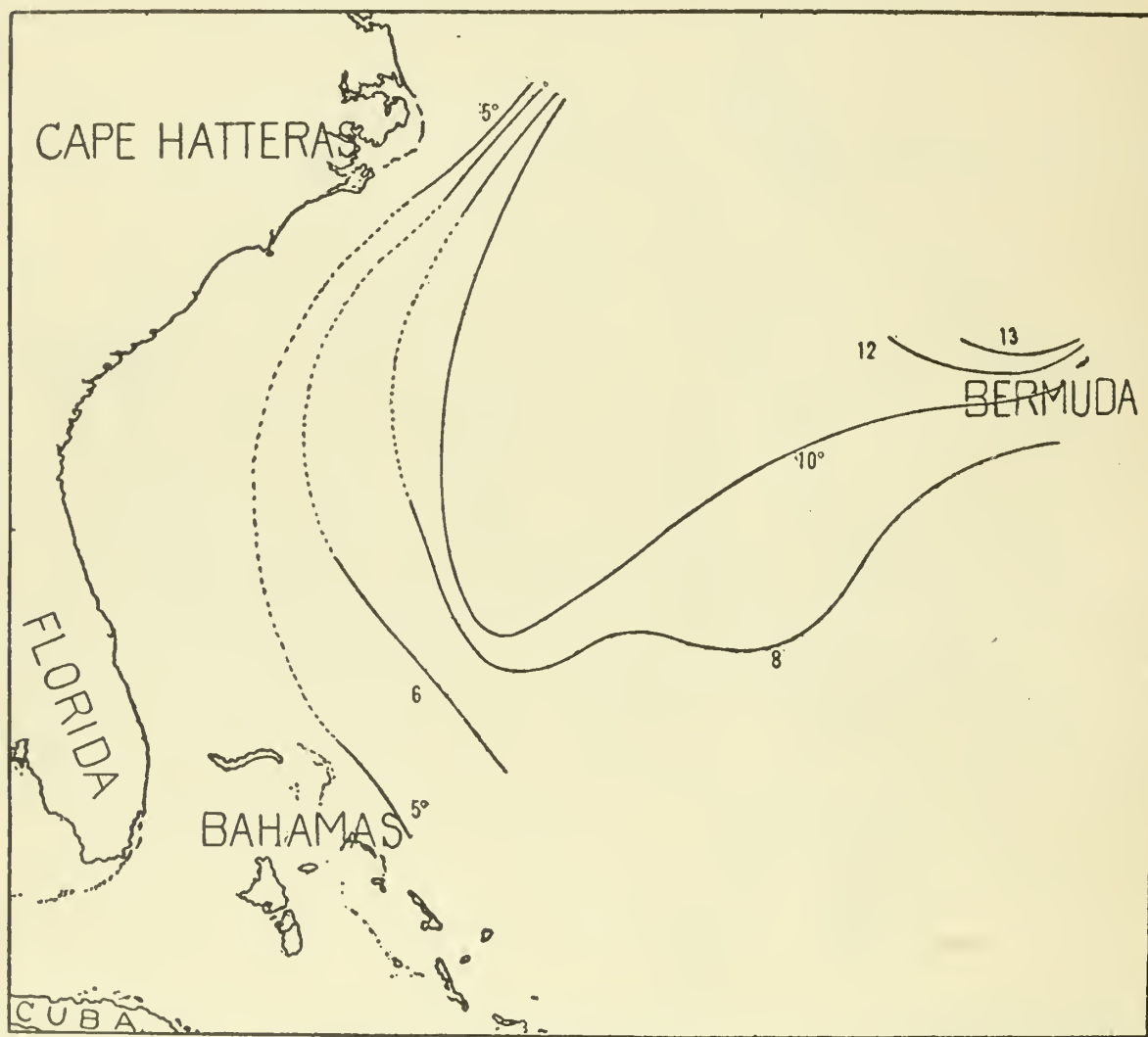
FIG. 20.—Temperature at 1,000 meters.
