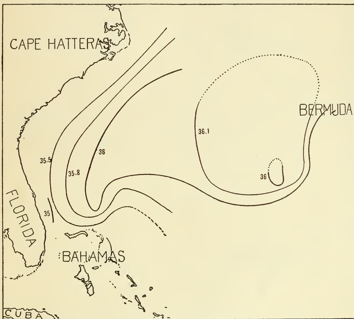
FIG. 19.—Salinity at 600 meters.
