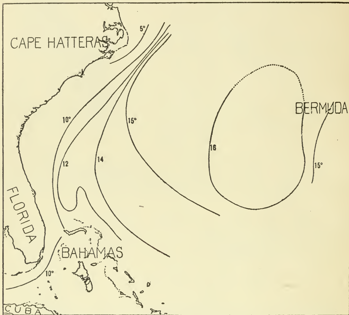
FIG. 18.—Temperatures at 600 meters.
