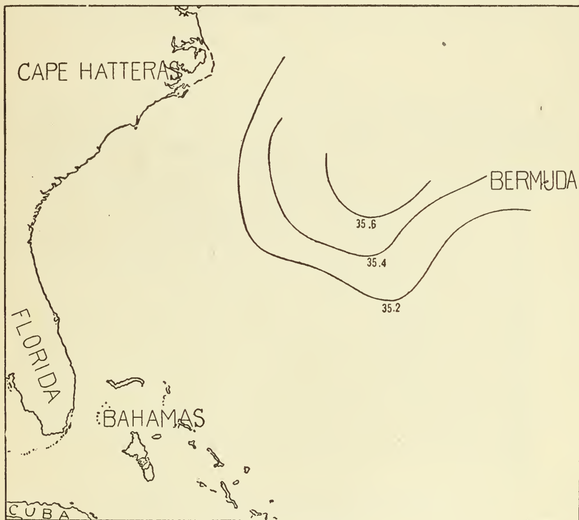
FIG. 21.—Salinity at 1,000 meters.
