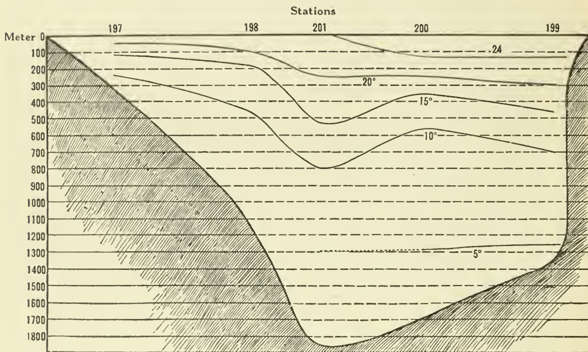
FIG. 24.—Temperature profile, Key West-Habana.
