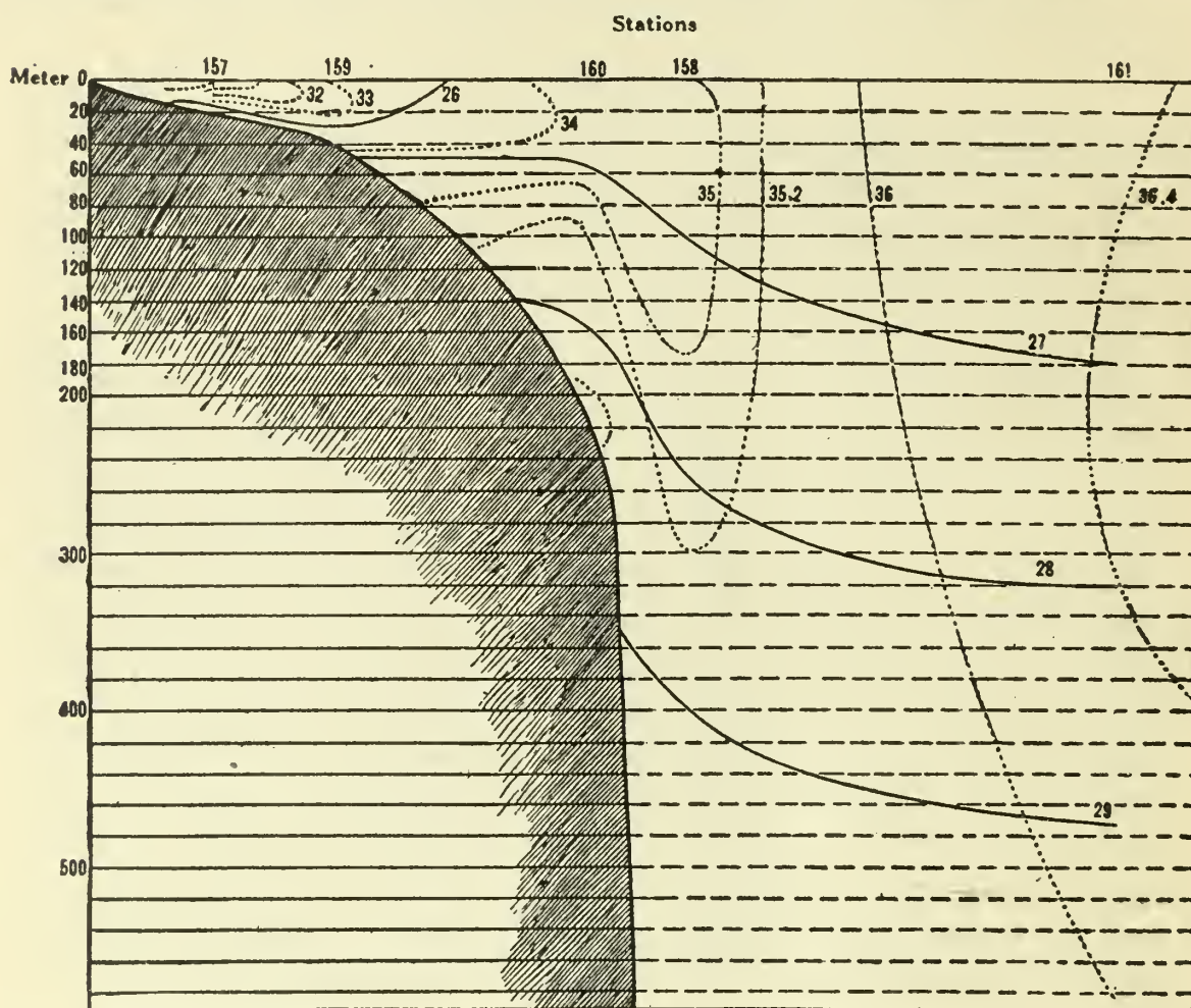
FIG. 49.—Profile of salinity, ....., and density at the temperature in situ , ———, from the mouth of Chesapeake Bay, across the continental shelf, to a point 90 miles southeast of the 200 meter contour.
