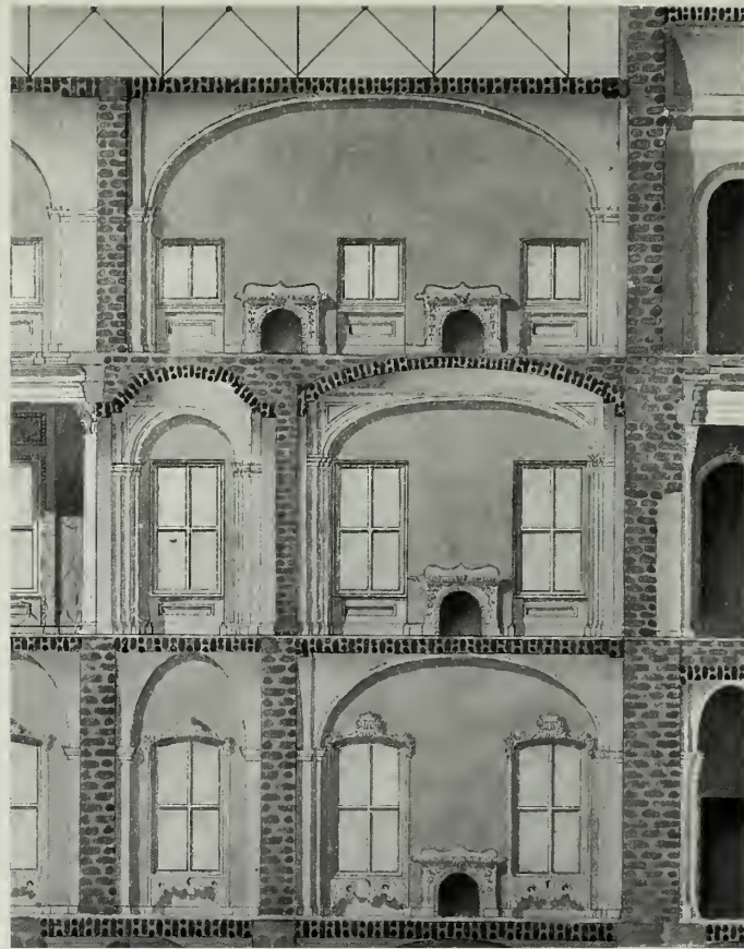
Figure 22. Original section drawing of the 2nd and 3rd floors of the House of Representatives Wing of the U.S. Capitol shows how Montgomery C. Meigs ensured the durability of the encaustic tile floors that were laid in the 1850s. He specified that the 3/4" tiles be laid on top of 1/2 to 3/4" mud (or mortar), which, in turn, was to be laid over a coal tar membrane on top of 3" of brick over an air space of 4-6". Photo: Wayne Firth, Office of the Architect of the Capitol.
